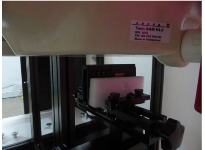
Photo 8: Top Side 15mm
