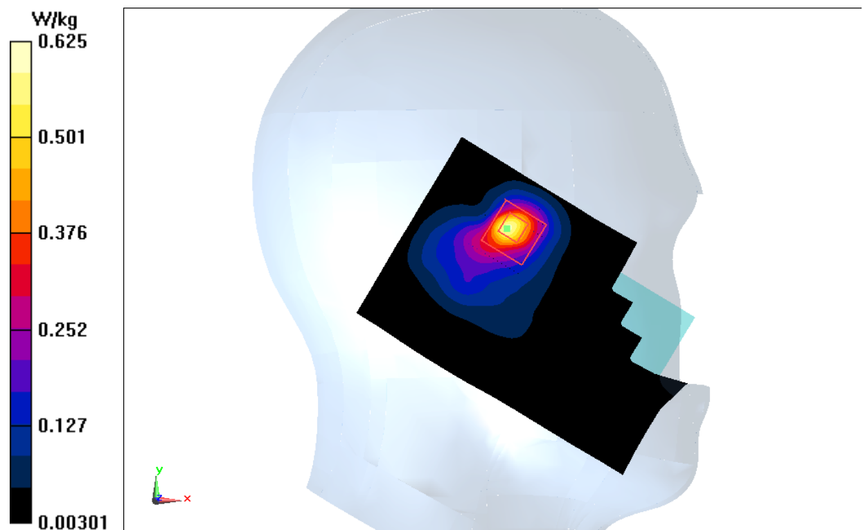
Fig.15 2450 MHz
