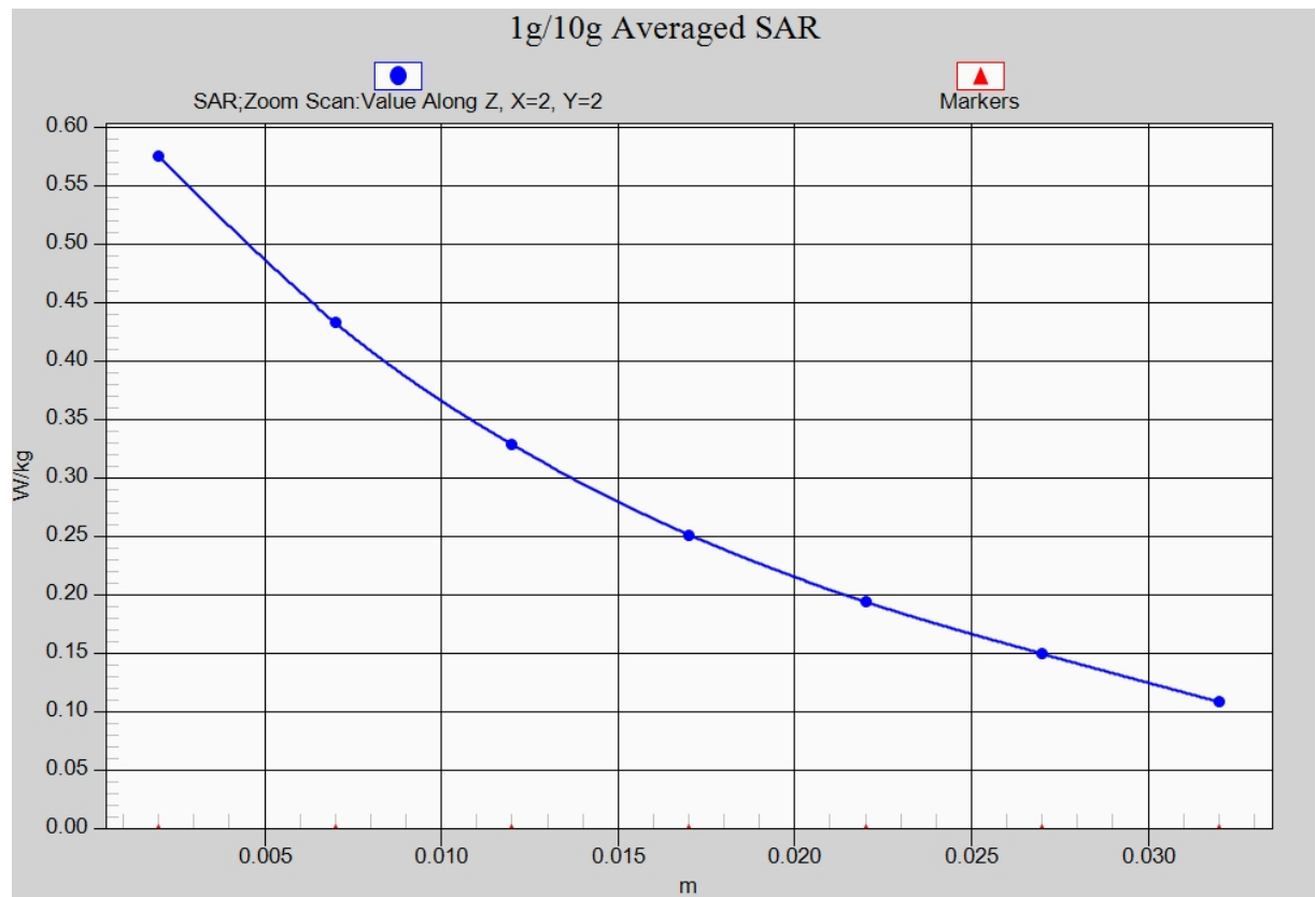
Fig. 14-1 Z-Scan at power reference point (LTE Band17)
