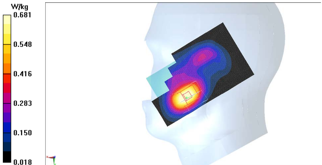
Fig.9 LTE Band4
