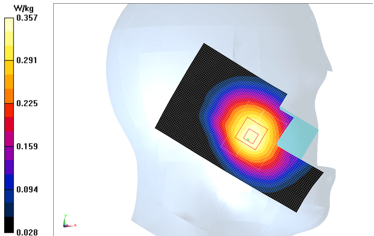
Fig.13 LTE Band17
