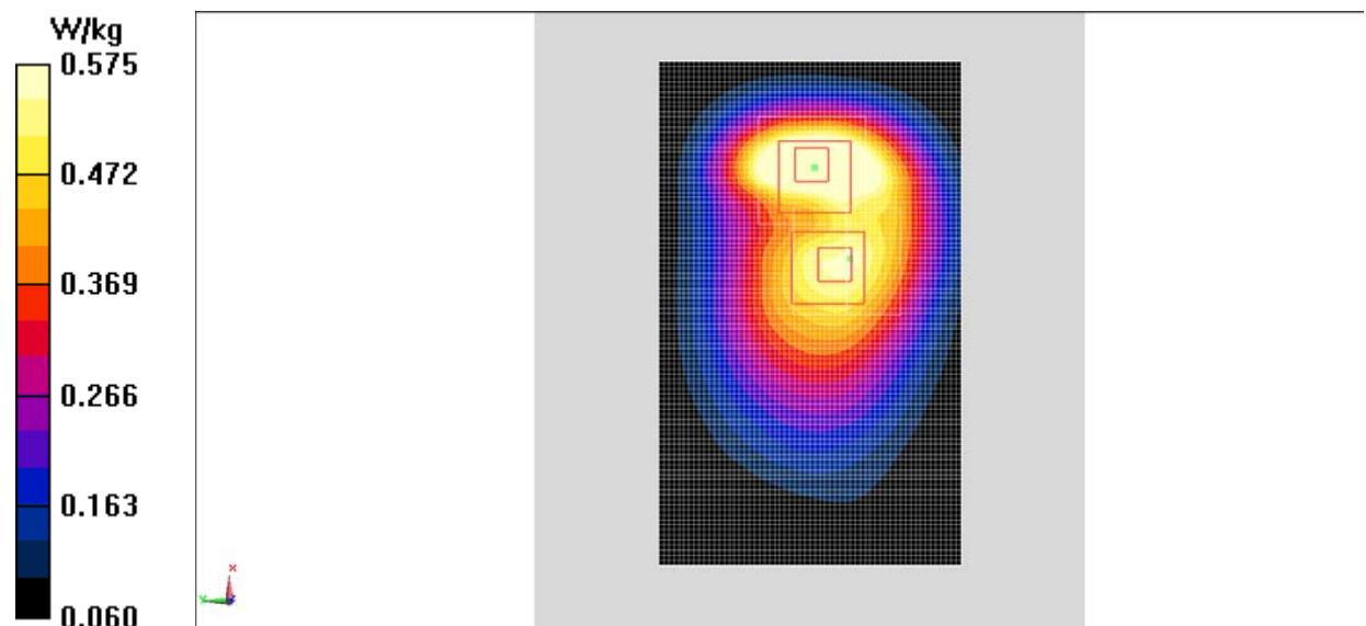
Fig.14 LTE Band17
