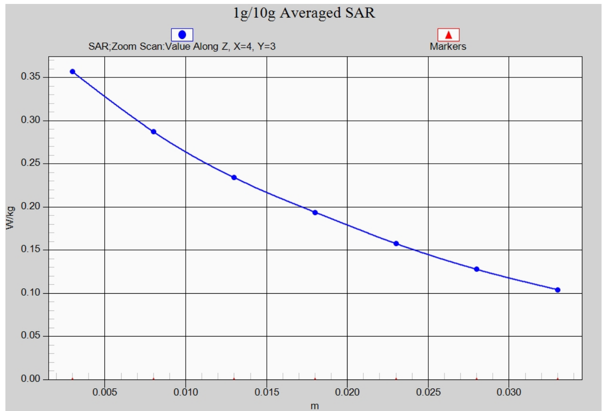
Fig. 13-1 Z-Scan at power reference point (LTE Band17)
