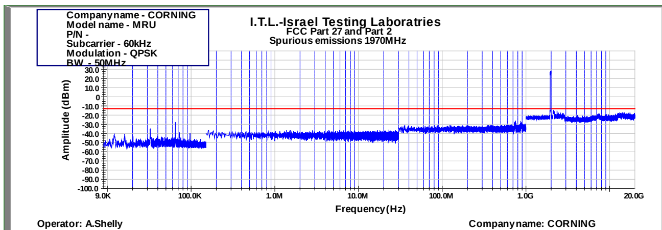
Figure 1058: Spurious Emissions at Antenna Terminal QPSK 50MHz B.W.; 1970.0MHz, 60kHz
