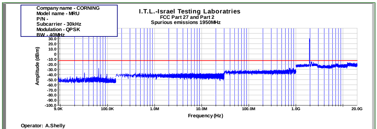
Figure 1042: Spurious Emissions at Antenna Terminal QPSK 40MHz B.W.; 1950.0MHz, 30kHz
