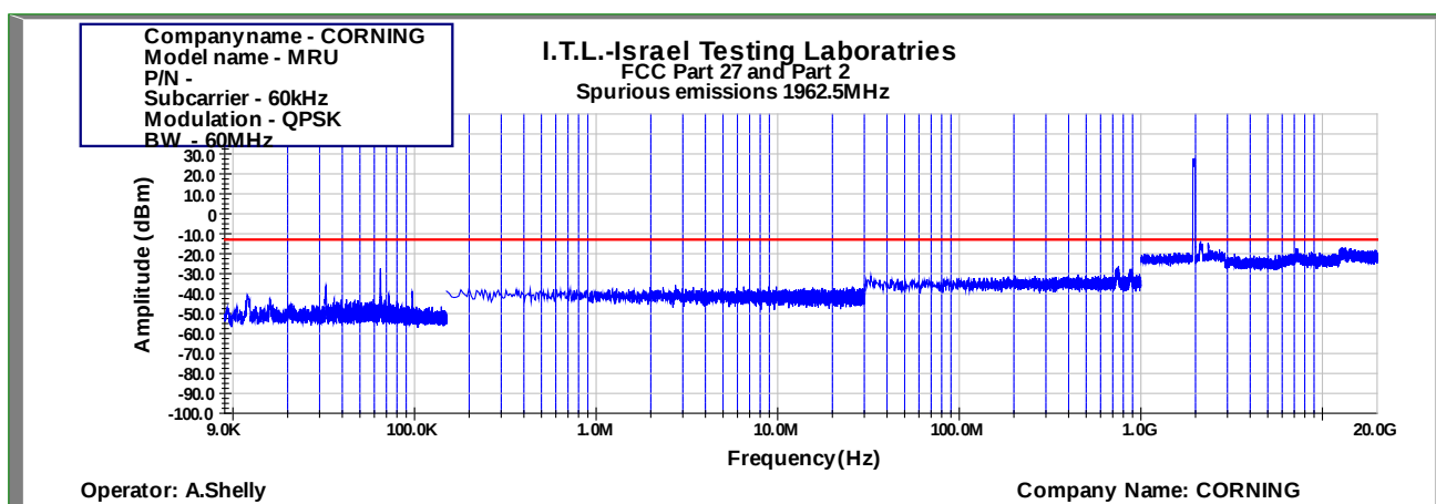
Figure 1062: Spurious Emissions at Antenna Terminal QPSK 60MHz B.W.; 1962.5MHz, 60kHz
