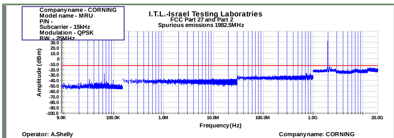
Figure 1038: Spurious Emissions at Antenna Terminal QPSK 25MHz B.W.; 1982.5MHz, 15kHz
