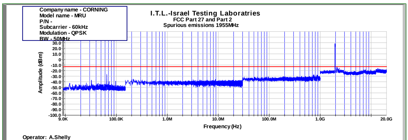
Figure 1052: Spurious Emissions at Antenna Terminal QPSK 50MHz B.W.; 1955.0MHz, 60kHz
