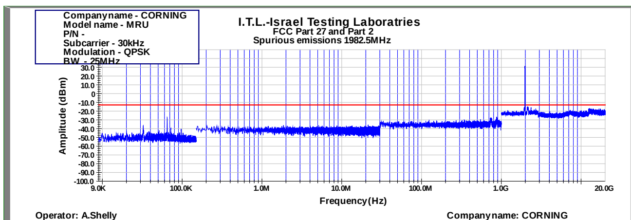
Figure 1039: Spurious Emissions at Antenna Terminal QPSK 25MHz B.W.; 1982.5MHz, 30kHz
