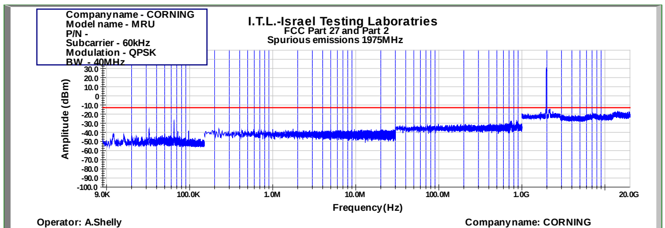
Figure 1049: Spurious Emissions at Antenna Terminal QPSK 40MHz B.W.; 1975.0MHz, 60kHz
