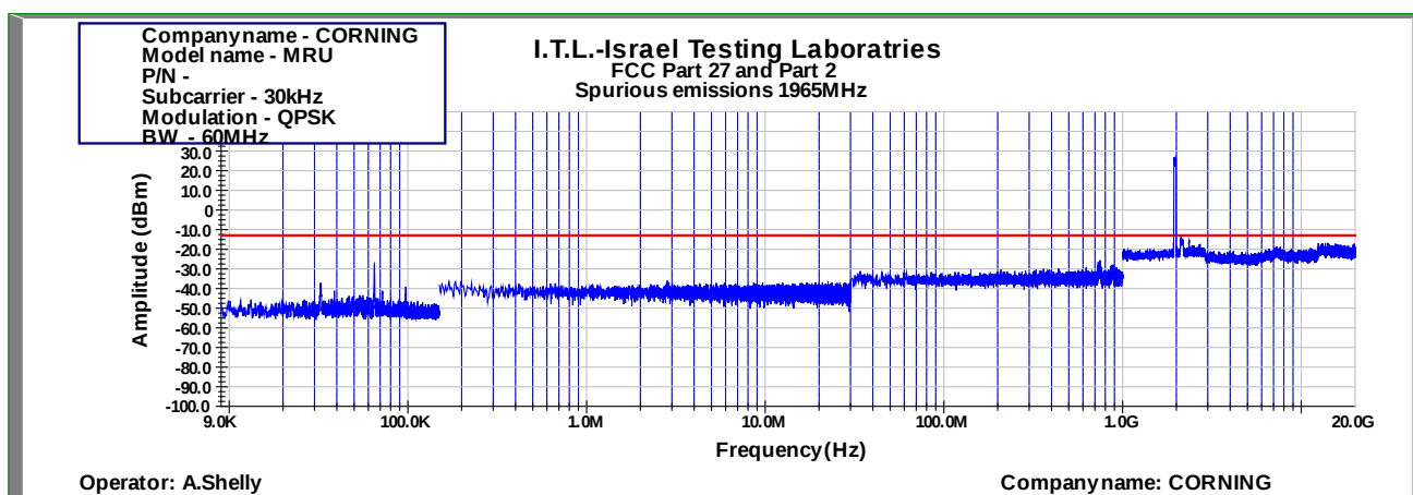
Figure 1063: Spurious Emissions at Antenna Terminal QPSK 60MHz B.W.; 1965.0MHz, 30kHz
