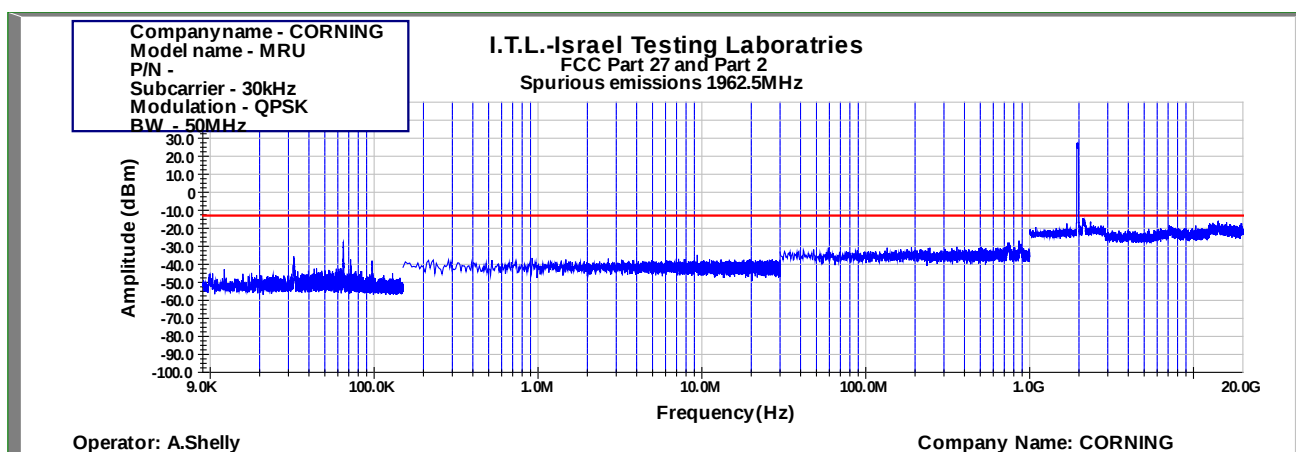
Figure 1054: Spurious Emissions at Antenna Terminal QPSK 50MHz B.W.; 1962.5MHz, 30kHz
