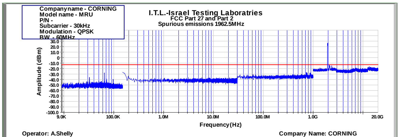
Figure 1061: Spurious Emissions at Antenna Terminal QPSK 60MHz B.W.; 1962.5MHz, 30kHz
