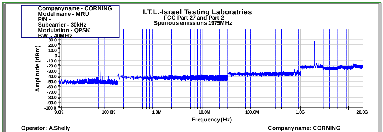
Figure 1048: Spurious Emissions at Antenna Terminal QPSK 40MHz B.W.; 1975.0MHz, 30kHz
