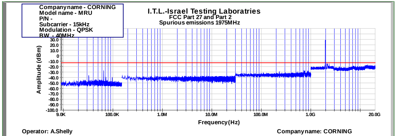
Figure 1047: Spurious Emissions at Antenna Terminal QPSK 40MHz B.W.; 1975.0MHz, 15kHz
