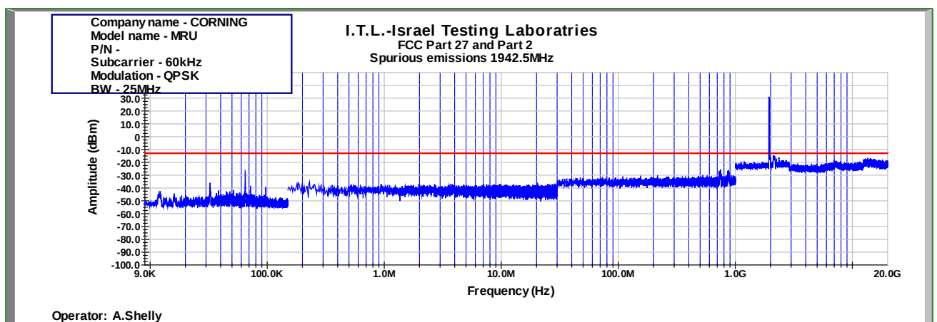
Figure 1034: Spurious Emissions at Antenna Terminal QPSK 25MHz B.W.; 1942.5MHz, 60kHz
