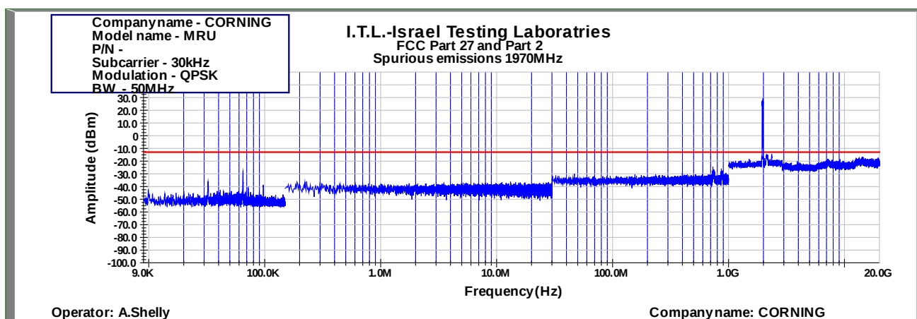
Figure 1057: Spurious Emissions at Antenna Terminal QPSK 50MHz B.W.; 1970.0MHz, 30kHz
