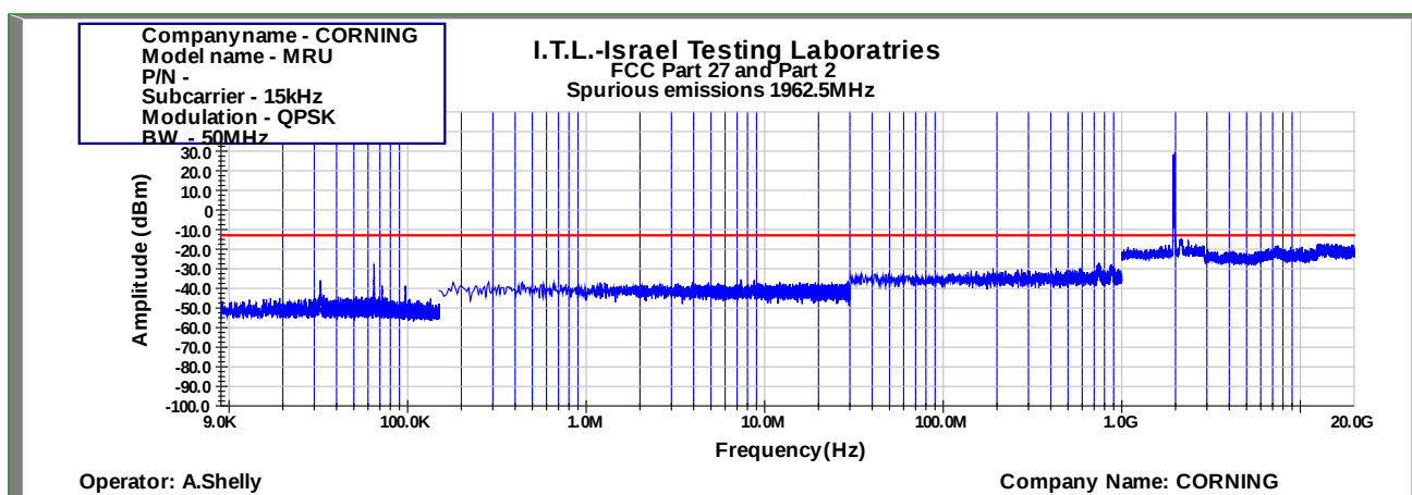
Figure 1053: Spurious Emissions at Antenna Terminal QPSK 50MHz B.W.; 1962.5MHz, 15kHz
