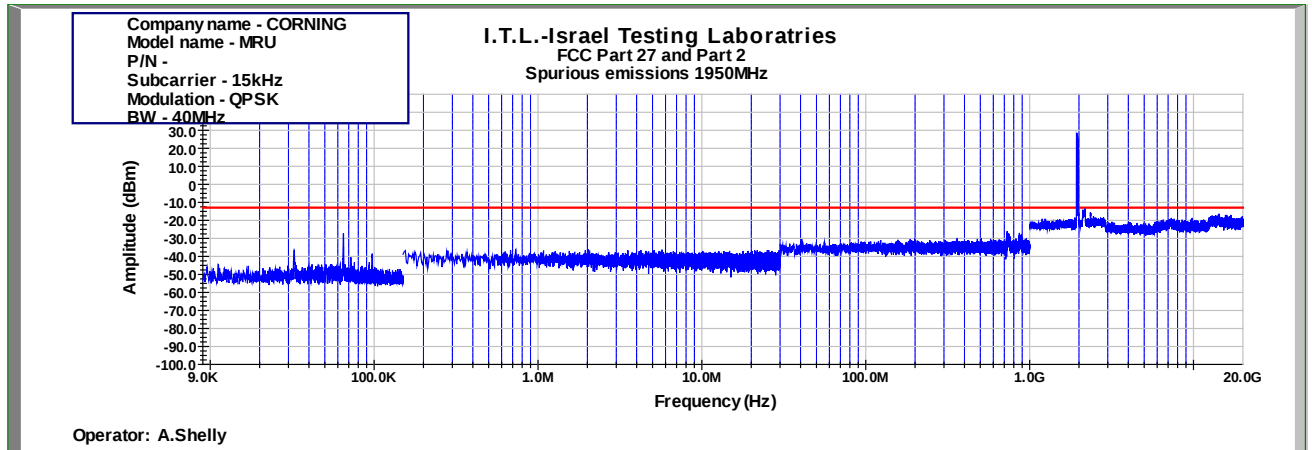
Figure 1041: Spurious Emissions at Antenna Terminal QPSK 40MHz B.W.; 1950.0MHz, 15kHz
