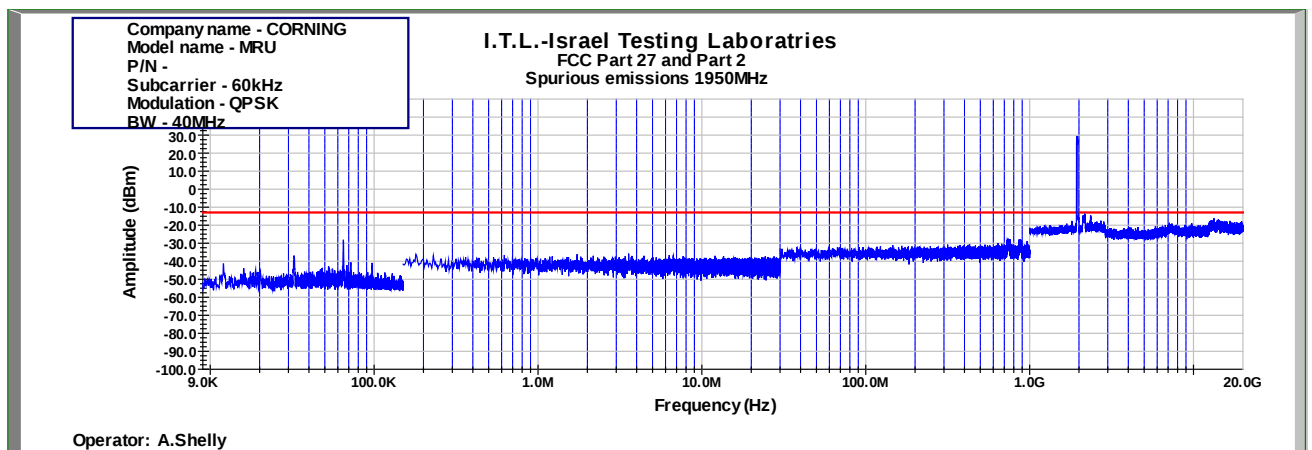
Figure 1043: Spurious Emissions at Antenna Terminal QPSK 40MHz B.W.; 1950.0MHz, 60kHz
