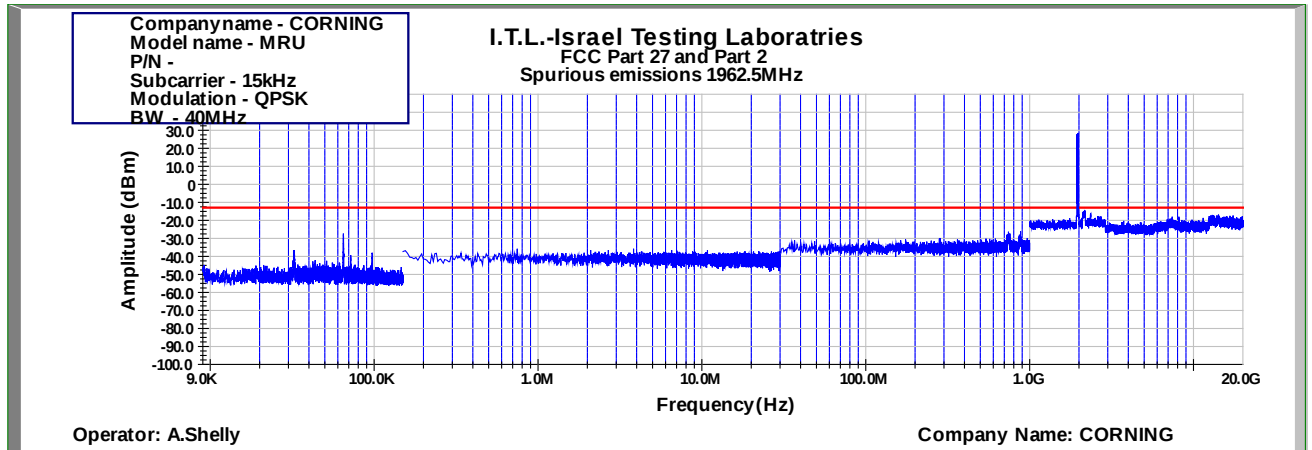
Figure 1044: Spurious Emissions at Antenna Terminal QPSK 40MHz B.W.; 1962.5MHz, 15kHz
