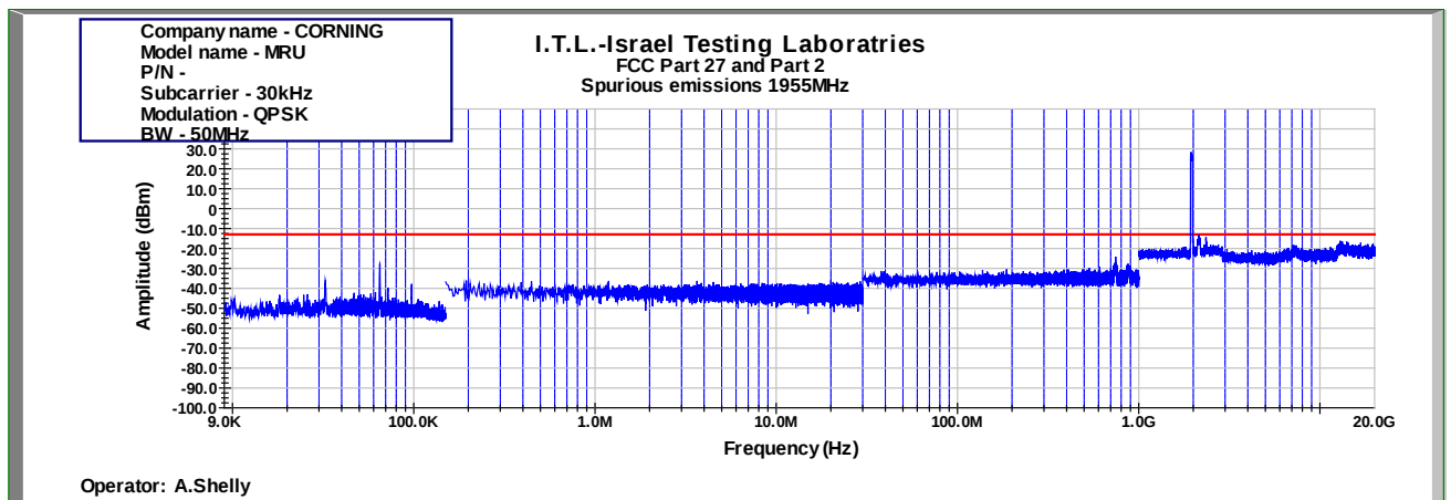
Figure 1051: Spurious Emissions at Antenna Terminal QPSK 50MHz B.W.; 1955.0MHz, 30kHz
