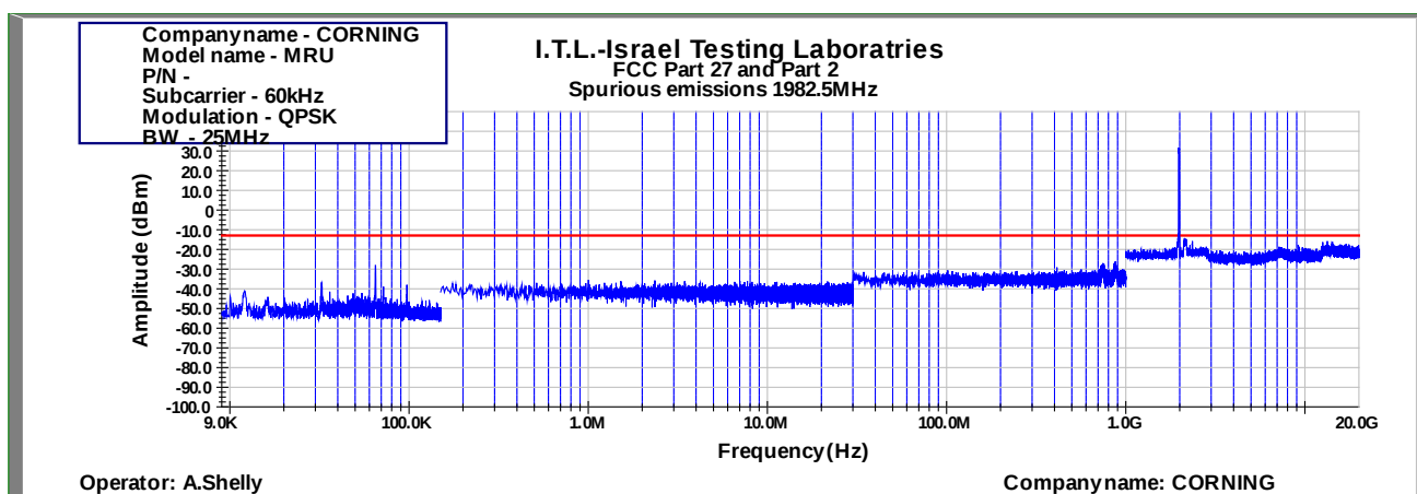
Figure 1040: Spurious Emissions at Antenna Terminal QPSK 25MHz B.W.; 1982.5MHz, 60kHz
