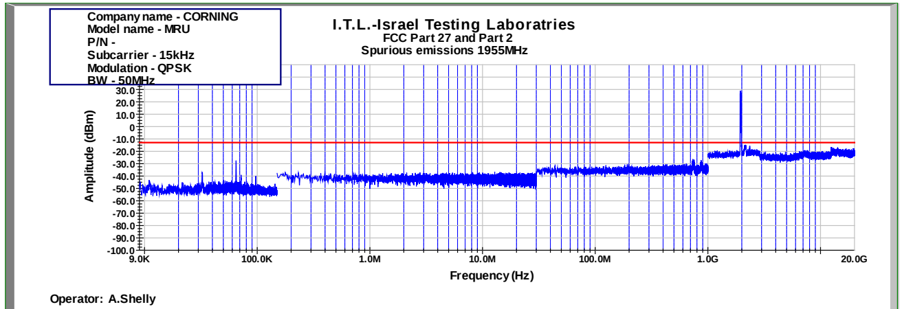
Figure 1050: Spurious Emissions at Antenna Terminal QPSK 50MHz B.W.; 1955.0MHz, 15kHz
