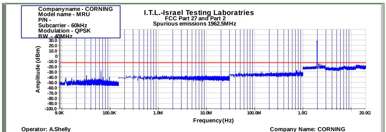
Figure 1046: Spurious Emissions at Antenna Terminal QPSK 40MHz B.W.; 1962.5MHz, 60kHz
