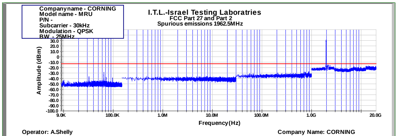
Figure 1036: Spurious Emissions at Antenna Terminal QPSK 25MHz B.W.; 1962.5MHz, 30kHz
