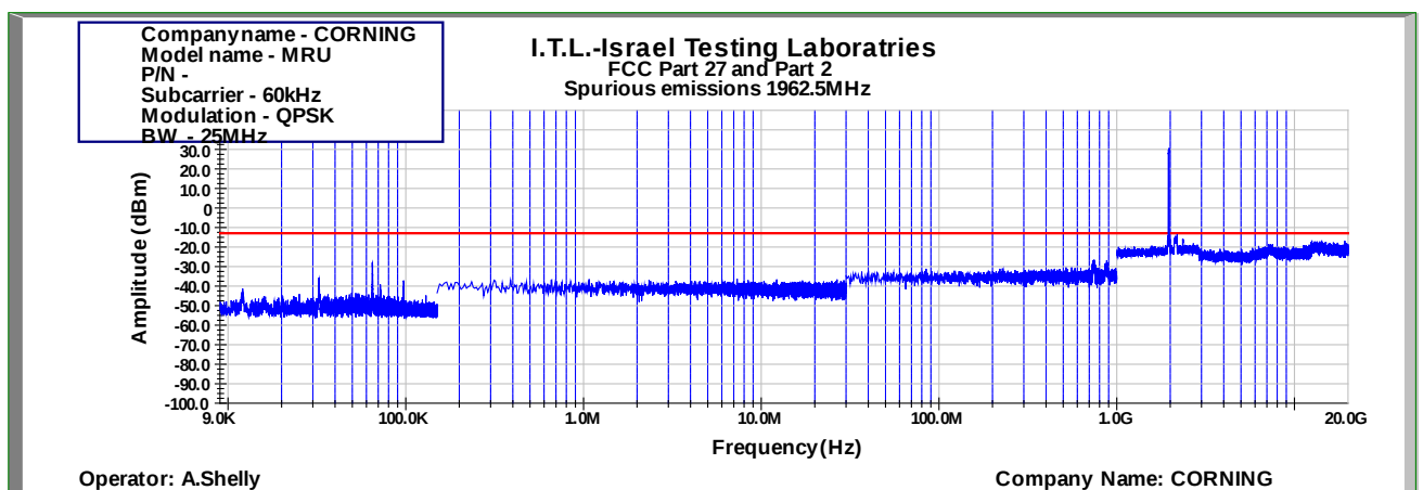
Figure 1037: Spurious Emissions at Antenna Terminal QPSK 25MHz B.W.; 1962.5MHz, 60kHz
