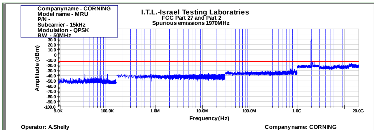
Figure 1056: Spurious Emissions at Antenna Terminal QPSK 50MHz B.W.; 1970.0MHz, 15kHz
