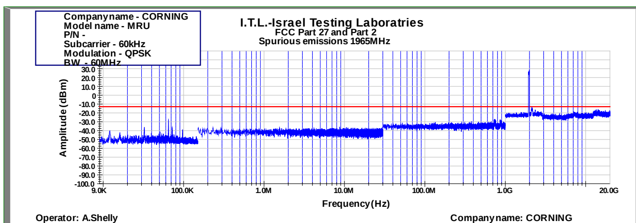
Figure 1064: Spurious Emissions at Antenna Terminal QPSK 60MHz B.W.; 1965.0MHz, 60kHz
