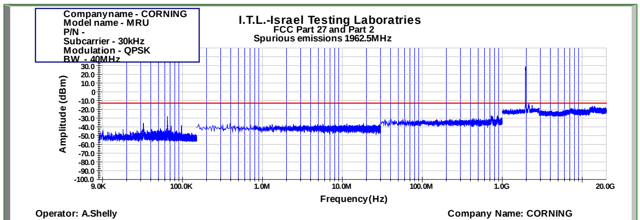
Figure 1045: Spurious Emissions at Antenna Terminal QPSK 40MHz B.W.; 1962.5MHz, 30kHz
