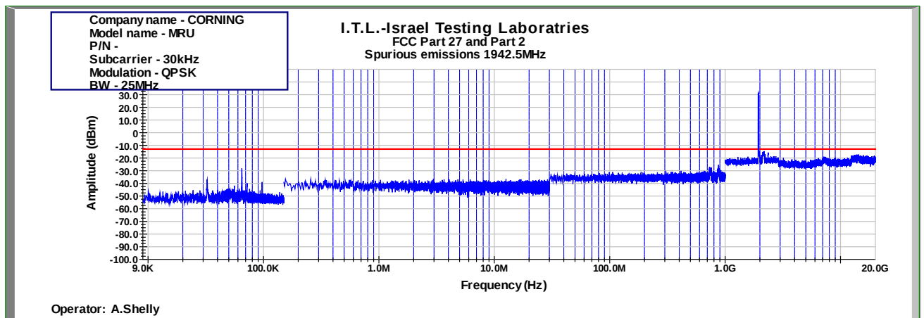
Figure 1033: Spurious Emissions at Antenna Terminal QPSK 25MHz B.W.; 1942.5MHz, 30kHz
