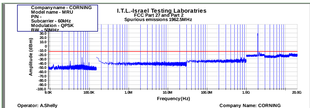
Figure 1055: Spurious Emissions at Antenna Terminal QPSK 50MHz B.W.; 1962.5MHz, 60kHz
