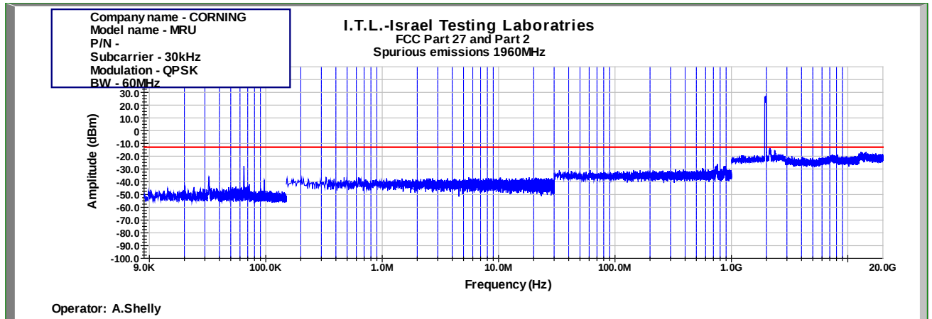
Figure 1059: Spurious Emissions at Antenna Terminal QPSK 60MHz B.W.; 1960.0MHz, 30kHz
