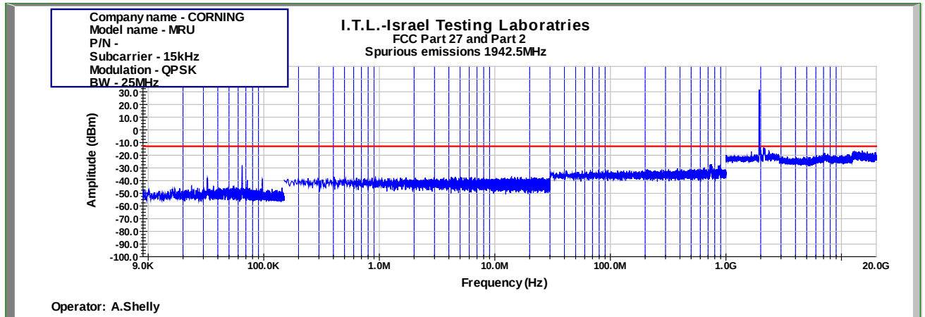
Figure 1032: Spurious Emissions at Antenna Terminal QPSK 25MHz B.W.; 1942.5MHz, 15kHz
