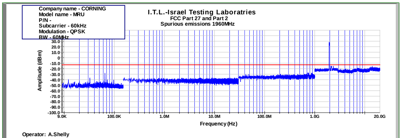
Figure 1060: Spurious Emissions at Antenna Terminal QPSK 60MHz B.W.; 1960.0MHz, 60kHz
