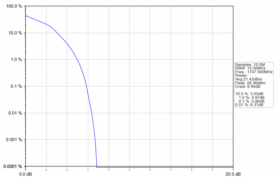
Band4 15MHz 16QAM HCH 1747.5MHz RB 75 0 NTNV
