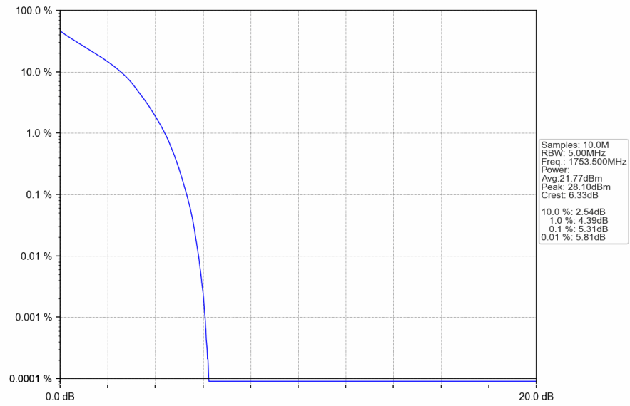
Band4 3MHz QPSK HCH 1753.5MHz RB 15 0 NTNV
