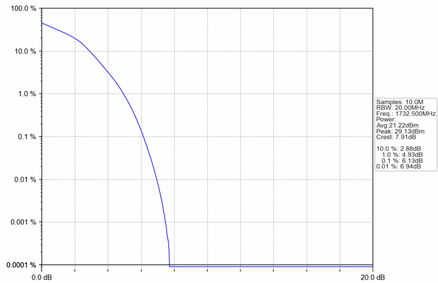
Band4 20MHz 16QAM MCH 1732.5MHz RB 100 0 NTNV
