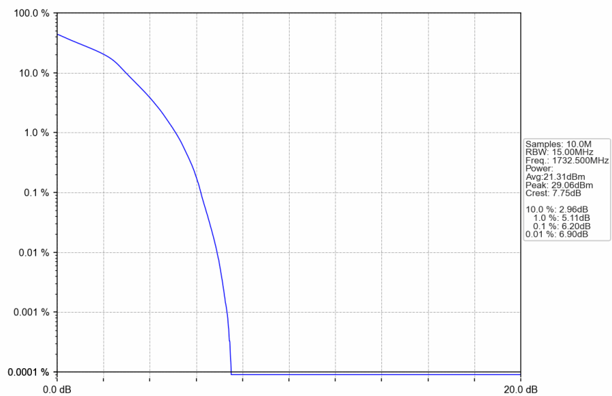
Band4 15MHz 16QAM MCH 1732.5MHz RB 75 0 NTNV
