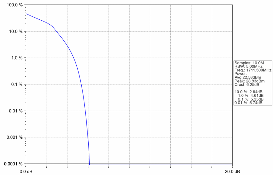
Band4 3MHz 16QAM LCH 1711.5MHz RB 15 0 NTNV
