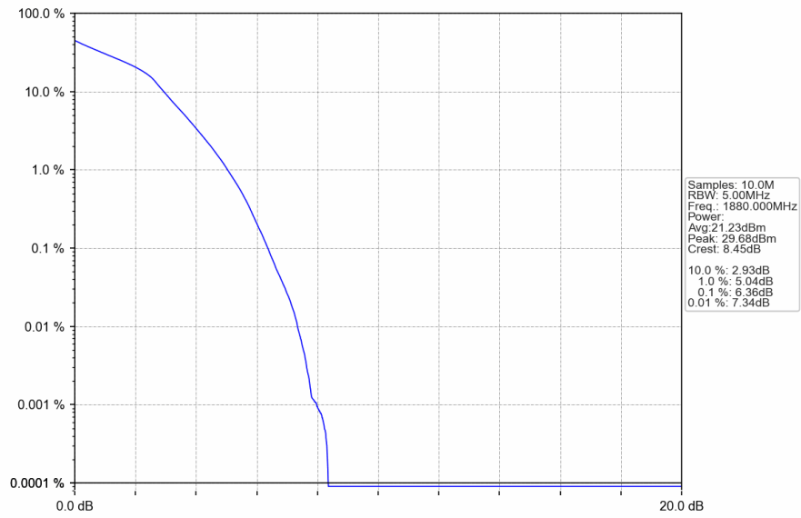
Band2 3MHz 16QAM MCH 1880MHz RB 15 0 NTNV
