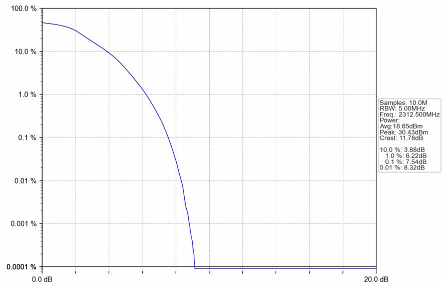
Band40a 5MHz QPSK HCH 2312.5MHz RB 25 0 NTN
