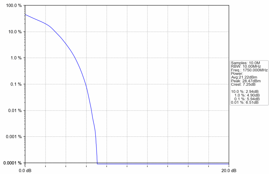
Band4 10MHz 16QAM HCH 1750MHz RB 50 0 NTNV
