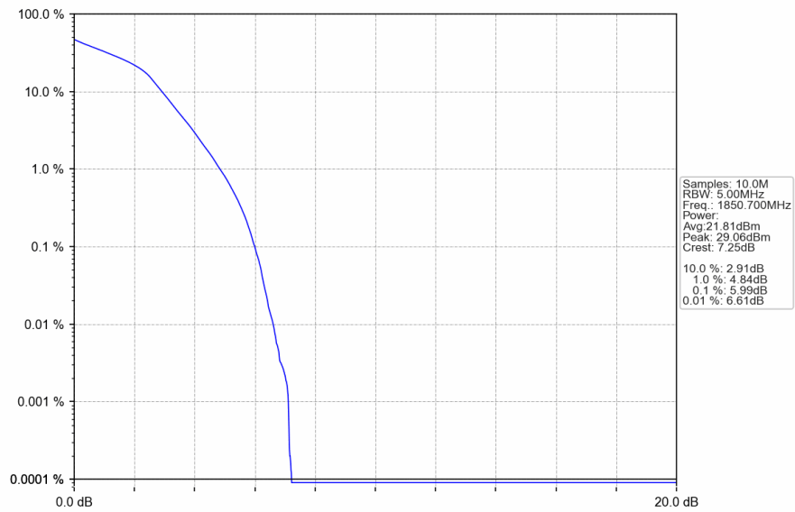
Band2 1.4MHz 16QAM LCH 1850.7MHz RB 6 0 NTNV
