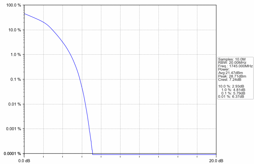
Band4 20MHz 16QAM HCH 1745MHz RB 100 0 NTNV
