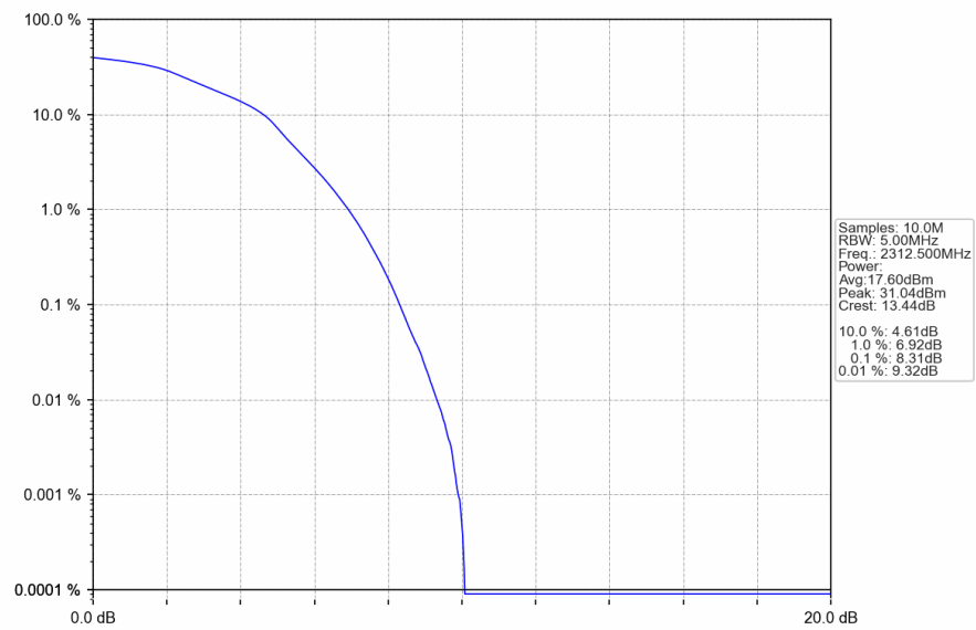
Band40a 5MHz 16QAM HCH 2312.5MHz RB 25 0 NTN
