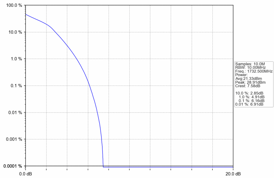
Band4 10MHz 16QAM MCH 1732.5MHz RB 50 0 NTNV
