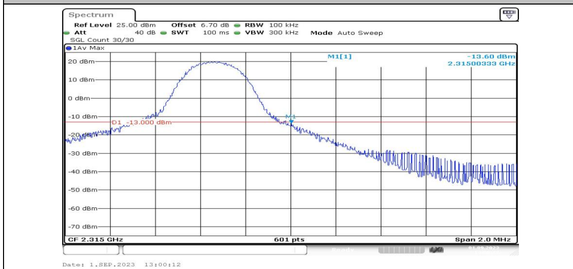
Band40-5MHz-16QAM-38775-1RB#24-PASS
