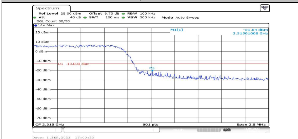
Band40-5MHz-QPSK-38775-25RB#0-PASS
