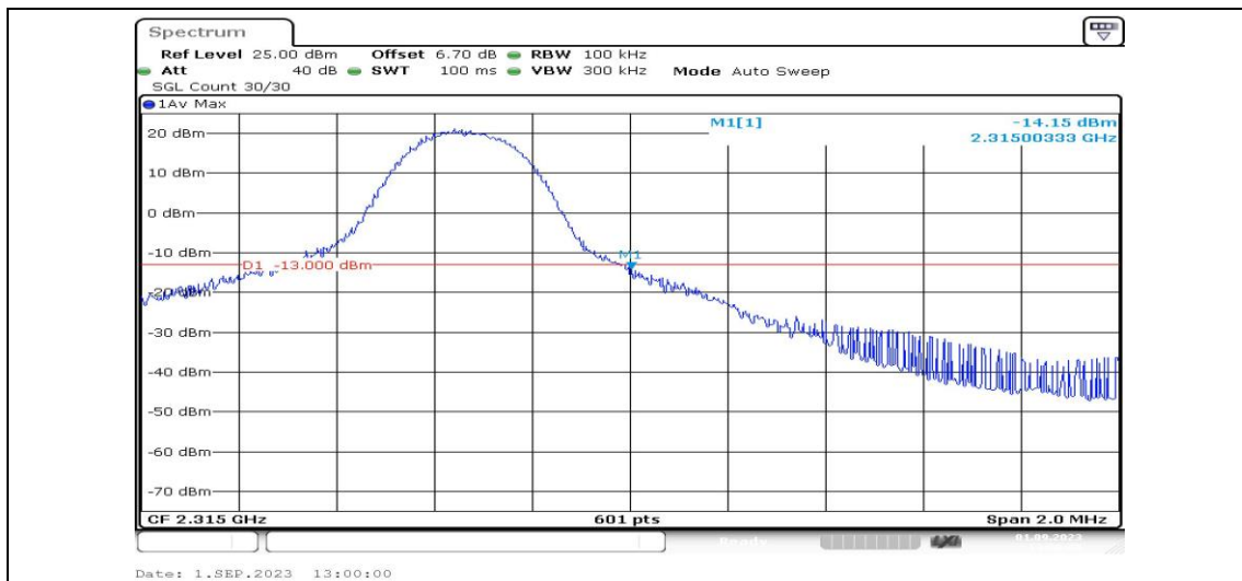
Band40-5MHz-QPSK-38775-1RB#24-PASS
