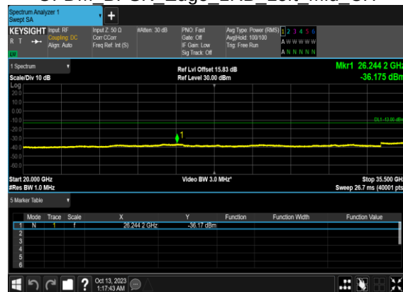
N78(10M)_DFT-s-OFDM BPSK Edge 1RB Left Mid CH
