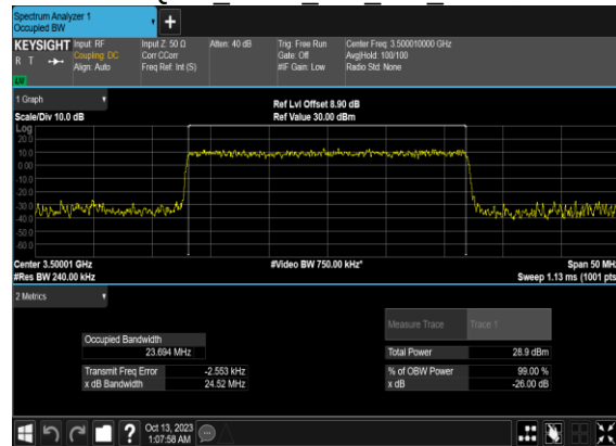
N78(25M)_CP-OFDM_16 QAM Outer Full Mid CH
