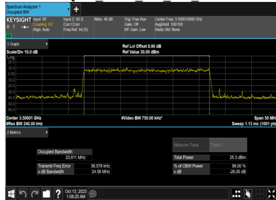
N78(25M)_CP-OFDM_256 QAM Outer Full Mid CH
