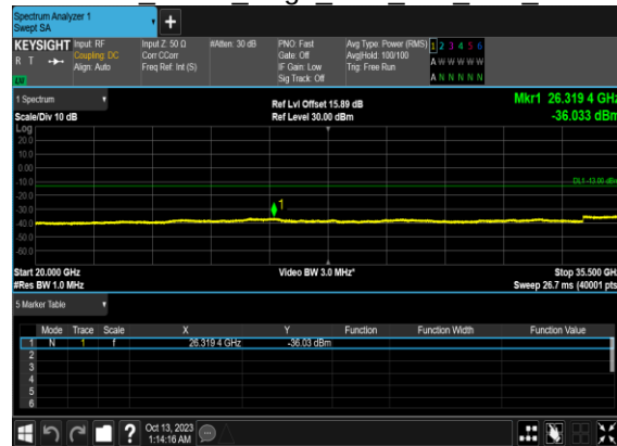
N78(10M)_DFT-s-OFDM BPSK Edge 1RB Left Low CH
