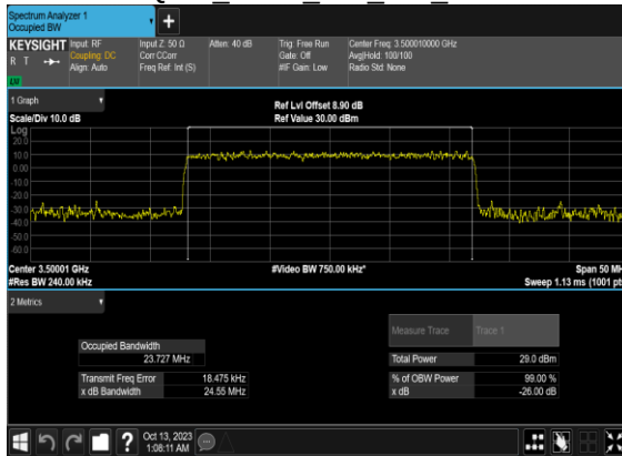
N78(25M)_CP-OFDM_64 QAM Outer Full Mid CH
