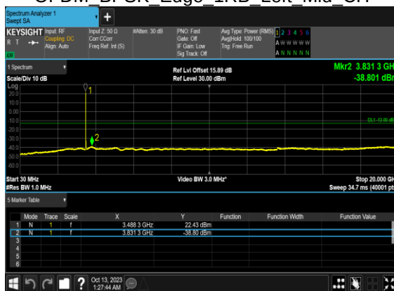
N78(25M)_DFT-s- OFDM BPSK Edge 1RB Left Mid CH
