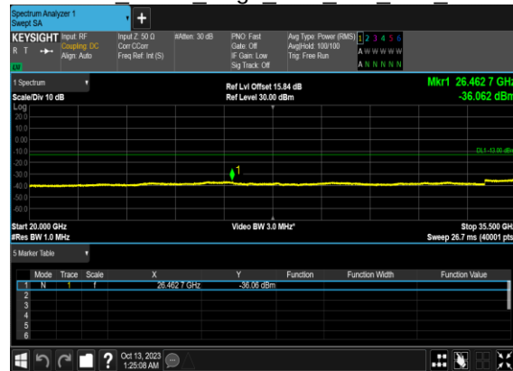
N78(25M)_DFT-s- OFDM BPSK Edge 1RB Left Low CH
