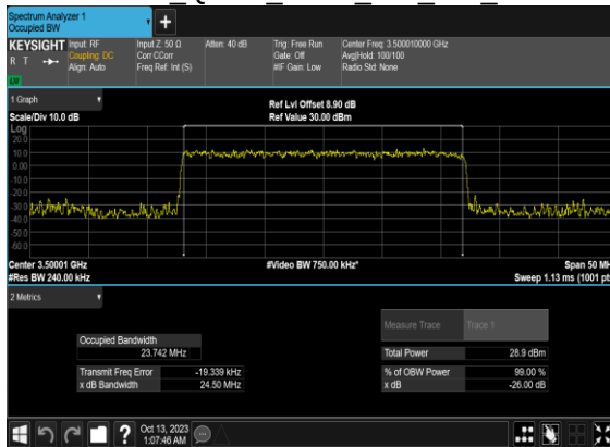
N78(25M)_CP- OFDM QPSK Outer Full Mid CH
