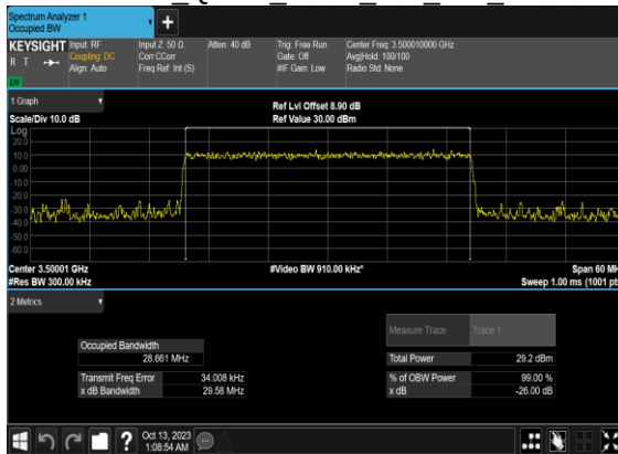
N78(30M)_CP- OFDM QPSK Outer Full Mid CH
