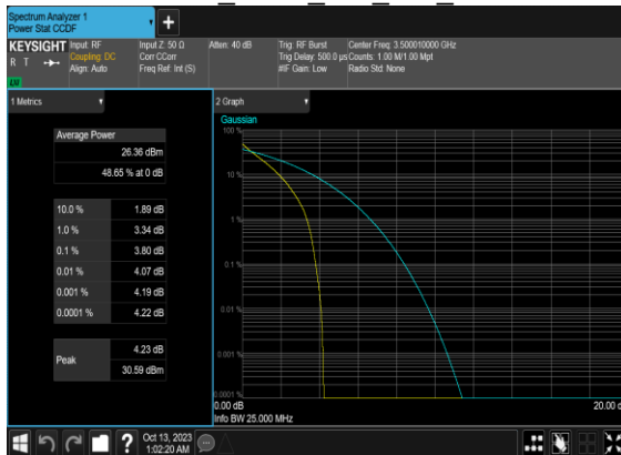
N78(20M)_DFT-s-OFDM_PI_2-BPSK Outer Full Mid CH
