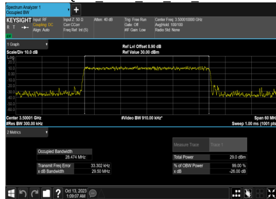
N78(30M)_CP-OFDM_16 QAM Outer Full Mid CH
