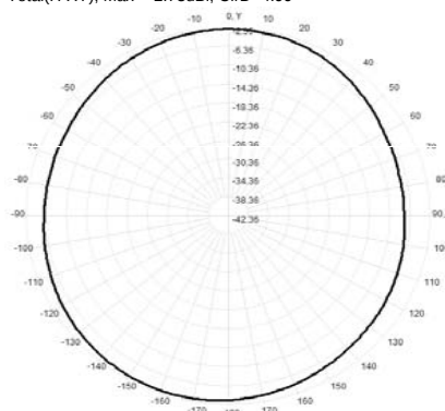
Total(H-XY), Max= -2.73dBi, CirD=4.99
