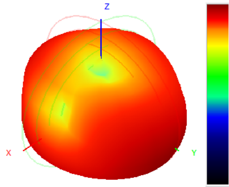
916.0MHz H+V, Eff: 21.4%
