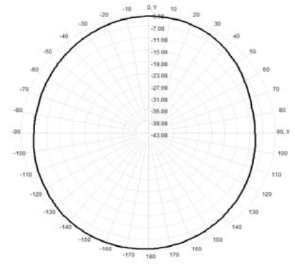
Total(H-XY), Max= -3.81dBi, CirD=6.07
