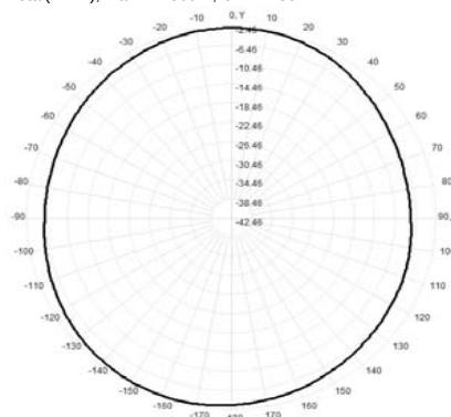
Total(H-XY), Max= -2.80dBi, CirD=4.80
