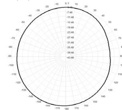
Total(H-XY), Max= -4.12dBi, CirD=6.55
