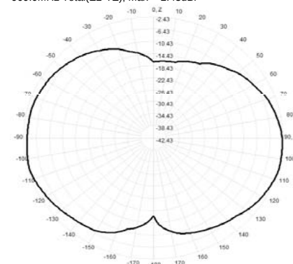
909.0MHz Total(E2-YZ), Max= -2.43dBi
