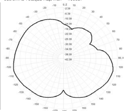
910.0MHz Total(E1-XZ), Max= -4.60dBi
