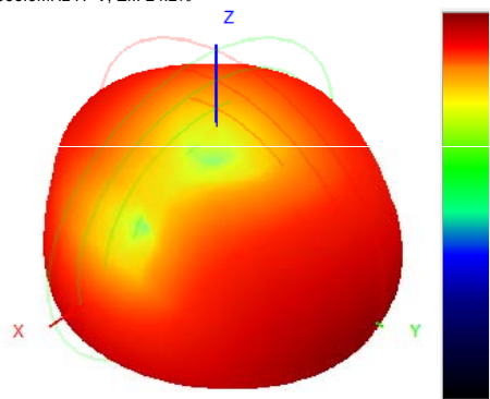
906.0MHz H+V, Eff: 24.2%
