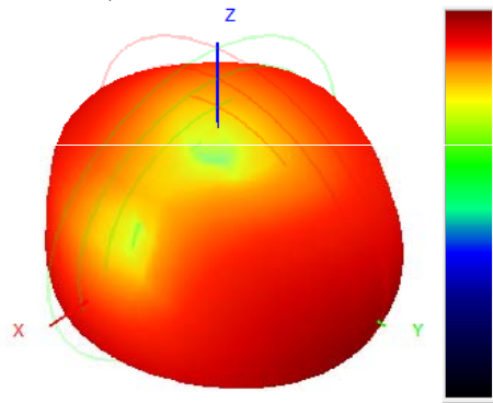
915.0MHz H+V, Eff: 21.8%
