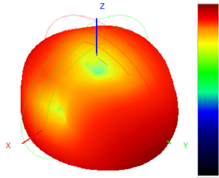
925.0MHz H+V, Eff: 18.4%
