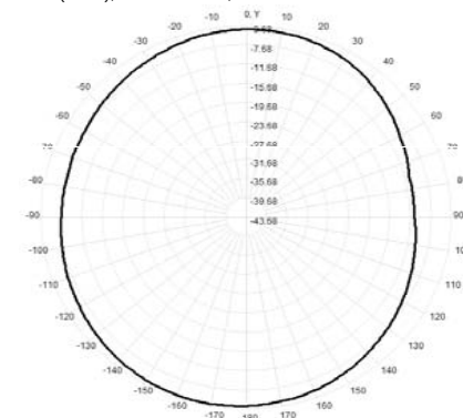
Total(H-XY), Max= -4.31dBi, CirD=6.75
