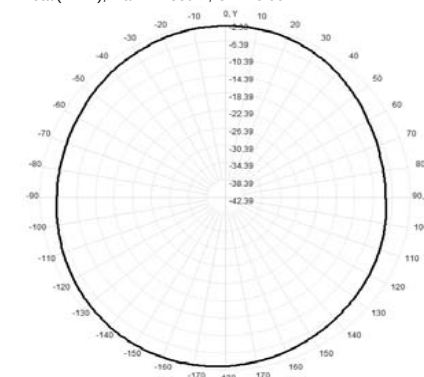
Total(H-XY), Max= -2.85dBi, CirD=5.06
