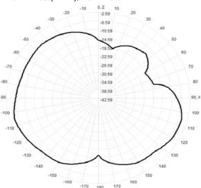
914.0MHz Total(E1-XZ), Max= -4.89dBi
