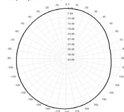
Total(H-XY), Max= -4.23dBi, CirD=6.60
