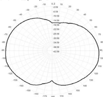
914.0MHz Total(E2-YZ), Max= -2.59dBi
