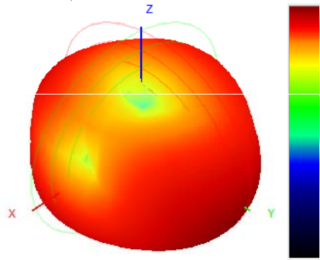
924.0MHz H+V, Eff: 18.7%
