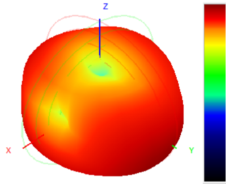
928.0MHz H+V, Eff: 17.3%
