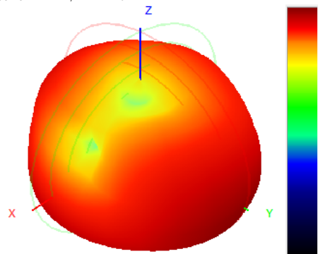
904.0MHz H+V, Eff: 24.4%
