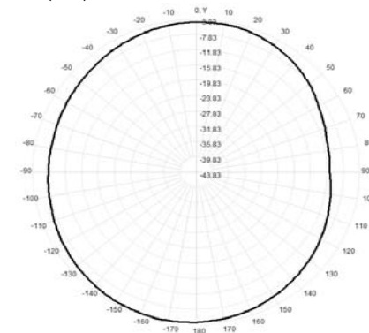
Total(H-XY), Max= -4.40dBi, CirD=6.95
