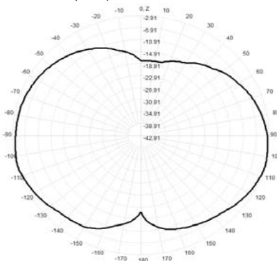
919.0MHz Total(E2-YZ), Max= -2.91dBi
