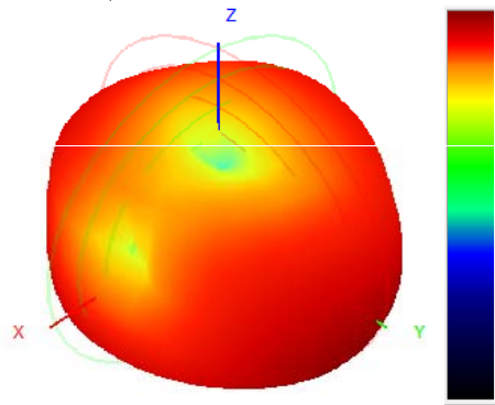
927.0MHz H+V, Eff: 17.7%
