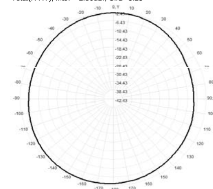
Total(H-XY), Max= -2.80dBi, CirD=5.25
