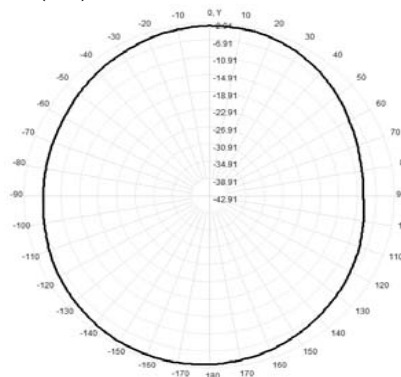
Total(H-XY), Max= -3.63dBi, CirD=6.22
