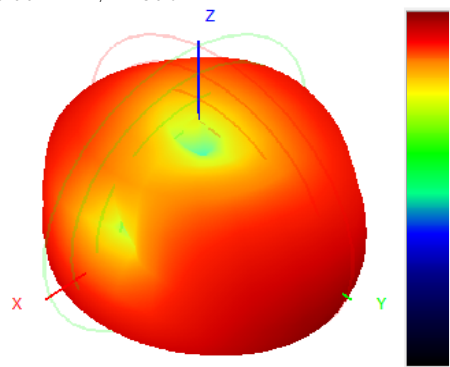
926.0MHz H+V, Eff: 18.0%
