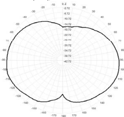
915.0MHz Total(E2-YZ), Max= -2.72dBi
