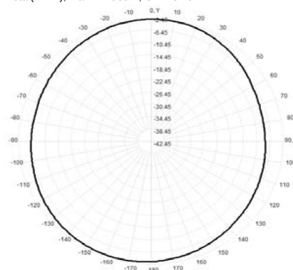
Total(H-XY), Max= -2.93dBi, CirD=5.19
