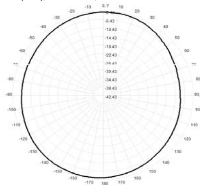
Total(H-XY), Max= -3.06dBi, CirD=5.44
