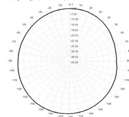
Total(H-XY), Max= -3.94dBi, CirD=6.57
