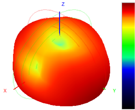
919.0MHz H+V, Eff: 20.3%
