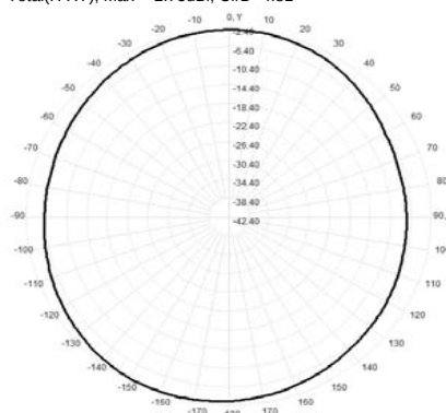
Total(H-XY), Max= -2.75dBi, CirD=4.81
