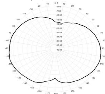
927.0MHz Total(E2-YZ), Max= -3.68dBi
