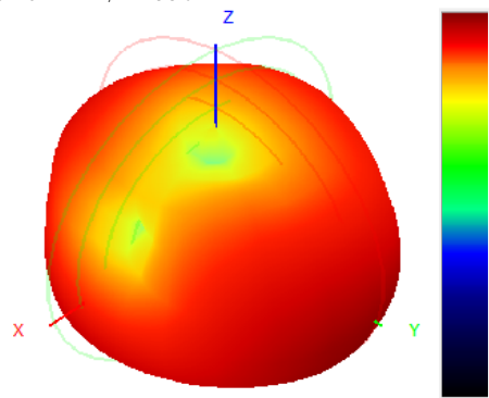
911.0MHz H+V, Eff: 23.3%
