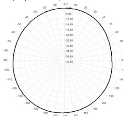
Total(H-XY), Max= -3.51dBi, CirD=6.02
