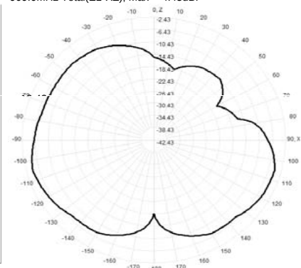
909.0MHz Total(E1-XZ), Max= -4.45dBi
