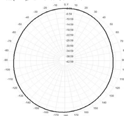
Total(H-XY), Max= -3.20dBi, CirD=5.45
