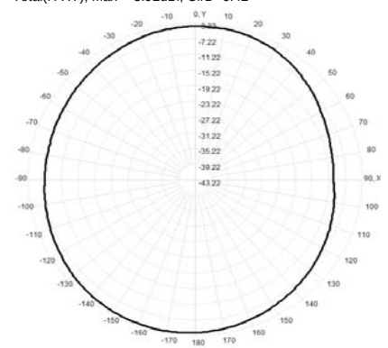
Total(H-XY), Max= -3.92dBi, CirD=6.42
