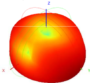
921.0MHz H+V, Eff: 19.8%
