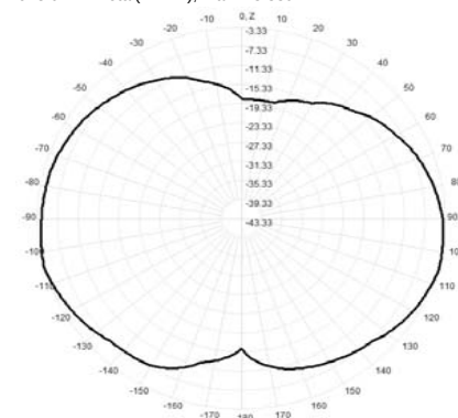
923.0MHz Total(E2-YZ), Max= -3.33dBi
