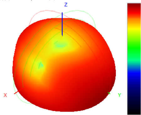
905.0MHz H+V, Eff: 24.3%
