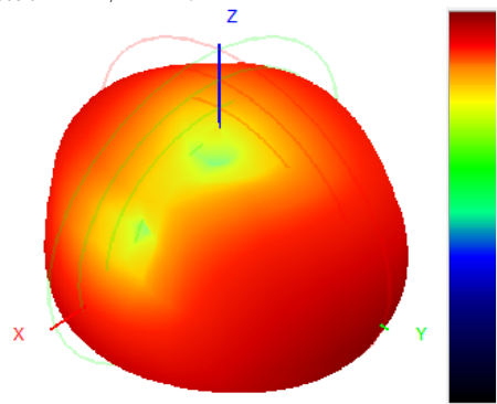
908.0MHz H+V, Eff: 24.1%
