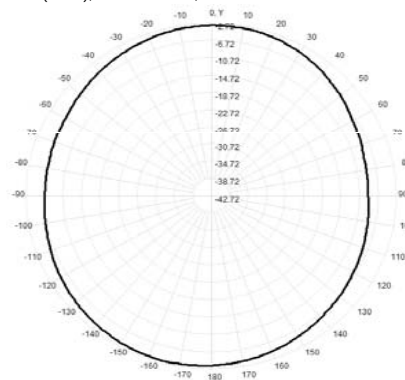
Total(H-XY), Max= -3.26dBi, CirD=5.75
