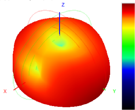
923.0MHz H+V, Eff: 19.1%
