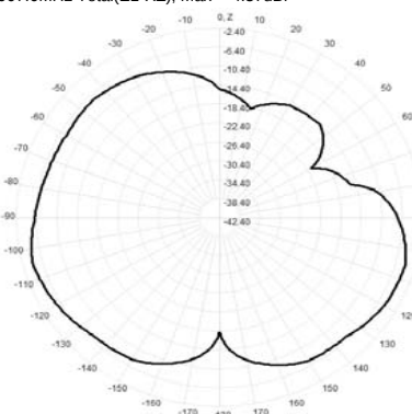
907.0MHz Total(E1-XZ), Max= -4.37dBi
