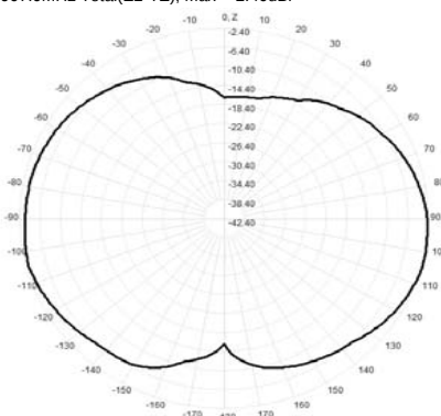
907.0MHz Total(E2-YZ), Max= -2.40dBi
