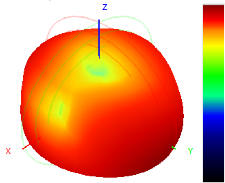
917.0MHz H+V, Eff: 20.9%
