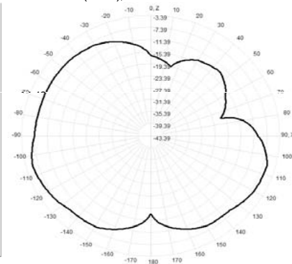
924.0MHz Total(E1-XZ), Max= -5.52dBi
