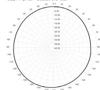
Total(H-XY), Max= -2.85dBi, CirD=5.39
