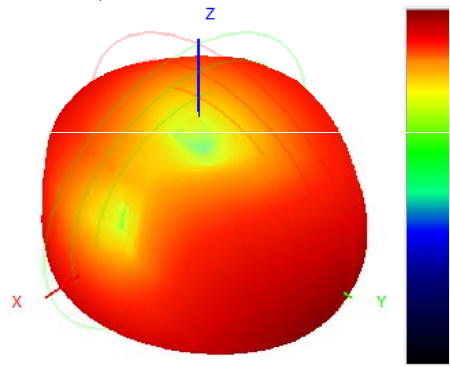
918.0MHz H+V, Eff: 20.6%
