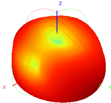
920.0MHz H+V, Eff: 20.1%
