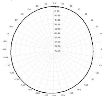
Total(H-XY), Max= -3.56dBi, CirD=5.74
