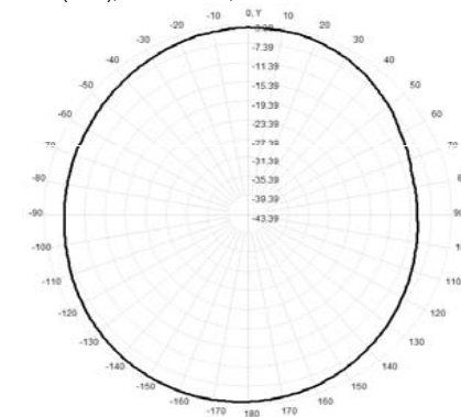
Total(H-XY), Max= -4.00dBi, CirD=6.33
