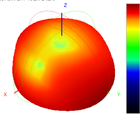
907.0MHz H+V, Eff: 24.2%
