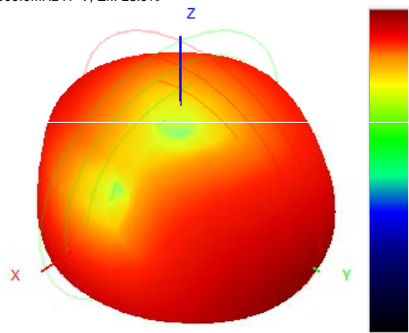
909.0MHz H+V, Eff: 23.9%
