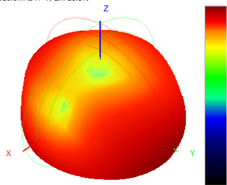
910.0MHz H+V, Eff: 23.5%
