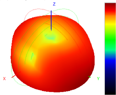
914.0MHz H+V, Eff: 22.2%
