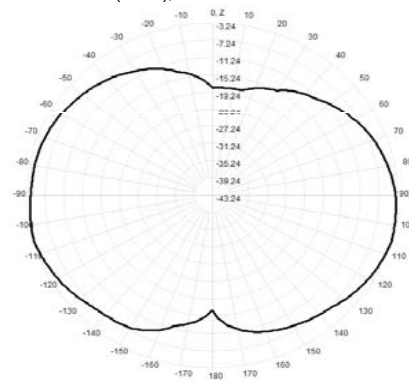
922.0MHz Total(E2-YZ), Max= -3.22dBi
