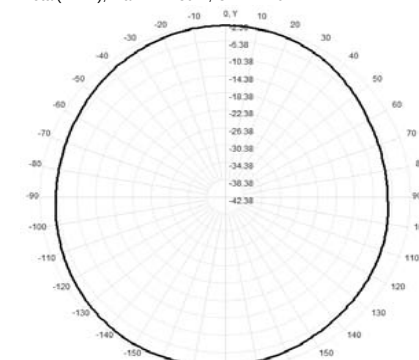
Total(H-XY), Max= -2.75dBi, CirD=4.76
