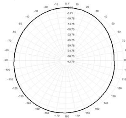
Total(H-XY), Max= -3.41dBi, CirD=5.96
