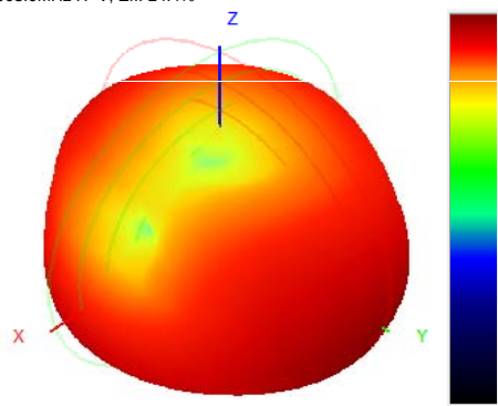
903.0MHz H+V, Eff: 24.4%
