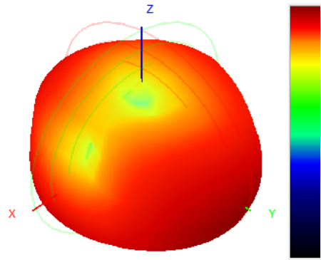
913.0MHz H+V, Eff: 22.6%
