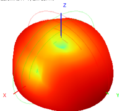
922.0MHz H+V, Eff: 19.4%
