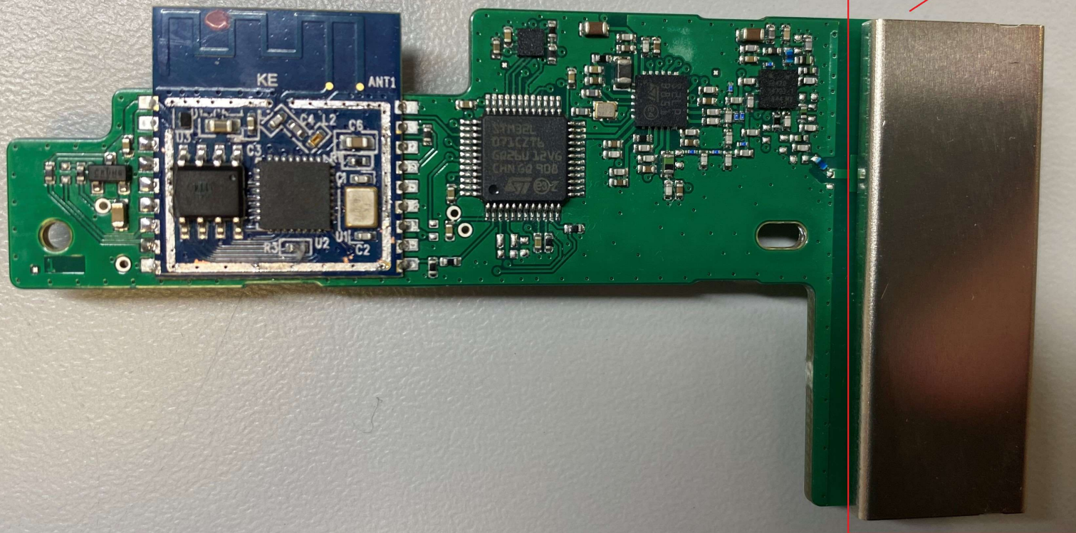
900MHz band Antenna
