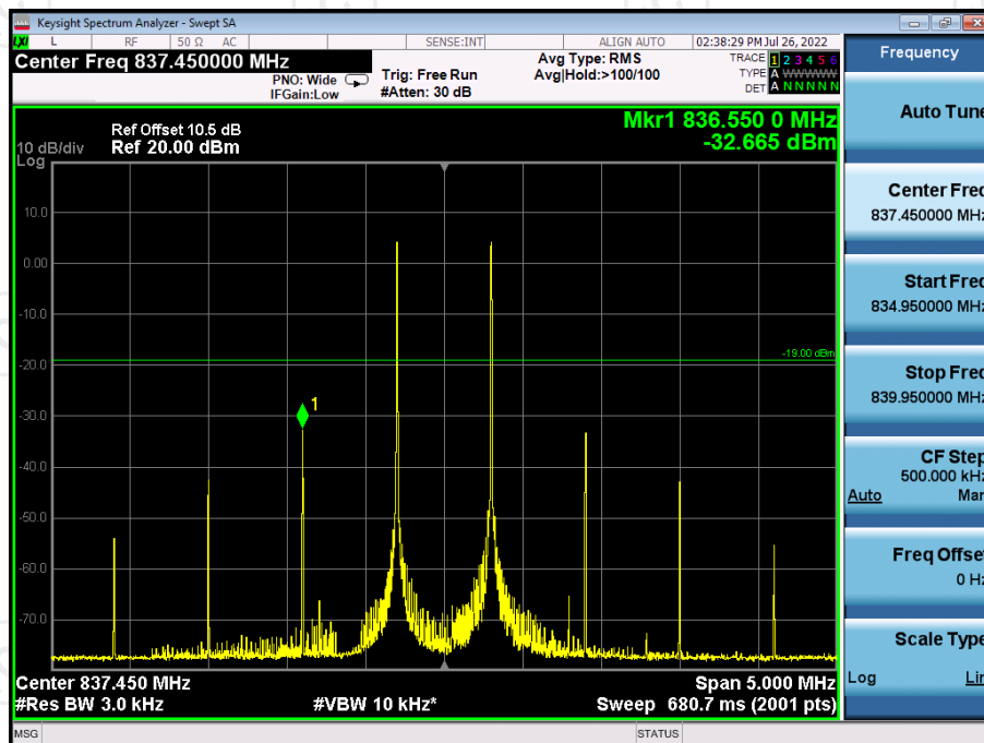
Cellular Max. Input, UL
