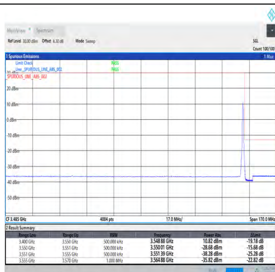
1-N78-3450-3550-30-80-H-2-DFT-PI2BPSK-Edge_1R B. Right-1@216-Ant1-1--PASS-see graph
