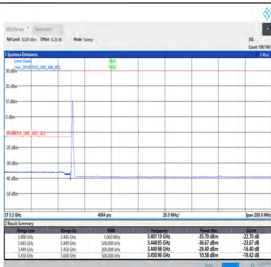
1-N78-3450-3550-30-20-L-1-DFT-PI2BPSK-Edge_1RB _Left-1@0-Ant1-1--PASS-see graph
