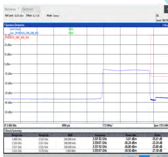
1-N78-3450-3550-30-50-H-6-CP-QPSK-Outer_Full -133@0-Ant1-1--PASS-see graph
