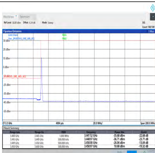
1-N78-3450-3550-30-60-L-1-DFT-PI2BPSK-Edge_1RB _Left-1@0-Ant1-1--PASS-see graph
