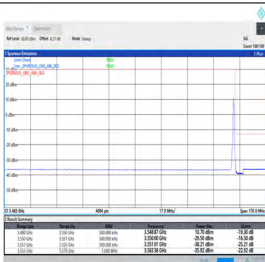
1-N78-3450-3550-30-30-H-2-DFT-PI2BPSK-Edge_1R_B_Right-1@77-Ant1-1--PASS-see graph
