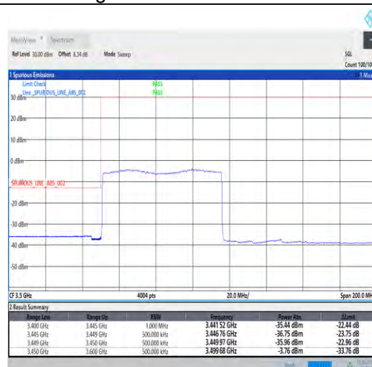
1-N78-3450-3550-30-70-L-3-DFT-PI2BPSK-Outer _Full-180@0-Ant1-1--PASS-see graph
