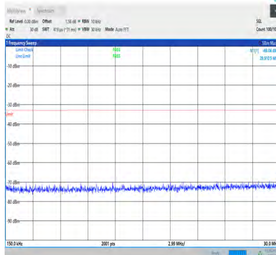
1-N78-3450-3550-30-100-L-1-DFT-QPSK-Edge_1RB _Left-1@0-0.15-30-Ant1-29.91--69.04--33-PASS
