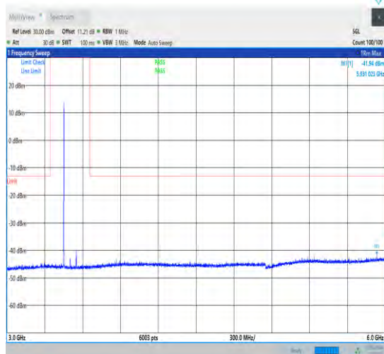
1-N78-3450-3550-30-100-H-1-DFT-QPSK-Edge_1R B_Left-1@0-3000-6000-Ant1-5931.02--41.94--13-PA SS
