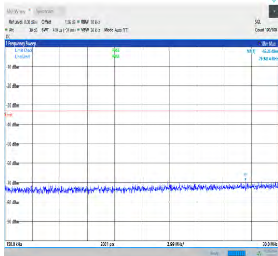
1-N78-3450-3550-30-100-M-1-DFT-QPSK-Edge_1R B_Left-1@0-0.15-30-Ant1-26.34--69.26--33-PASS
