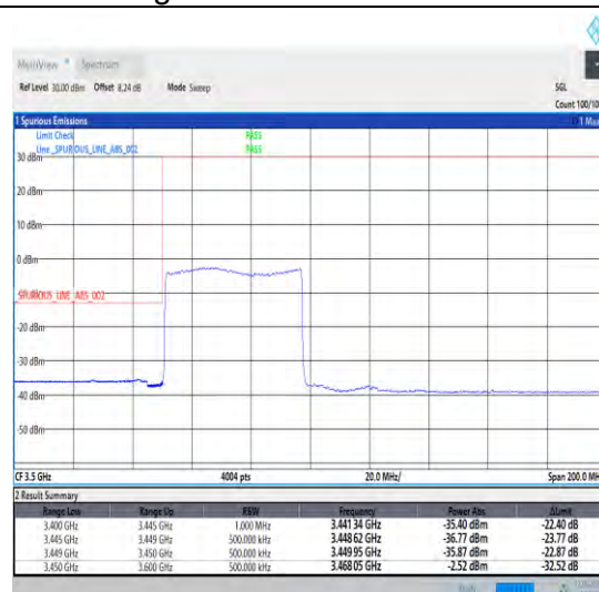
1-N78-3450-3550-30-50-L-3-DFT-PI2BPSK-Outer _Full-128@0-Ant1-1--PASS-see graph
