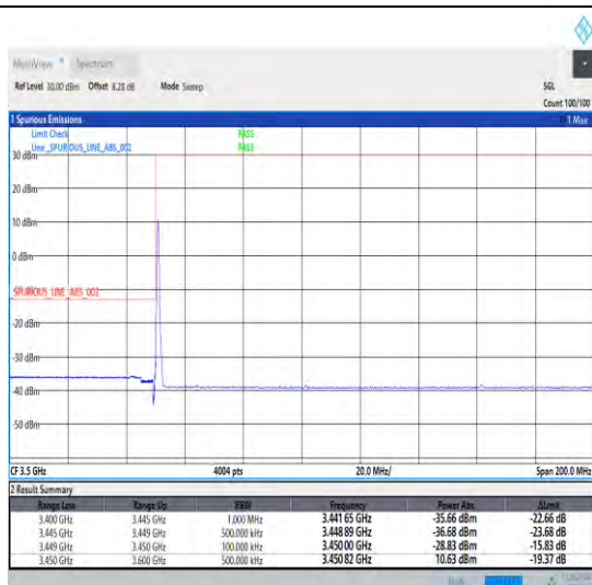
1-N78-3450-3550-30-15-L-1-DFT-PI2BPSK-Edge_1RB _Left-1@0-Ant1-1--PASS-see graph
