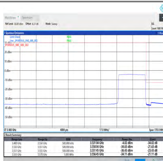
1-N78-3450-3550-30-30-H-6-CP-QPSK-Outer_Full-78@0-Ant1-1--PASS-see graph
