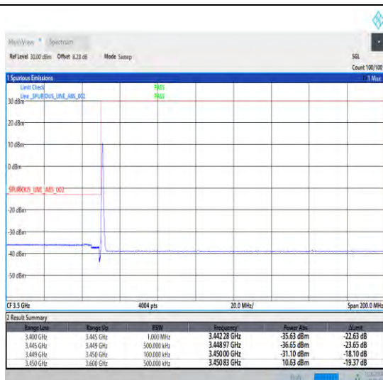
1-N78-3450-3550-30-10-L-1-DFT-PI2BPSK-Edge_1RB _Left-1@0-Ant1-1--PASS-see graph
