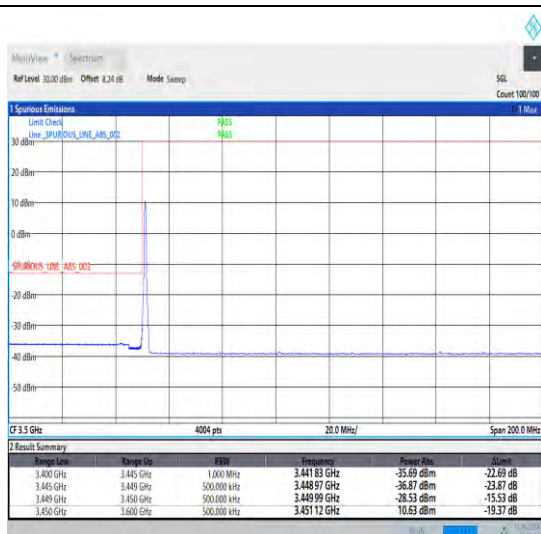
1-N78-3450-3550-30-30-L-1-DFT-PI2BPSK-Edge_1RB _Left-1@0-Ant1-1--PASS-see graph
