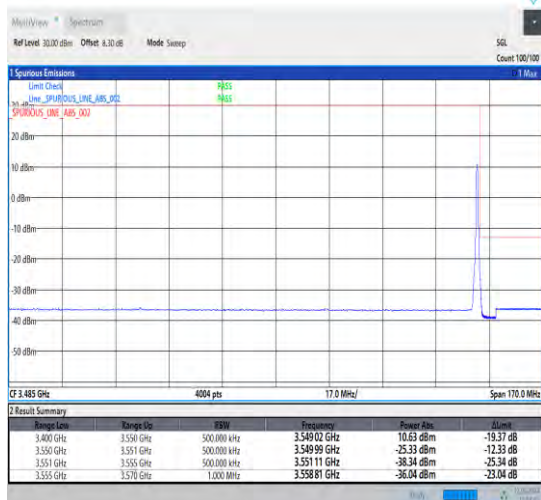
1-N78-3450-3550-30-60-H-2-DFT-PI2BPSK-Edge_1R B_Right-1@161-Ant1-1--PASS-see graph
