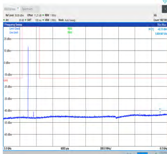
1-N78-3450-3550-30-100-M-1-DFT-QPSK-Edge_1R B_Left-1@0-3000-6000-Ant1-5859.05--42.15--13-PA SS
