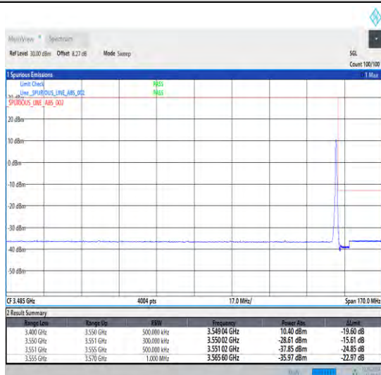
1-N78-3450-3550-30-25-H-5-CP-QPSK-Edge_1RB_Ri ght-1@64-Ant1-1--PASS-see graph
