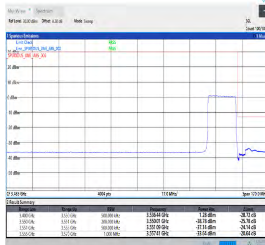
1-N78-3450-3550-30-20-H-3-DFT-PI2BPSK-Outer_Full-50@0-Ant1-1--PASS-see graph
