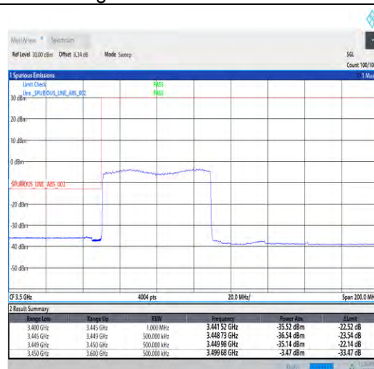
1-N78-3450-3550-30-60-L-3-DFT-PI2BPSK-Outer _Full-162@0-Ant1-1--PASS-see graph
