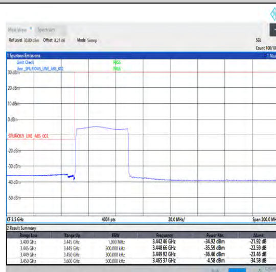
1-N78-3450-3550-30-40-L-6-CP-QPSK-Outer_Full -106@0-Ant1-1--PASS-see graph
