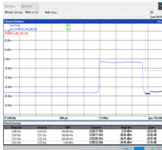
1-N78-3450-3550-30-50-H-3-DFT-PI2BPSK-Outer _Full-128@0-Ant1-1--PASS-see graph
