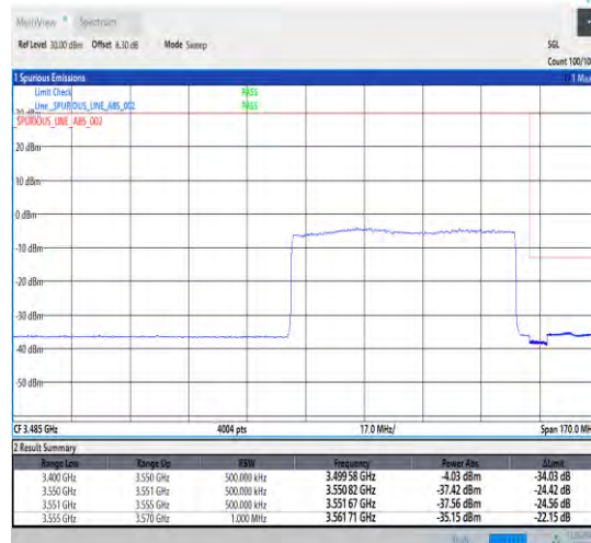
1-N78-3450-3550-30-70-H-3-DFT-PI2BPSK-Outer _Full-180@0-Ant1-1--PASS-see graph
