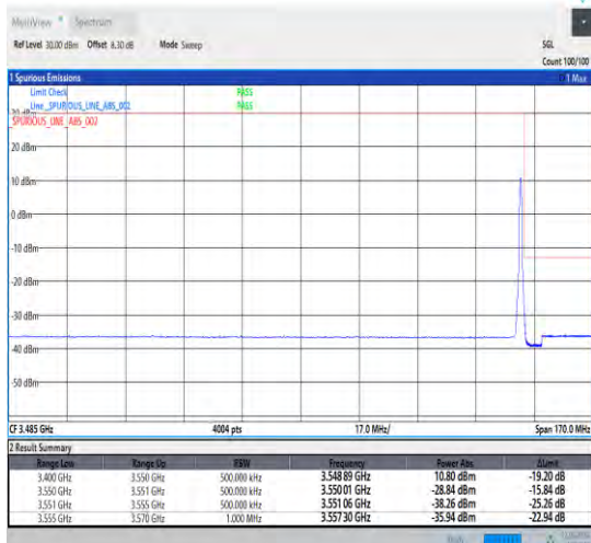
1-N78-3450-3550-30-70-H-2-DFT-PI2BPSK-Edge_1R B_Right-1@188-Ant1-1--PASS-see graph
