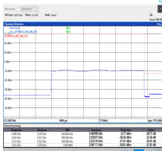
1-N78-3450-3550-30-100-H-6-CP-QPSK-Outer_Full-273@0-Ant1-1--PASS-see graph
