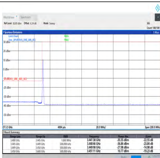
1-N78-3450-3550-30-80-L-1-DFT-PI2BPSK-Edge_1RB _Left-1@0-Ant1-1--PASS-see graph
