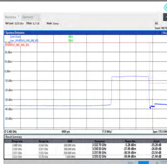
1-N78-3450-3550-30-40-H-6-CP-QPSK-Outer_Full -106@0-Ant1-1--PASS-see graph
