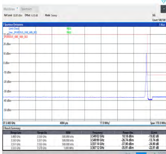
1-N78-3450-3550-30-60-H-5-CP-QPSK-Edge_1RB_Ri ght-1@161-Ant1-1--PASS-see graph
