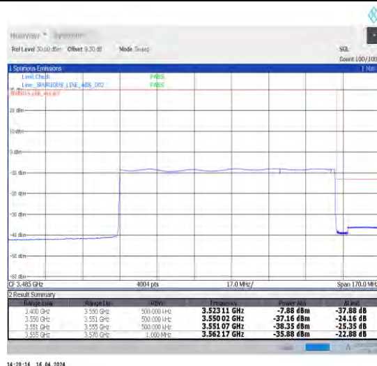
1-N78-3450-3550-30-100-H-6-CP-QPSK-Outer_Full-273@0-Ant1-1--PASS-see graph
