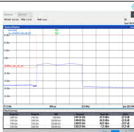
1-N78-3450-3550-30-70-L-6-CP-QPSK-Outer_Full -189@0-Ant1-1--PASS-see graph
