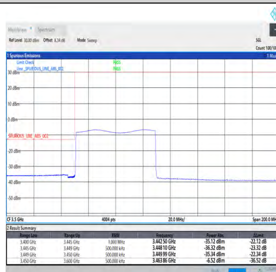
1-N78-3450-3550-30-60-L-6-CP-QPSK-Outer_Full -162@0-Ant1-1--PASS-see graph
