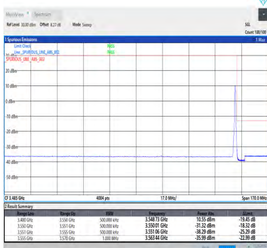
1-N78-3450-3550-30-50-H-5-CP-QPSK-Edge_1RB_Ri ght-1@132-Ant1-1--PASS-see graph
