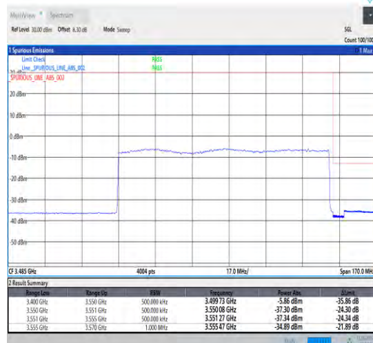
1-N78-3450-3550-30-100-H-3-DFT-PI2BPSK-Outer_Full-270@0-Ant1-1--PASS-see graph
