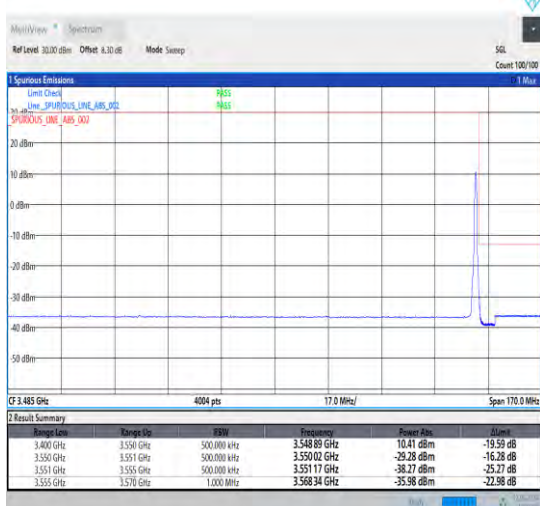
1-N78-3450-3550-30-70-H-5-CP-QPSK-Edge_1RB_Ri ght-1@188-Ant1-1--PASS-see graph
