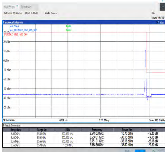
1-N78-3450-3550-30-20-H-2-DFT-PI2BPSK-Edge_1R_B_Right-1@50-Ant1-1--PASS-see graph
