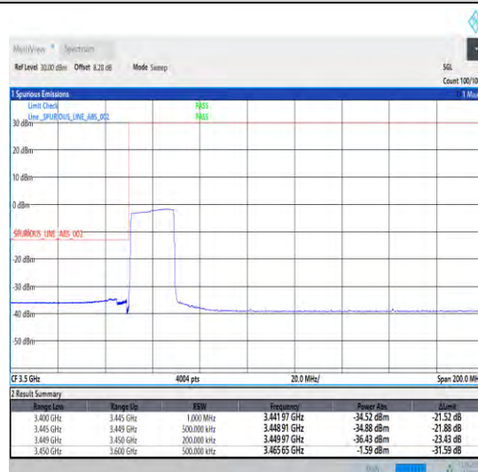
1-N78-3450-3550-30-20-L-6-CP-QPSK-Outer_Full -51@0-Ant1-1--PASS-see graph
