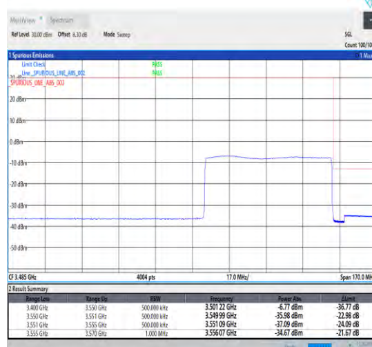
1-N78-3450-3550-30-60-H-6-CP-QPSK-Outer_Full -162@0-Ant1-1--PASS-see graph
