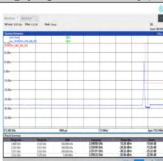
1-N78-3450-3550-30-80-H-5-CP-QPSK-Edge_1RB_Ri ght-1@216-Ant1-1--PASS-see graph
