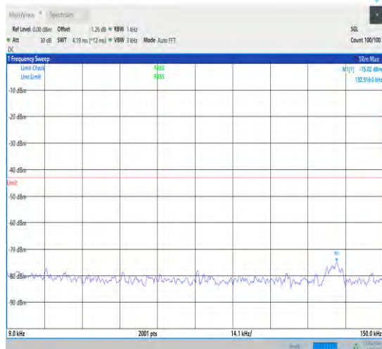
1-N78-3450-3550-30-100-L-1-DFT-QPSK-Edge_1R B_Left-1@0-0.009-0.15-Ant1-0.13--75.02--43-PASS
