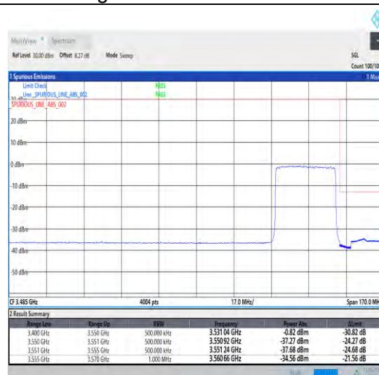
1-N78-3450-3550-30-30-H-3-DFT-PI2BPSK-Outer_Full-75@0-Ant1-1--PASS-see graph
