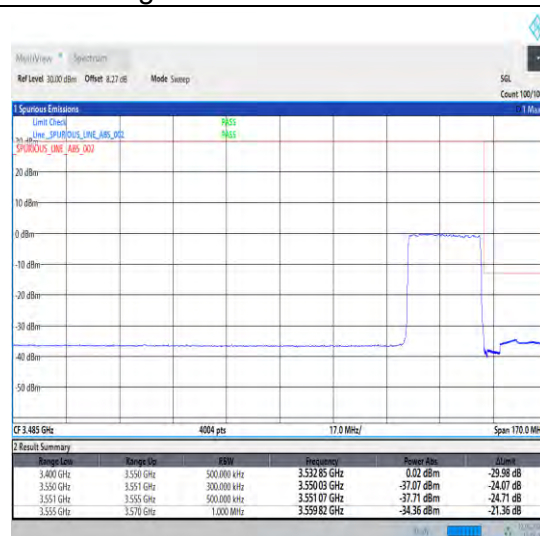
1-N78-3450-3550-30-25-H-3-DFT-PI2BPSK-Outer _Full-64@0-Ant1-1--PASS-see graph
