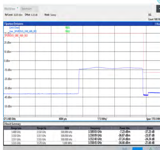
1-N78-3450-3550-30-70-H-6-CP-QPSK-Outer_Full -189@0-Ant1-1--PASS-see graph
