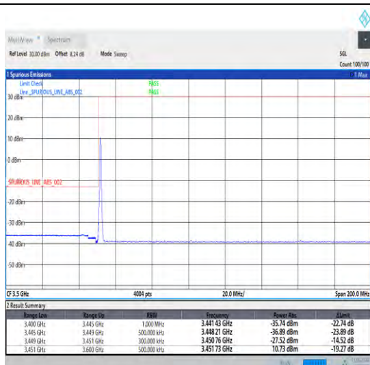
1-N78-3450-3550-30-25-L-1-DFT-PI2BPSK-Edge_1RB _Left-1@0-Ant1-1--PASS-see graph
