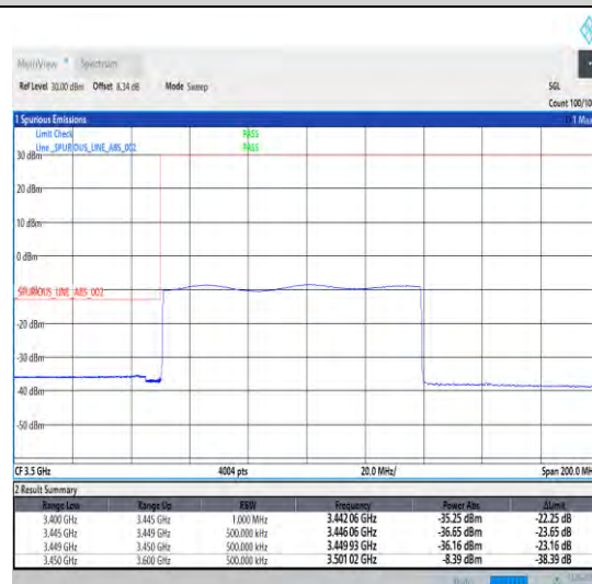
1-N78-3450-3550-30-90-L-6-CP-QPSK-Outer_Full -245@0-Ant1-1--PASS-see graph
