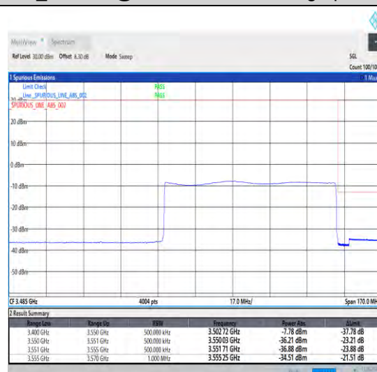
1-N78-3450-3550-30-80-H-6-CP-QPSK-Outer_Full -217@0-Ant1-1--PASS-see graph
