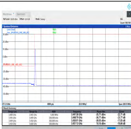
1-N78-3450-3550-30-40-L-4-CP-QPSK-Edge_1RB_Lef t-1@0-Ant1-1--PASS-see graph
