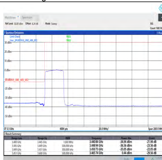
1-N78-3450-3550-30-25-L-3-DFT-PI2BPSK-Outer _Full-64@0-Ant1-1--PASS-see graph
