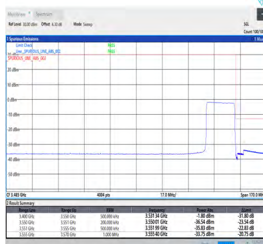
1-N78-3450-3550-30-20-H-6-CP-QPSK-Outer_Full-51@0-Ant1-1--PASS-see graph
