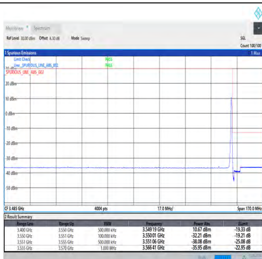
1-N78-3450-3550-30-10-H-2-DFT-PI2BPSK-Edge_1R_B_Right-1@23-Ant1-1--PASS-see graph
