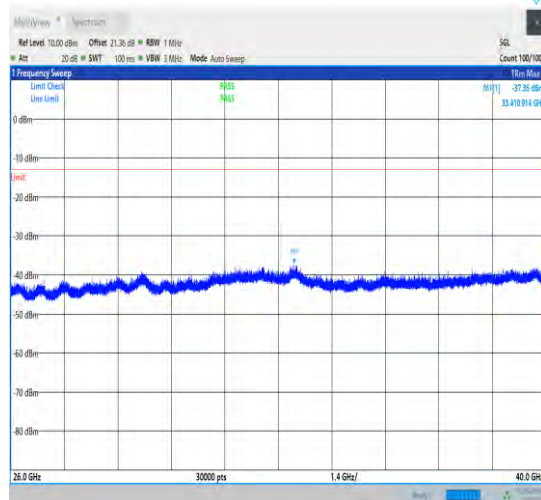
1-N78-3450-3550-30-100-M-1-DFT-QPSK-Edge_1R B_Left-1@0-26000-40000-Ant1-33410.91--37.35--13- -PASS
