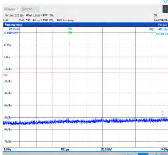
1-N78-3450-3550-30-100-M-1-DFT-QPSK-Edge_1R B_Left-1@0-1000-3000-Ant1-2921.52--48.95--13-PA SS
