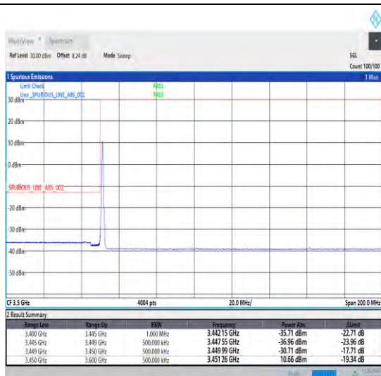
1-N78-3450-3550-30-50-L-1-DFT-PI2BPSK-Edge_1RB _Left-1@0-Ant1-1--PASS-see graph
