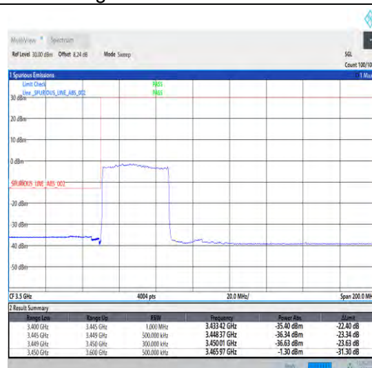
1-N78-3450-3550-30-40-L-3-DFT-PI2BPSK-Outer _Full-100@0-Ant1-1--PASS-see graph
