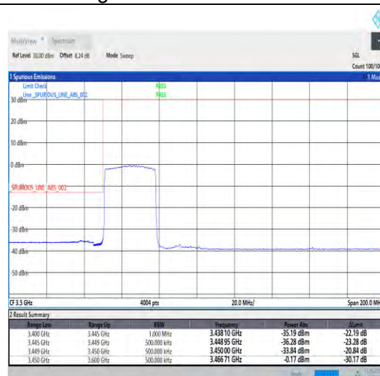
1-N78-3450-3550-30-30-L-3-DFT-PI2BPSK-Outer _Full-75@0-Ant1-1--PASS-see graph
