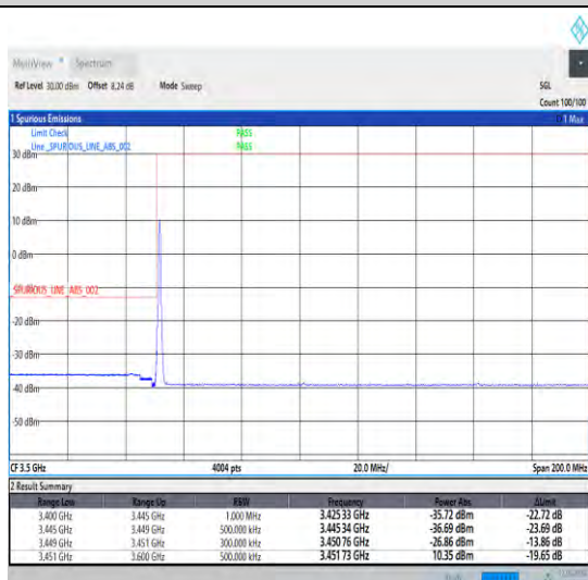
1-N78-3450-3550-30-25-L-4-CP-QPSK-Edge_1RB_Lef t-1@0-Ant1-1--PASS-see graph
