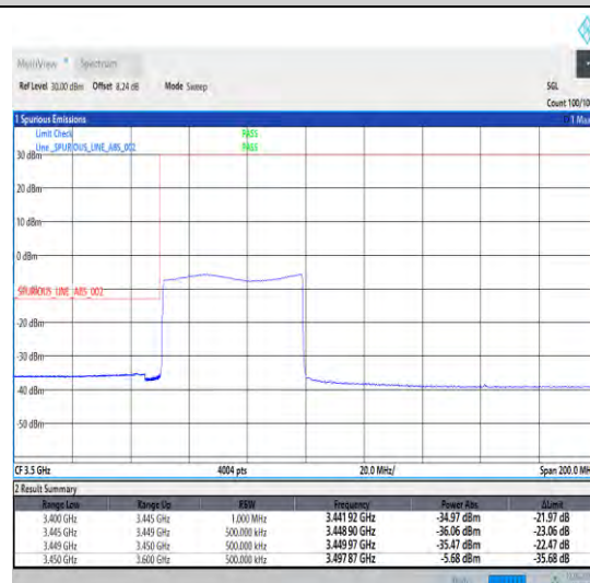
1-N78-3450-3550-30-50-L-6-CP-QPSK-Outer_Full -133@0-Ant1-1--PASS-see graph
