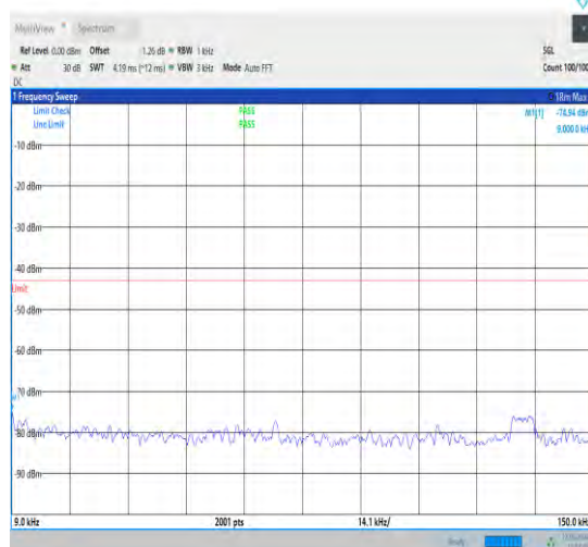
1-N78-3450-3550-30-100-M-1-DFT-QPSK-Edge_1R B_Left-1@0-0.009-0.15-Ant1-0.01--74.94--43-PASS
