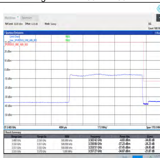
1-N78-3450-3550-30-80-H-3-DFT-PI2BPSK-Outer Full-216@0-Ant1-1--PASS-see graph
