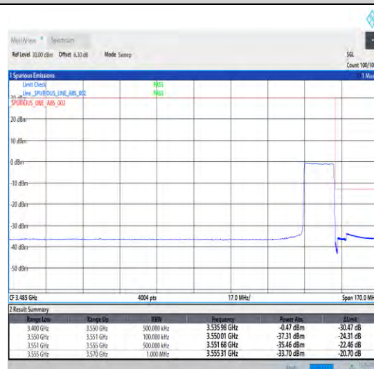
1-N78-3450-3550-30-15-H-6-CP-QPSK-Outer_Full-38@0-Ant1-1--PASS-see graph
