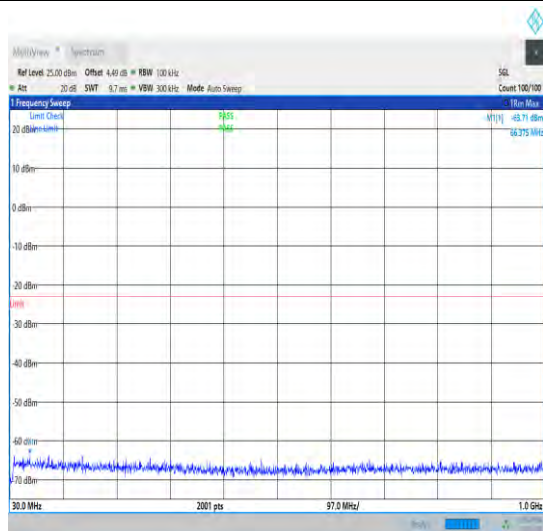
1-N78-3450-3550-30-100-L-1-DFT-QPSK-Edge_1R B_Left-1@0-30-1000-Ant1-66.38--63.71--23-PASS
