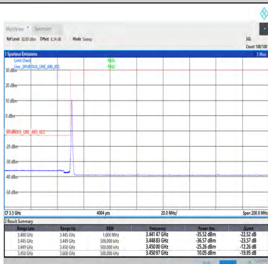
1-N78-3450-3550-30-60-L-4-CP-QPSK-Edge_1RB_Lef t-1@0-Ant1-1--PASS-see graph
