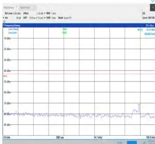
1-N78-3450-3550-30-100-H-1-DFT-QPSK-Edge_1R B_Left-1@0-0.009-0.15-Ant1-0.13--75.10--43-PASS
