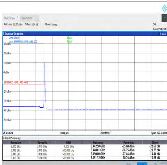
1-N78-3450-3550-30-90-L-1-DFT-PI2BPSK-Edge_1RB _Left-1@0-Ant1-1--PASS-see graph
