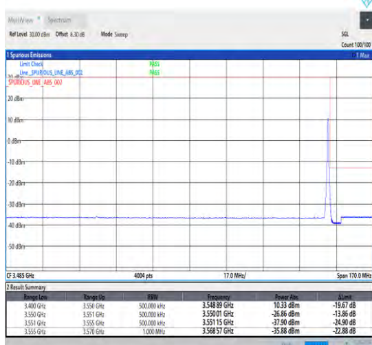
1-N78-3450-3550-30-100-H-5-CP-QPSK-Edge_1RB_Right-1@272-Ant1-1--PASS-see graph
