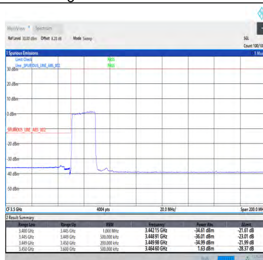
1-N78-3450-3550-30-20-L-3-DFT-PI2BPSK-Outer _Full-50@0-Ant1-1--PASS-see graph
