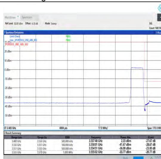
1-N78-3450-3550-30-15-H-3-DFT-PI2BPSK-Outer_Full-36@0-Ant1-1--PASS-see graph
