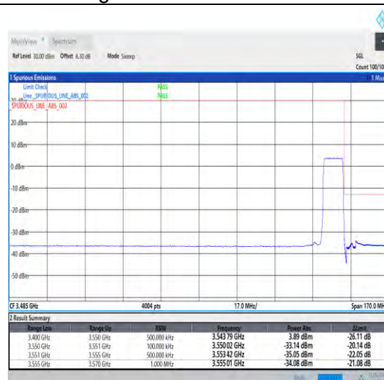
1-N78-3450-3550-30-10-H-3-DFT-PI2BPSK-Outer_Full-24@0-Ant1-1--PASS-see graph
