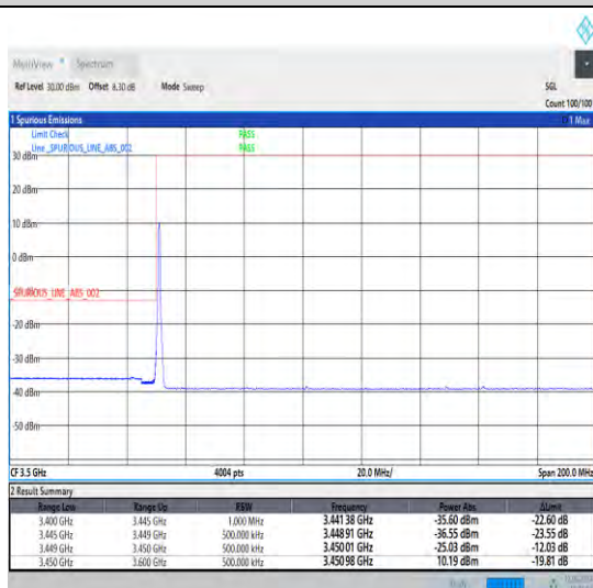
1-N78-3450-3550-30-100-L-4-CP-QPSK-Edge_1RB_Left-1@0-Ant1-1--PASS-see graph
