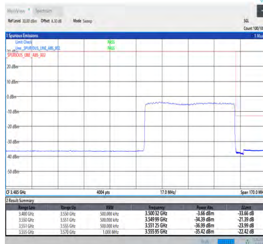
1-N78-3450-3550-30-60-H-3-DFT-PI2BPSK-Outer _Full-162@0-Ant1-1--PASS-see graph
