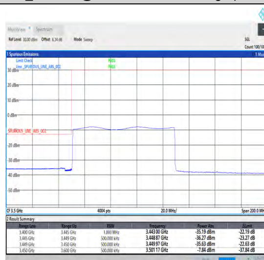
1-N78-3450-3550-30-80-L-6-CP-QPSK-Outer_Full -217@0-Ant1-1--PASS-see graph
