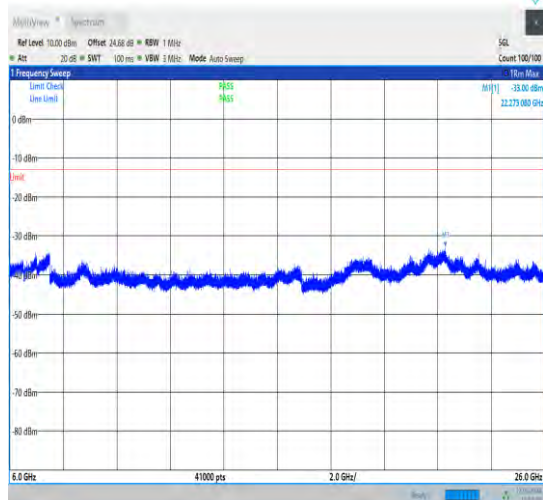
1-N78-3450-3550-30-100-M-1-DFT-QPSK-Edge_1R B_Left-1@0-6000-26000-Ant1-22273.08--33.00--13- PASS
