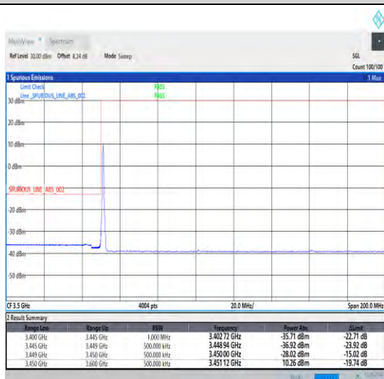
1-N78-3450-3550-30-30-L-4-CP-QPSK-Edge_1RB_Lef t-1@0-Ant1-1--PASS-see graph
