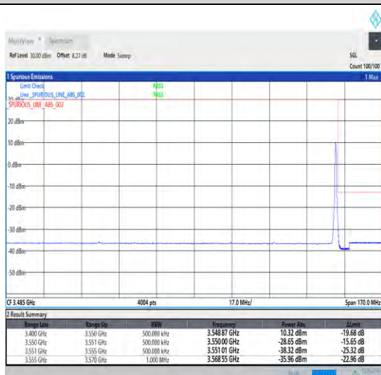
1-N78-3450-3550-30-30-H-5-CP-QPSK-Edge_1RB_Right-1@77-Ant1-1--PASS-see graph
