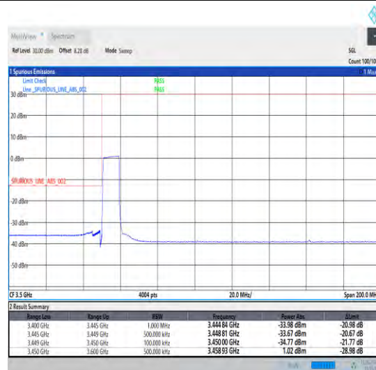
1-N78-3450-3550-30-10-L-6-CP-QPSK-Outer_Full -24@0-Ant1-1--PASS-see graph
