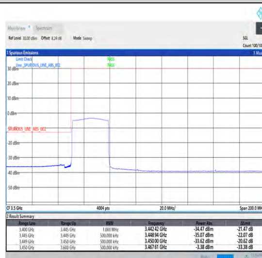
1-N78-3450-3550-30-30-L-6-CP-QPSK-Outer_Full -78@0-Ant1-1--PASS-see graph
