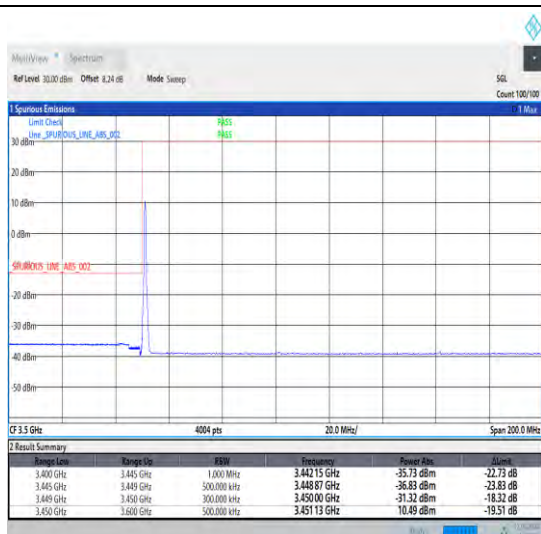
1-N78-3450-3550-30-40-L-1-DFT-PI2BPSK-Edge_1RB _Left-1@0-Ant1-1--PASS-see graph
