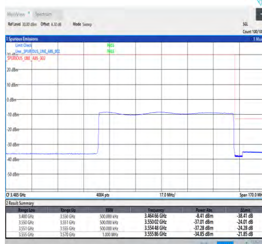
1-N78-3450-3550-30-90-H-6-CP-QPSK-Outer_Full -245@0-Ant1-1--PASS-see graph
