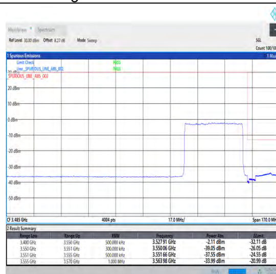
1-N78-3450-3550-30-40-H-3-DFT-PI2BPSK-Outer _Full-100@0-Ant1-1--PASS-see graph
