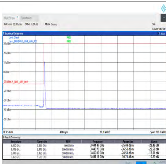
1-N78-3450-3550-30-70-L-1-DFT-PI2BPSK-Edge_1RB _Left-1@0-Ant1-1--PASS-see graph
