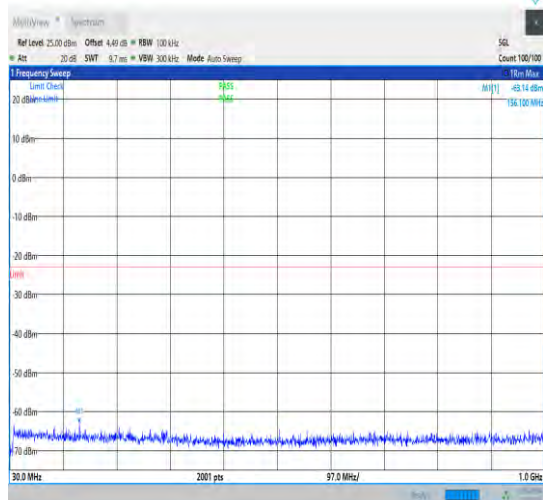
1-N78-3450-3550-30-100-H-1-DFT-QPSK-Edge_1R B_Left-1@0-30-1000-Ant1-156.10--63.14--23-PASS
