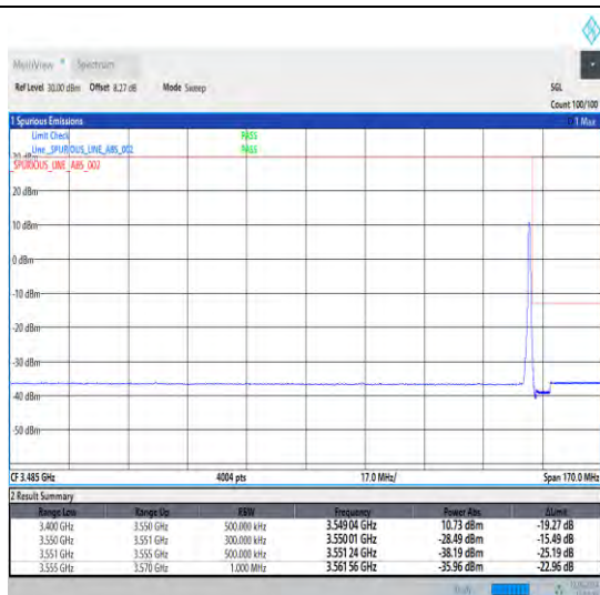
1-N78-3450-3550-30-25-H-2-DFT-PI2BPSK-Edge_1R B_Right-1@64-Ant1-1--PASS-see graph
