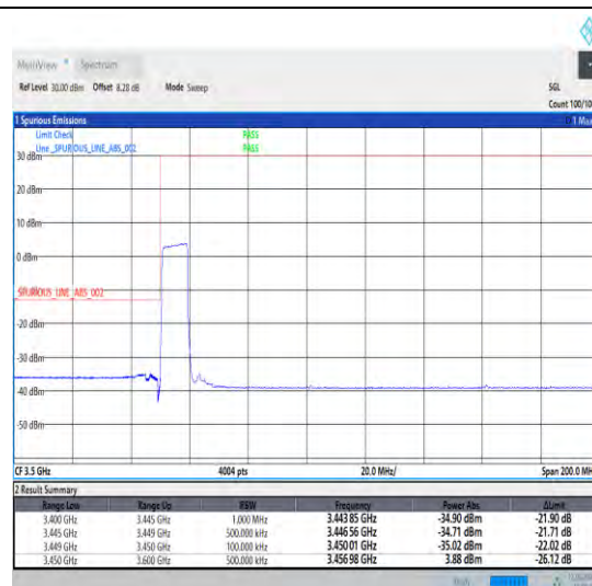
1-N78-3450-3550-30-10-L-3-DFT-PI2BPSK-Outer _Full-24@0-Ant1-1--PASS-see graph
