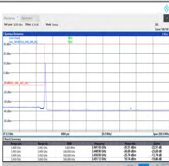
1-N78-3450-3550-30-90-L-4-CP-QPSK-Edge_1RB_Lef t-1@0-Ant1-1--PASS-see graph
