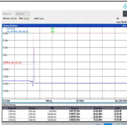
1-N78-3450-3550-30-15-L-4-CP-QPSK-Edge_1RB_Lef t-1@0-Ant1-1--PASS-see graph
