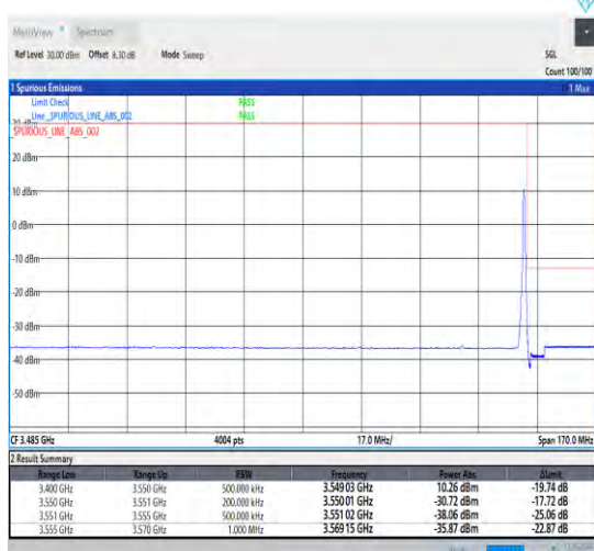
1-N78-3450-3550-30-20-H-5-CP-QPSK-Edge_1RB_Right-1@50-Ant1-1--PASS-see graph
