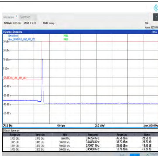
1-N78-3450-3550-30-100-L-1-DFT-PI2BPSK-Edge_1R_B_Left-1@0-Ant1-1--PASS-see graph
