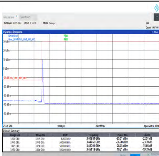
1-N78-3450-3550-30-70-L-4-CP-QPSK-Edge_1RB_Lef t-1@0-Ant1-1--PASS-see graph
