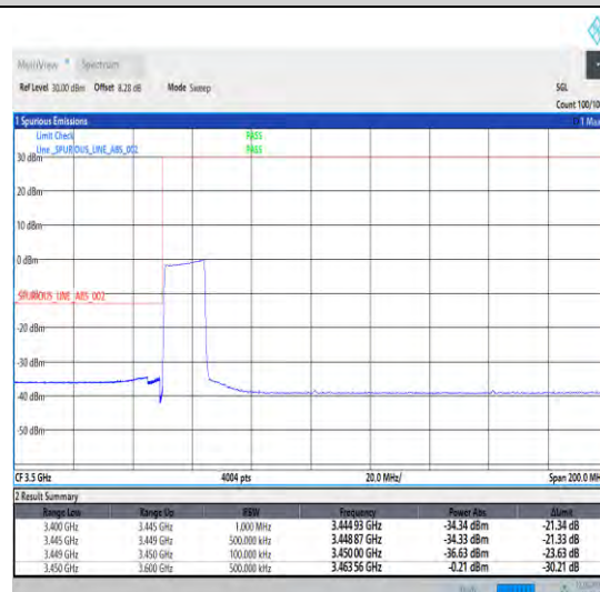
1-N78-3450-3550-30-15-L-6-CP-QPSK-Outer_Full -38@0-Ant1-1--PASS-see graph
