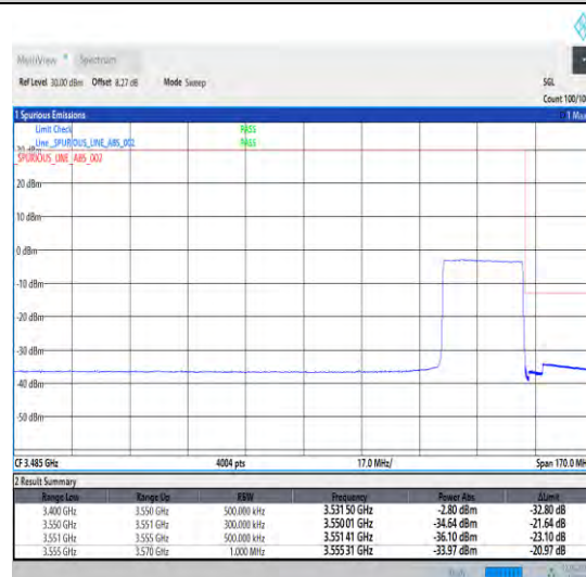
1-N78-3450-3550-30-25-H-6-CP-QPSK-Outer_Full -65@0-Ant1-1--PASS-see graph
