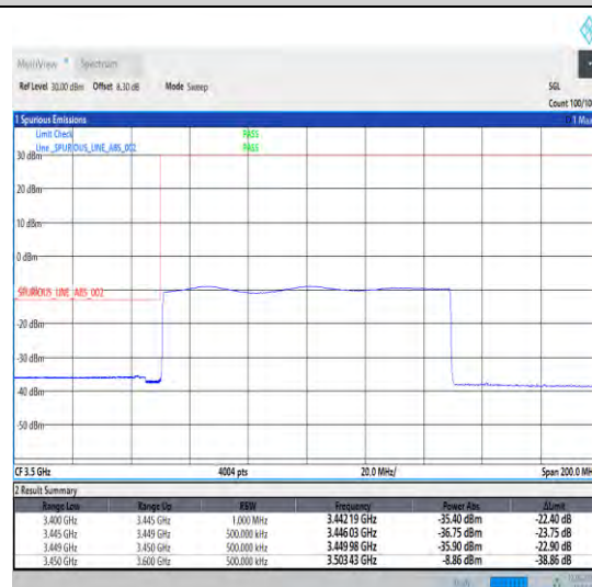
1-N78-3450-3550-30-100-L-6-CP-QPSK-Outer_Full-273@0-Ant1-1--PASS-see graph
