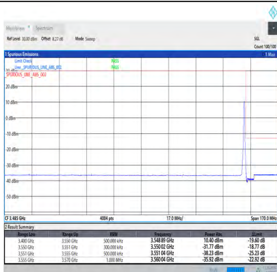
1-N78-3450-3550-30-40-H-5-CP-QPSK-Edge_1RB_Ri ght-1@105-Ant1-1--PASS-see graph
