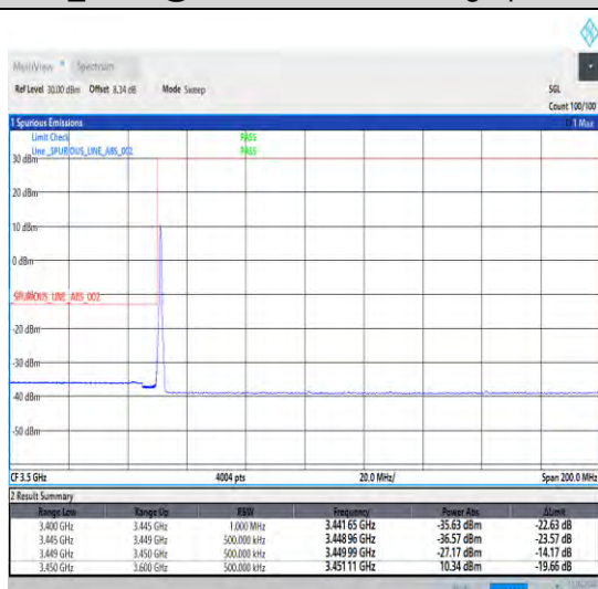
1-N78-3450-3550-30-80-L-4-CP-QPSK-Edge_1RB_Lef t-1@0-Ant1-1--PASS-see graph
