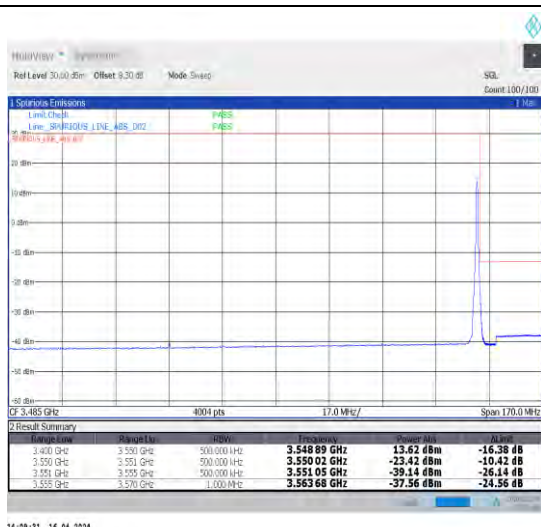
1-N78-3450-3550-30-100-H-2-DFT-PI2BPSK-Edge_1R_B_Right-1@272-Ant1-1--PASS-see graph
