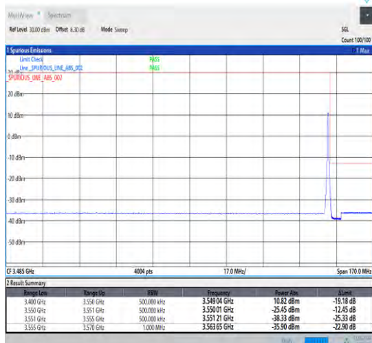
1-N78-3450-3550-30-100-H-2-DFT-PI2BPSK-Edge_1R_B_Right-1@272-Ant1-1--PASS-see graph
