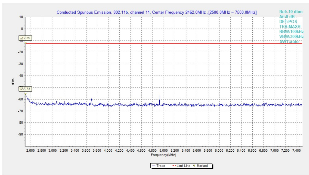
Fig.A.6.1.20 Conducted Spurious Emission (802.11b, Ch11, 2.5 GHz-7.5 GHz)
