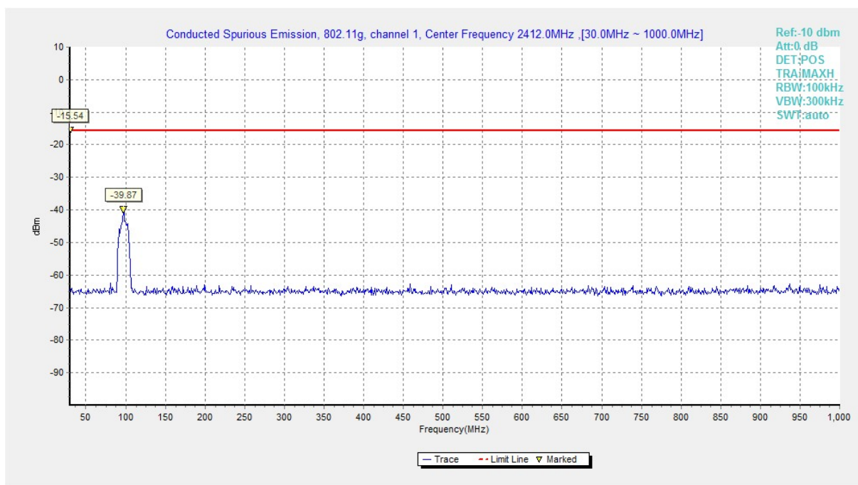
Fig.A.6.1.26 Conducted Spurious Emission (802.11g, Ch1, 30 MHz-1 GHz)
