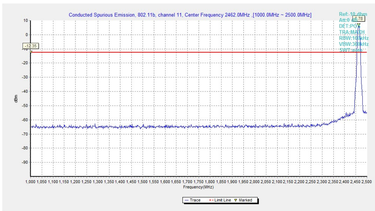
Fig.A.6.1.19 Conducted Spurious Emission (802.11b, Ch11, 1 GHz-2.5 GHz)
