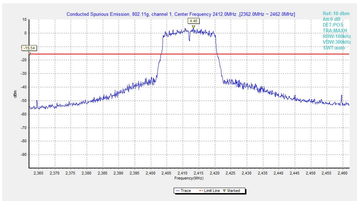
Fig.A.6.1.25 Conducted Spurious Emission (802.11g, Ch1, Center Frequency)
