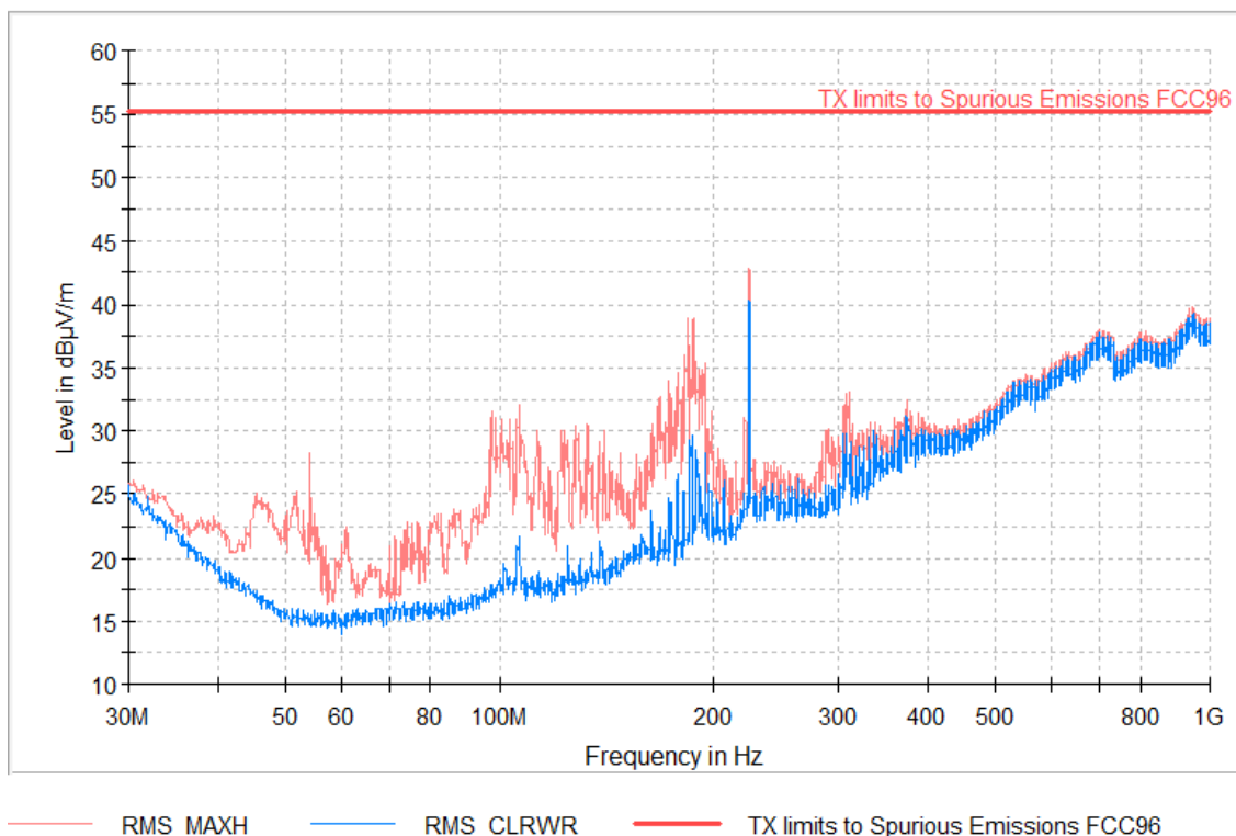
RF_FCC_Part96_E Field_30MHz_1GHz
