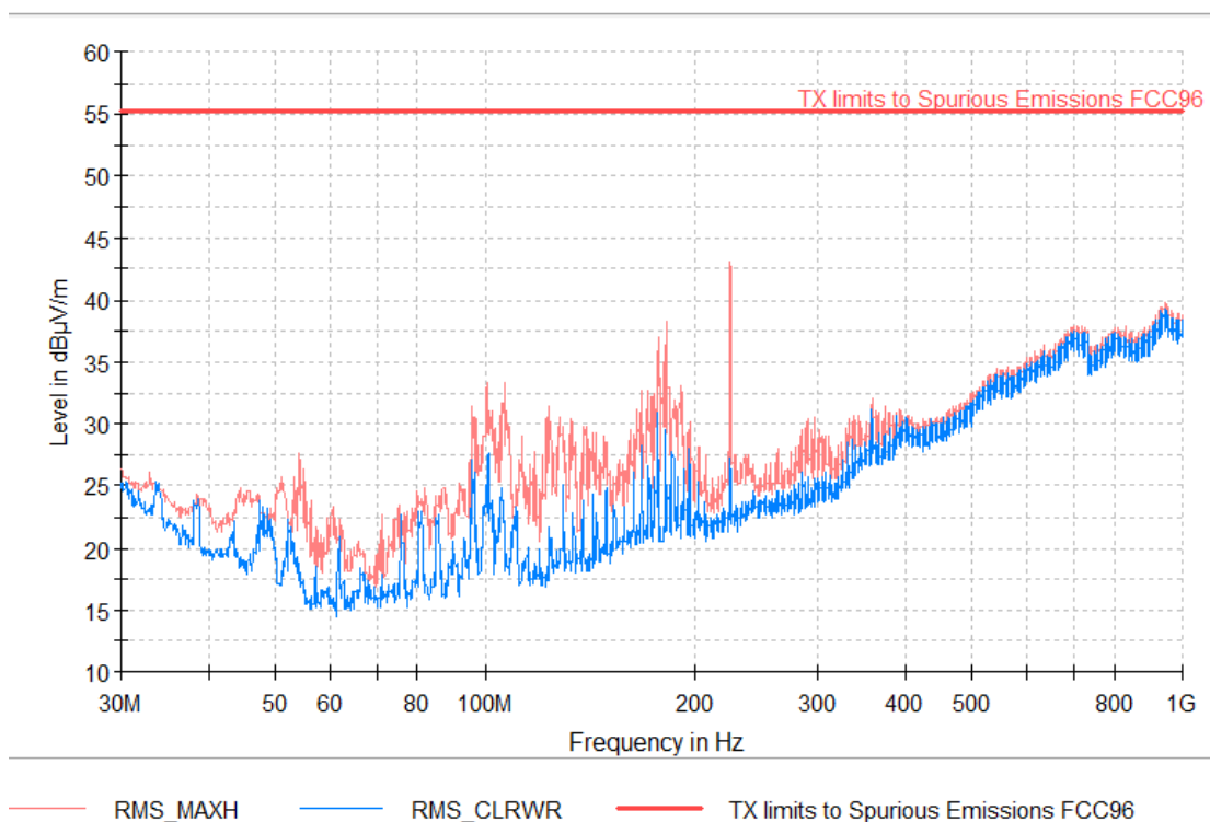
RF_FCC_Part96_E Field_30MHz_1GHz
