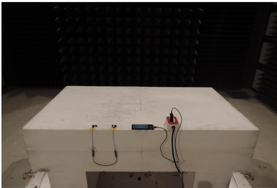
Rear View
