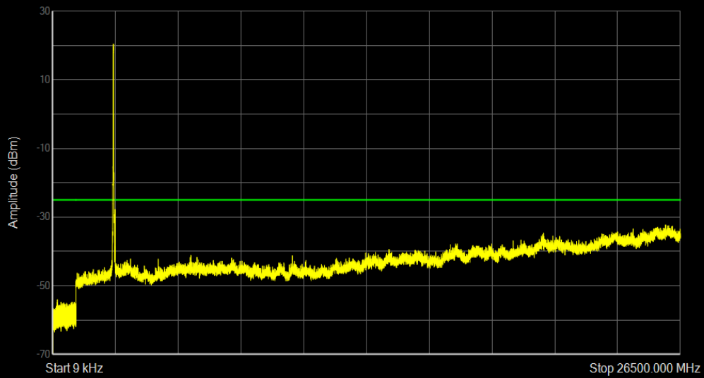
Band38 QPSK BW=20MHz Channel=37850 RB Size=100 Position=#0
