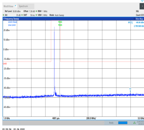
1-N66-PC3-15-40-M-1-DFT-PI2BPSK-Inner_1RB_Le ft-1@1-1000-3000-Ant0--44.44--13-PASS
