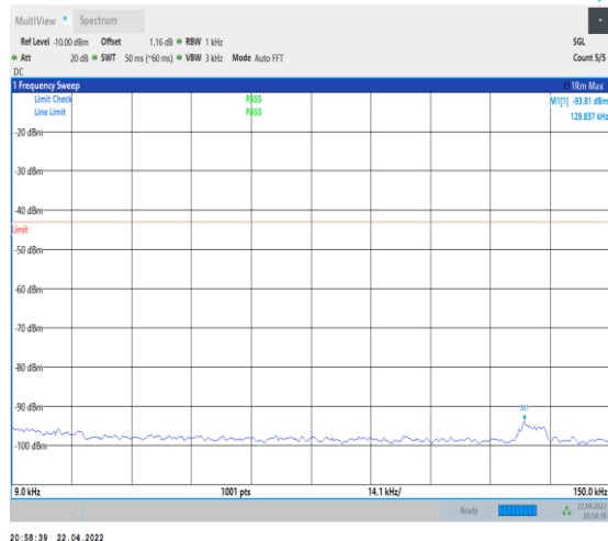
1-N66-PC3-15-40-L-1-DFT-PI2BPSK-Inner_1RB_Le ft-1@1-0.009-0.15-Ant0--93.81--43-PASS
