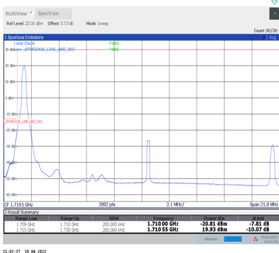
1-N66-PC3-15-20-L-4-CP-QPSK-Edge_1RB_Left-1@0-Ant0-seegraph-PASS-see graph
