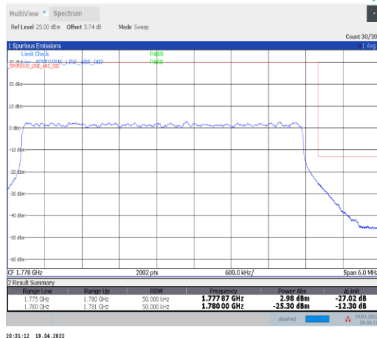
1-N66-PC3-15-5-H-3-DFT-PI2BPSK-Outer_Full-25@0-Ant0-seegraph-PASS-see graph
