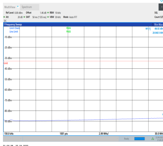
1-N66-PC3-15-40-H-1-DFT-PI2BPSK-Inner_1RB_Lef t-1@1-0.15-30-Ant0--86.92--33-PASS
