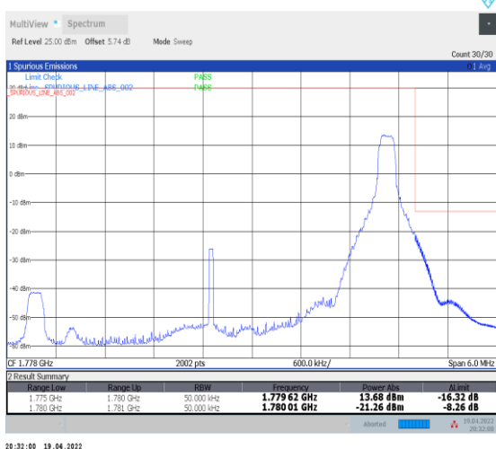
1-N66-PC3-15-5-H-5-CP-QPSK-Edge_1RB_Right-1@24-Ant0-seegraph-PASS-see graph
