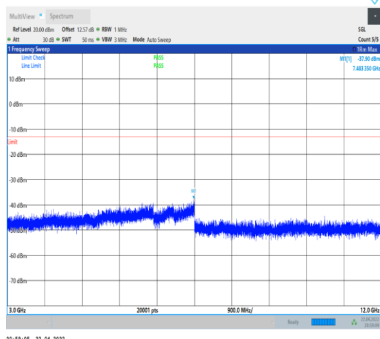
1-N66-PC3-15-40-L-1-DFT-PI2BPSK-Inner_1RB_Le ft-1@1-3000-12000-Ant0--37.90--13-PASS
