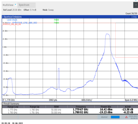
1-N66-PC3-15-5-H-2-DFT-PI2BPSK-Edge_1RB_Right-1@24-Ant0-seegraph-PASS-see graph
