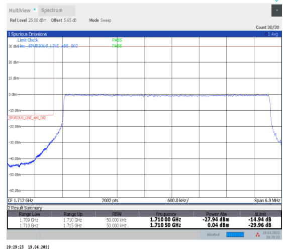
1-N66-PC3-15-5-L-6-CP-QPSK-Outer_Full-25@0-Ant0-seegraph-PASS-see graph
