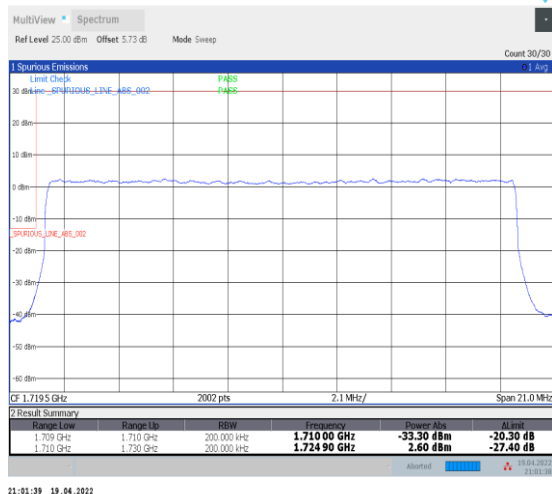
1-N66-PC3-15-20-L-3-DFT-PI2BPSK-Outer_Full-100@0-Ant0-seegraph-PASS-see graph
