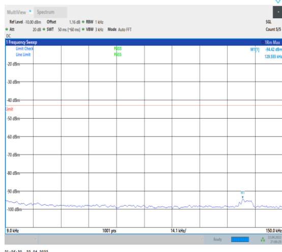
1-N66-PC3-15-40-H-1-DFT-PI2BPSK-Inner_1RB_Lef t-1@1-0.009-0.15-Ant0--94.42--43-PASS
