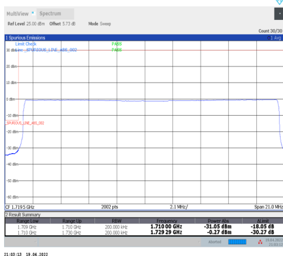
1-N66-PC3-15-20-L-6-CP-QPSK-Outer_Full-106@0-Ant0-seegraph-PASS-see graph
