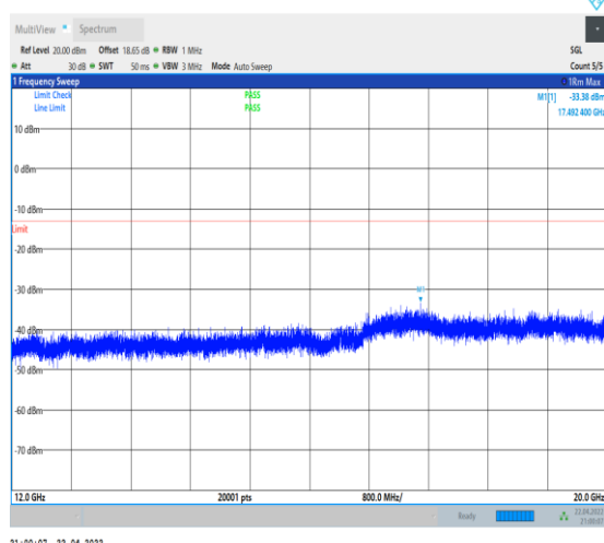
1-N66-PC3-15-40-M-1-DFT-PI2BPSK-Inner_1RB_Le ft-1@1-12000-20000-Ant0--33.38--13-PASS
