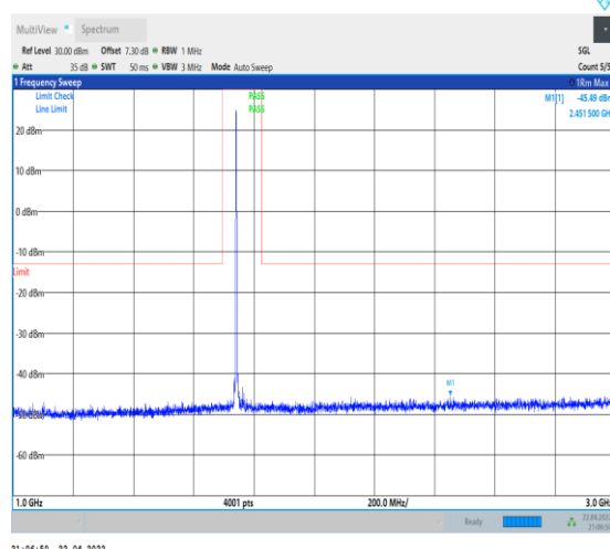
1-N66-PC3-15-40-H-1-DFT-PI2BPSK-Inner_1RB_Lef t-1@1-1000-3000-Ant0--45.49--13-PASS
