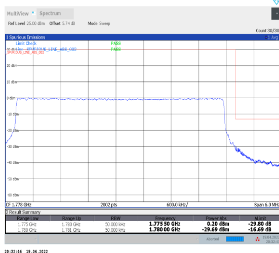
1-N66-PC3-15-5-H-6-CP-QPSK-Outer_Full-25@0-Ant0-seegraph-PASS-see graph
