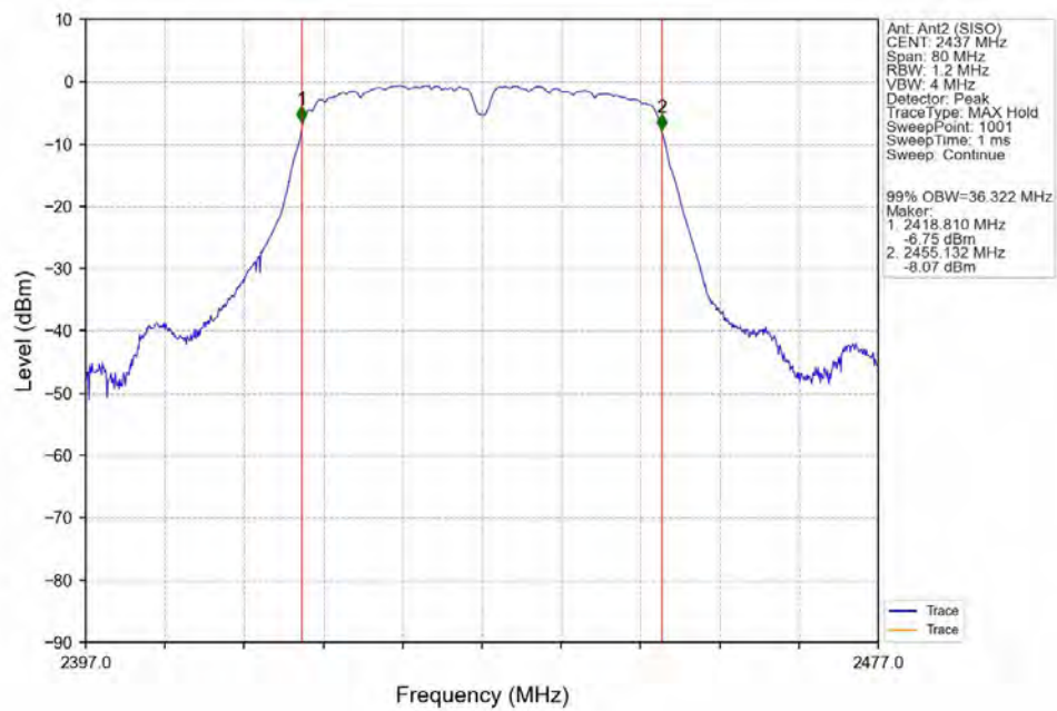
802.11ax(HEW40)_MCH_2437MHz_Ant2 (SISO)_NTNV
