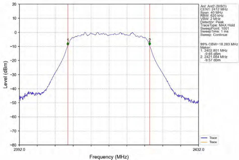
802.11ax(HEW20)_LCH_2412MHz_Ant2 (SISO)_NTNV
