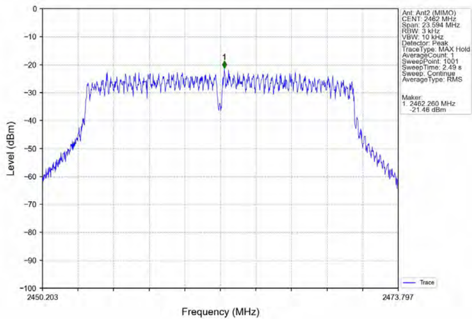
802.11ax(HEW20)_HCH_2462MHz_Ant2 (MIMO)_NTNV
