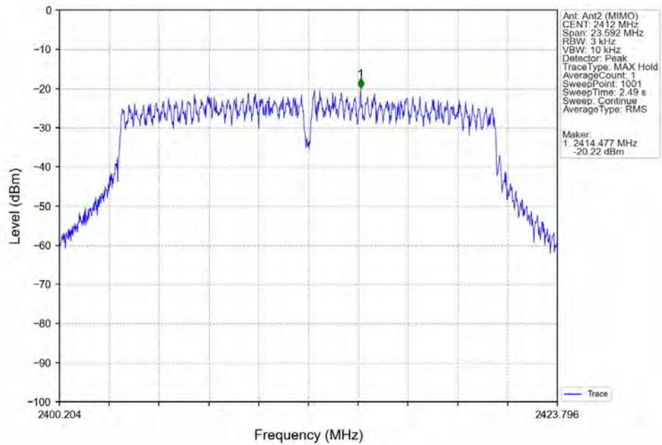
802.11ax(HEW20)_LCH_2412MHz_Ant2 (MIMO)_NTNV
