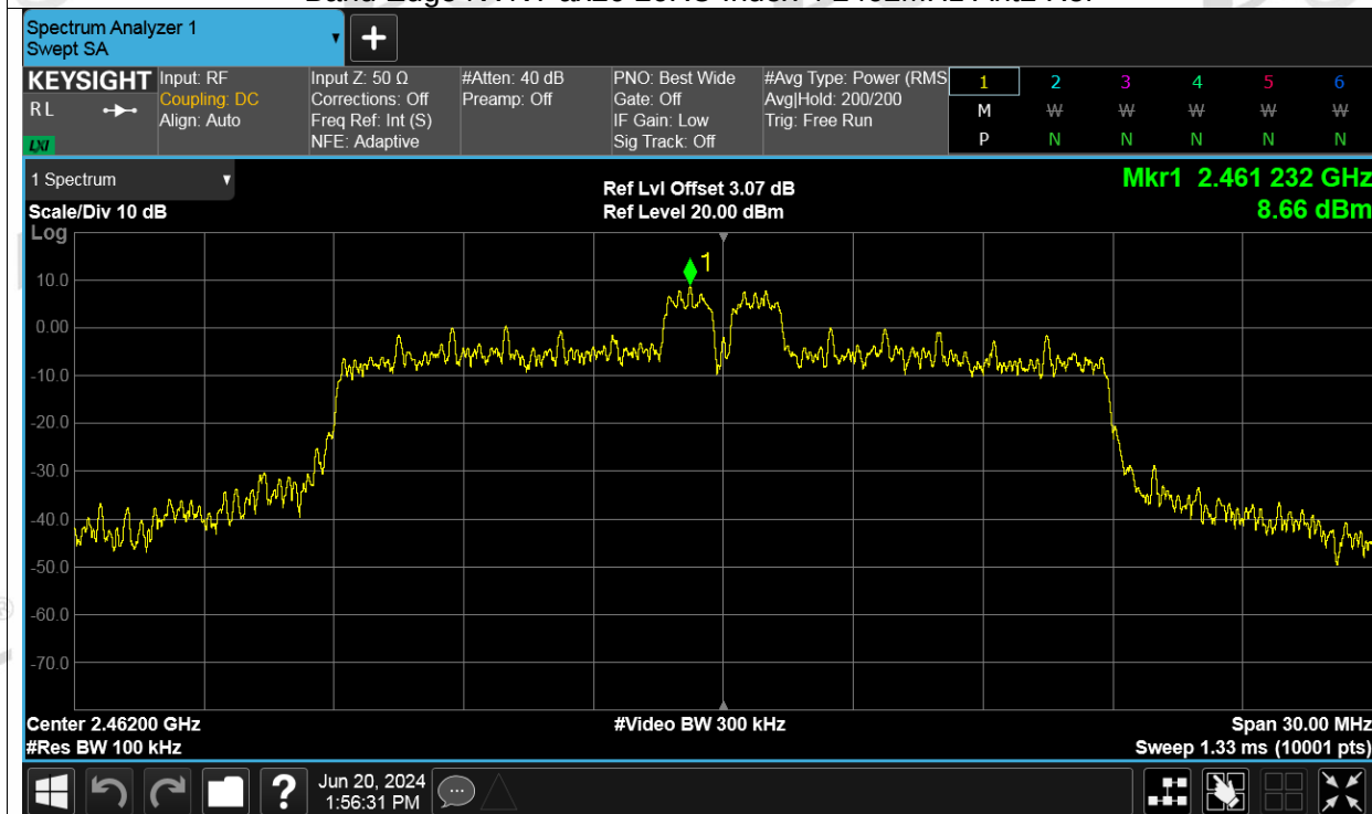
Band Edge NVNT ax20 26RU Index 4 2462MHz Ant2 Emission
