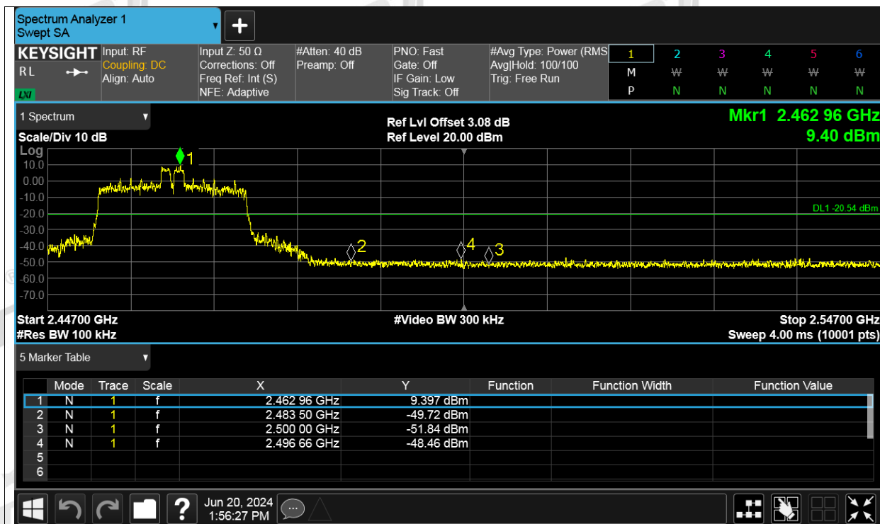
Band Edge NVNT ax20 26RU Index 4 2462MHz Ant2 Ref
