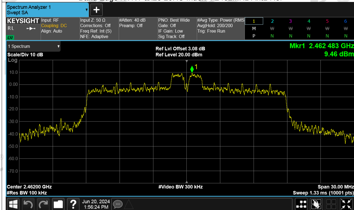
Band Edge NVNT ax20 26RU Index 4 2462MHz Ant1 Emission
