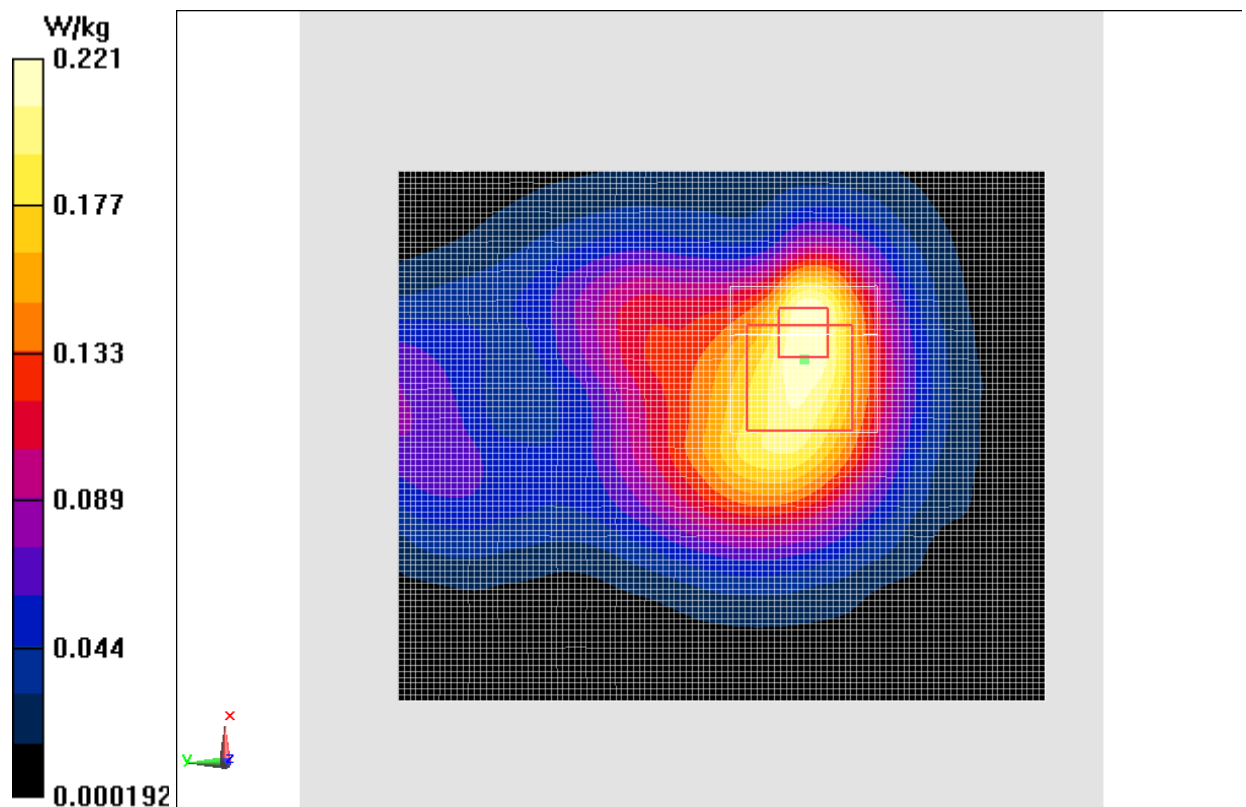
Fig.8 2450 MHz CH11
