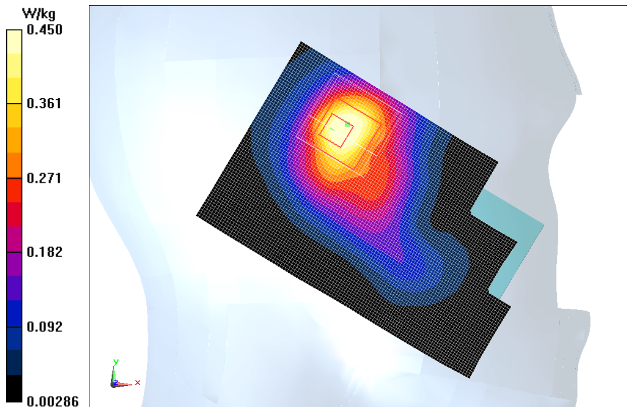
Fig.7 2450 MHz CH11
