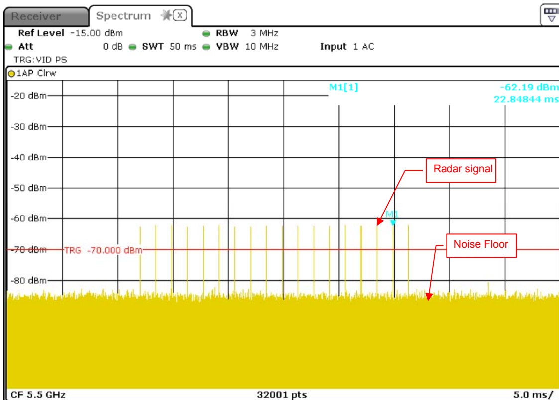
Radar Signal 0
