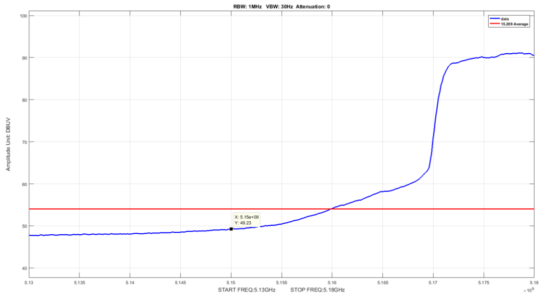
Figure 13: Band Edge BW 20M Ch 5180M 802.11n Average
