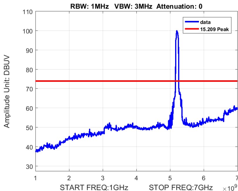
Figure 8: Radiated Spurious Emissions 1-7GHz BW 80M Ch 5210M 802.11ac Peak
