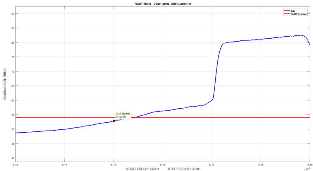
Figure 15: Band Edge BW 40M Ch 5190M 802.11n Average
