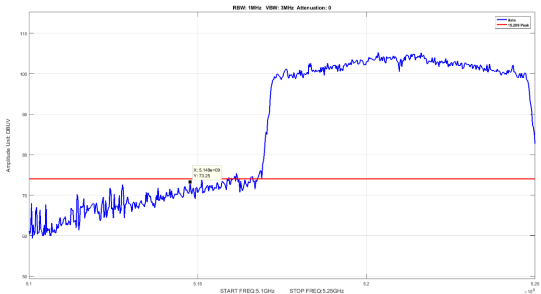
Figure 18: Band Edge BW 80M Ch 5210M 802.11ac Peak
