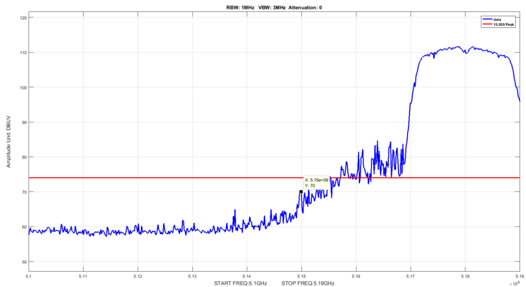
Figure 14: Band Edge BW 20M Ch 5180M 802.11n Peak
