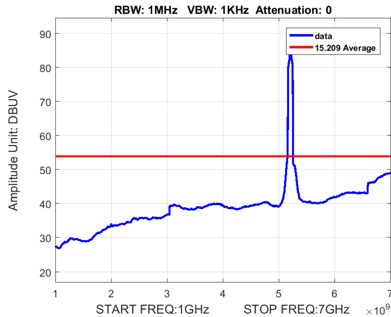
Figure 7: Radiated Spurious Emissions 1-7GHz BW 80M Ch 5210M 802.11ac Average
