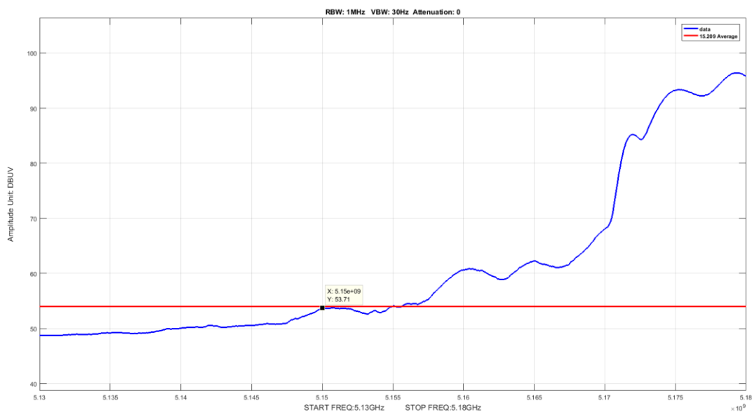
Figure 11: Band Edge BW 20M Ch 5180M 802.11a Average
