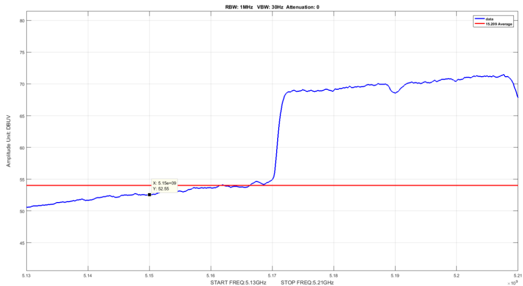
Figure 17: Band Edge BW 80M Ch 5210M 802.11ac Average
