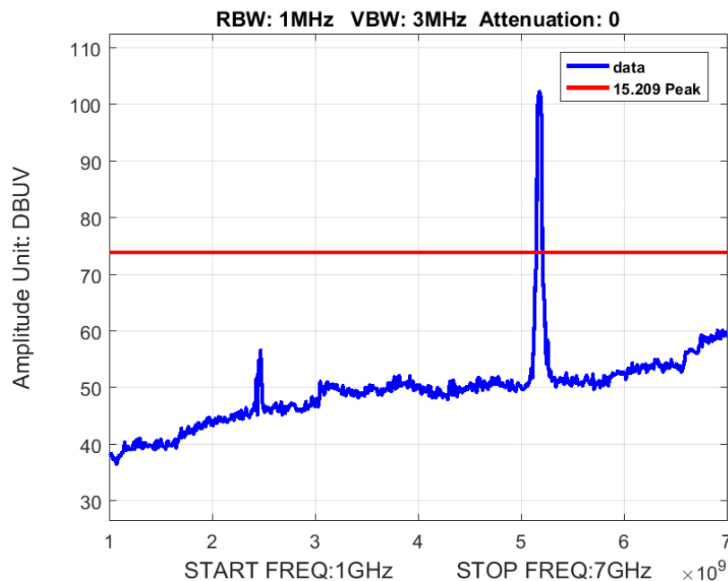
Figure 2: Radiated Spurious Emissions 1-7GHz BW 20M Ch 5180M 802.11a Peak
