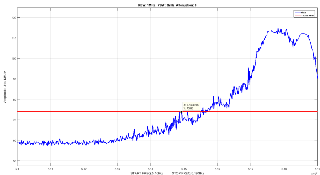
Figure 12: Band Edge BW 20M Ch 5180M 802.11a Peak
