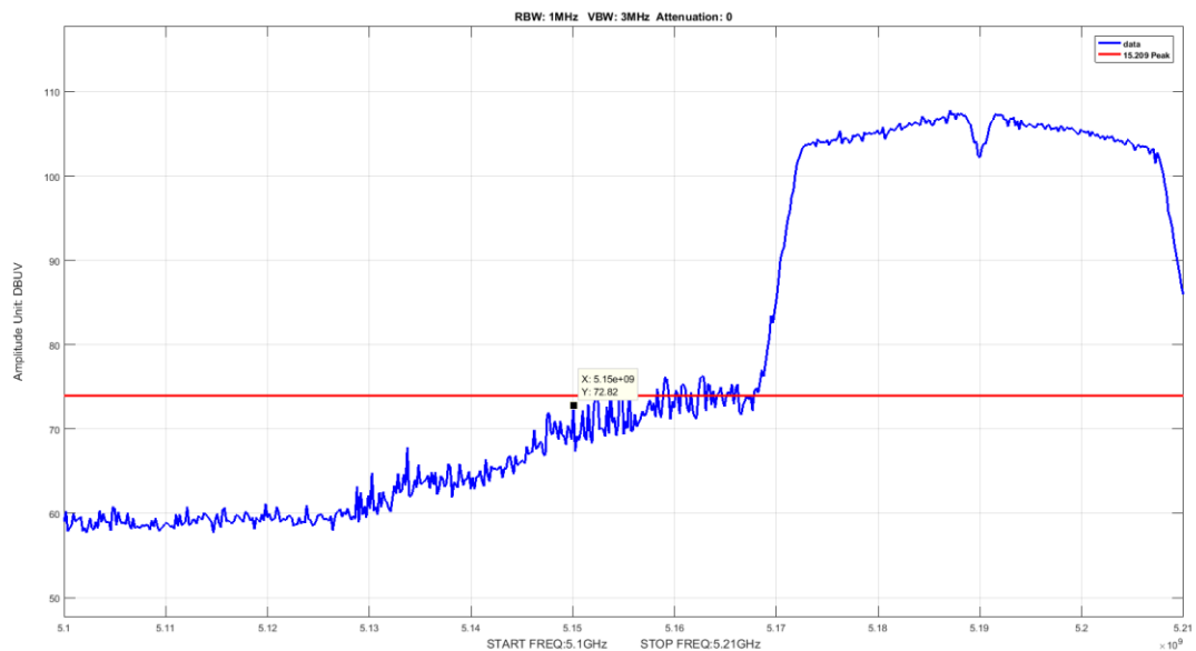
Figure 16: Band Edge BW 40M Ch 5190M 802.11n Peak
