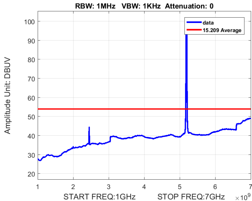
Figure 5: Radiated Spurious Emissions 1-7GHz BW 40M Ch 5190M 802.11n Average
