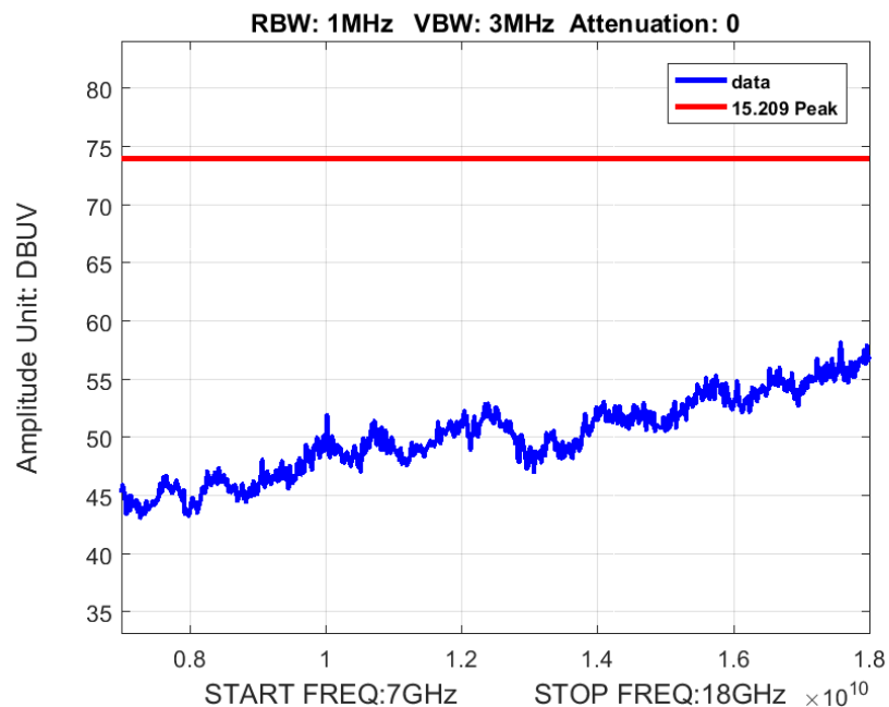
Figure 10: Radiated Spurious Emissions 7-18GHz Worst Case Peak
