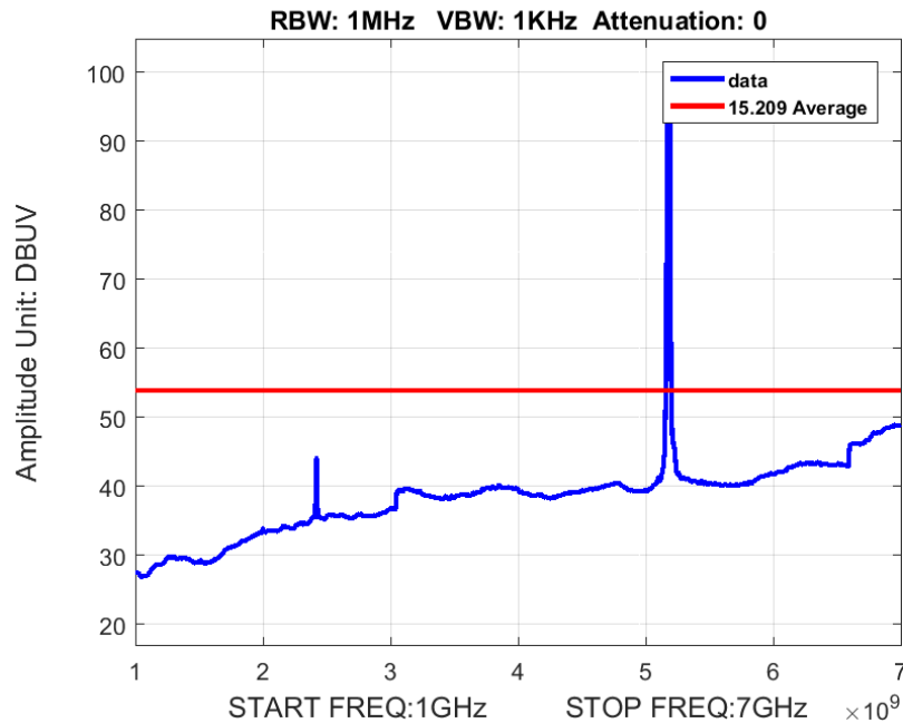
Figure 3: Radiated Spurious Emissions 1-7GHz BW 20M Ch 5180M 802.11n Average
