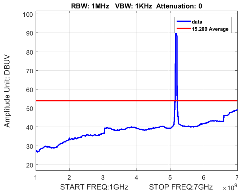
Figure 1: Radiated Spurious Emissions 1-7GHz BW 20M Ch 5180M 802.11a Average
