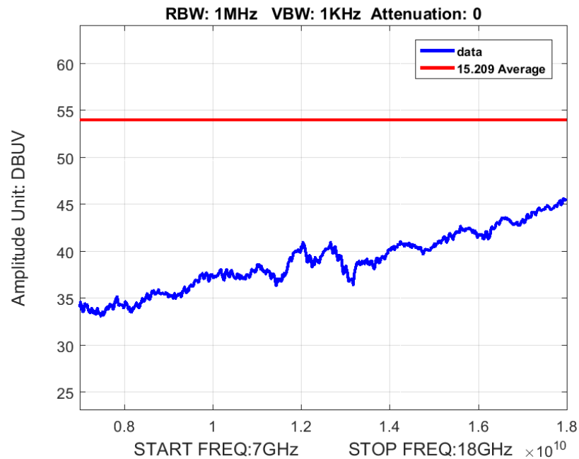
Figure 9: Radiated Spurious Emissions 7-18GHz Worst Case Average
