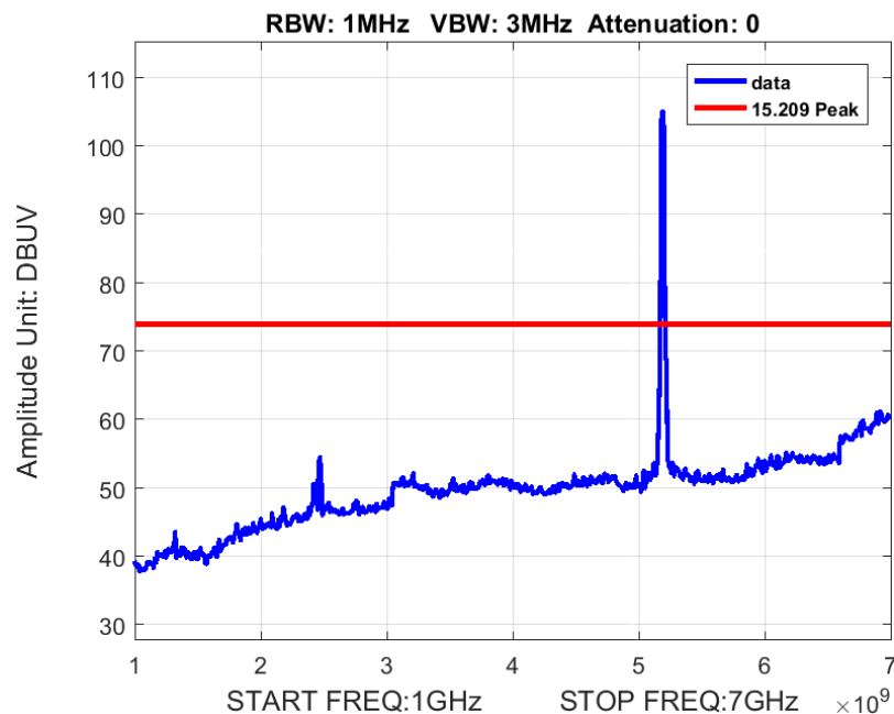
Figure 6: Radiated Spurious Emissions 1-7GHz BW 40M Ch 5190M 802.11n Peak
