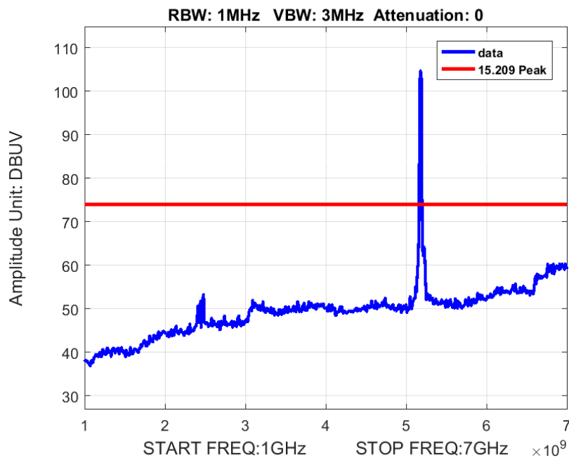
Figure 4: Radiated Spurious Emissions 1-7GHz BW 20M Ch 5180M 802.11n Peak
