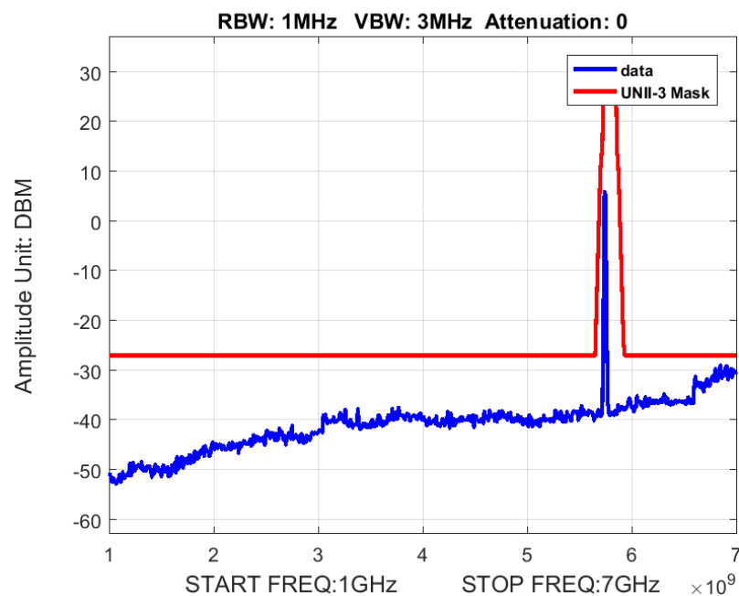
Figure 2: Out of Band Emissions with Mask BW 20M Ch 5745M 80211n
