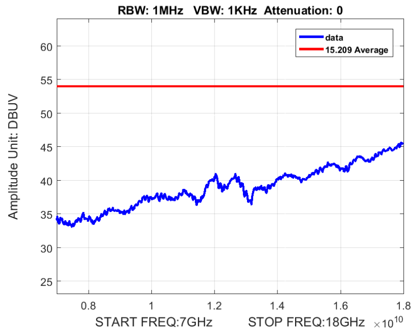
Figure 5: Radiated Spurious Emission 7-18GHz Worst Case Average
