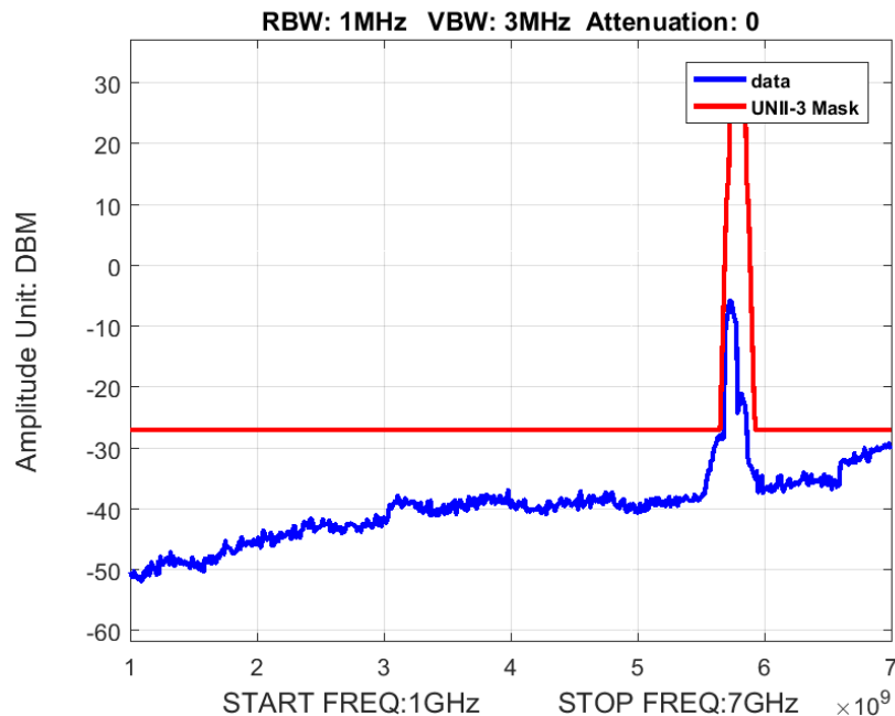
Figure 4: Out of Band Emissions with Mask BW 80M Ch 5775M 80211ac
