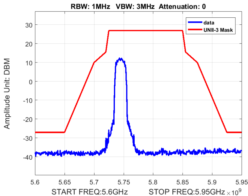
Figure 8: Band Edge Emissions Mask BW 20M Ch 5745M 80211n
