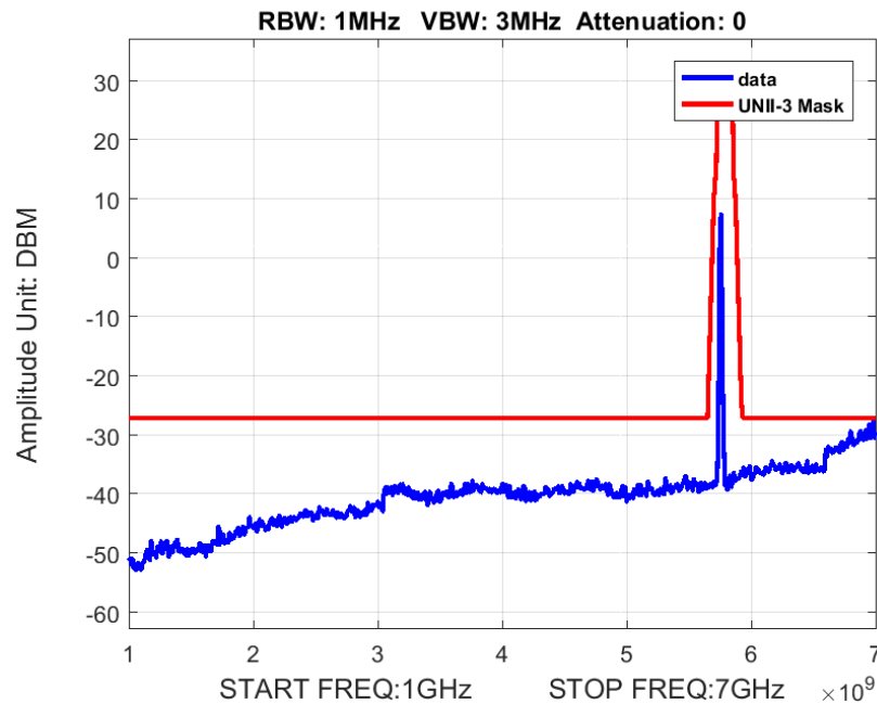
Figure 1: Out of Band Emissions with Mask BW 20M Ch 5745M 80211a
