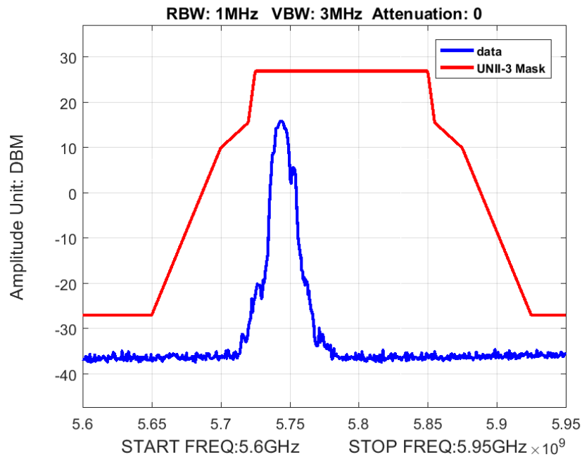
Figure 7: Band Edge Emissions Mask BW 20M Ch 5745M 80211a
