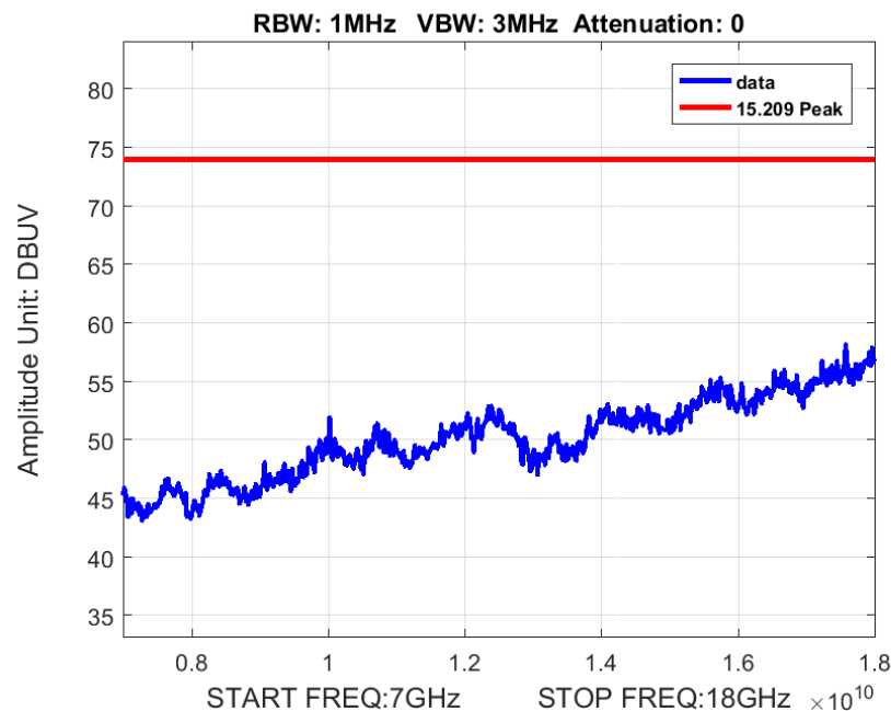
Figure 6: Radiated Spurious Emission 7-18GHz Worst Case Peak
