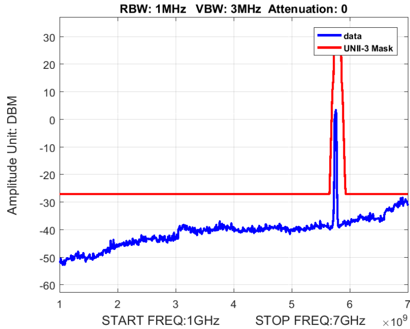
Figure 3: Out of Band Emissions with Mask BW 40M Ch 5755M 80211n
