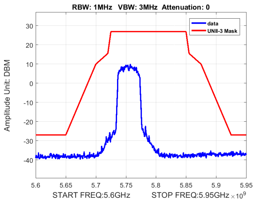
Figure 9: Band Edge Emissions Mask BW 40M Ch 5755M 80211n
