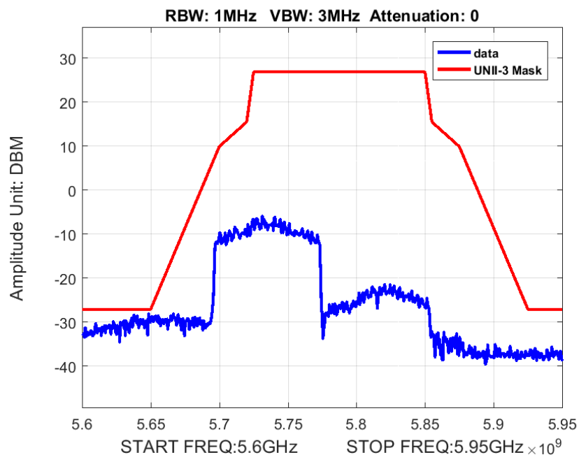
Figure 10: Band Edge Emissions Mask BW 80M Ch 5775M 80211ac
