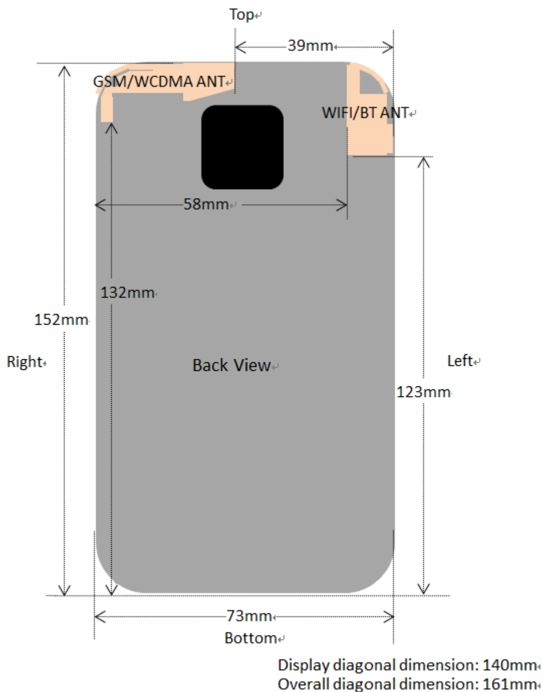
Fig.14.1 EUT Antenna Locations
