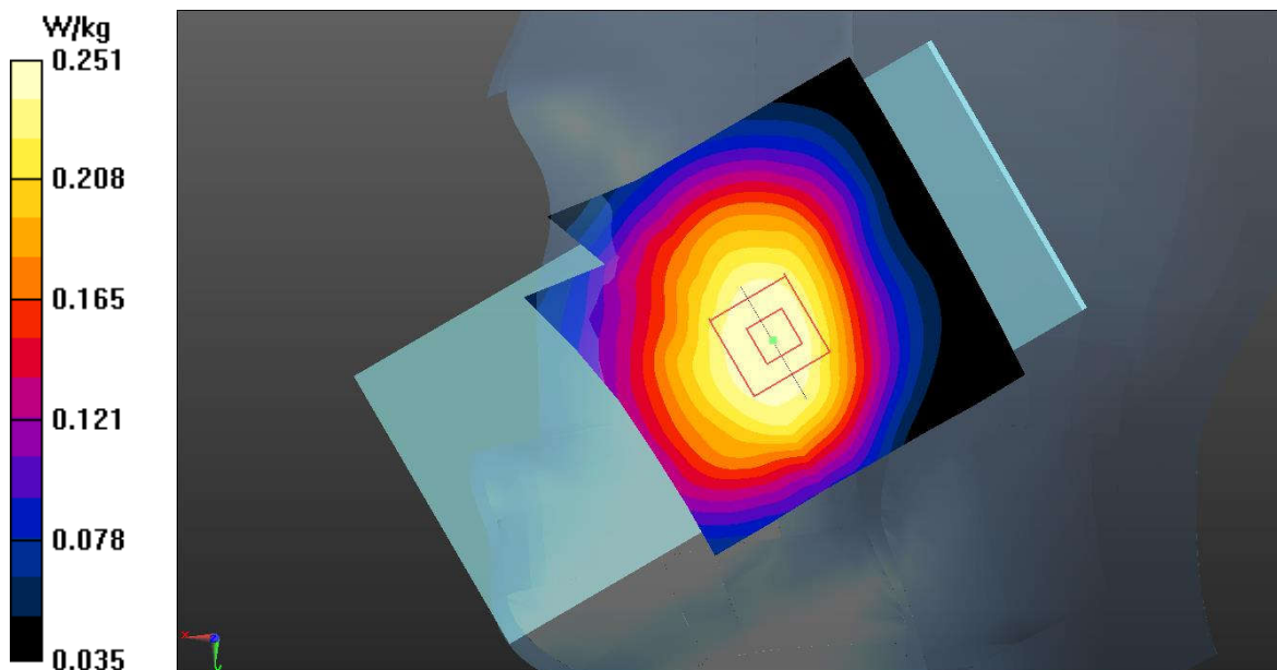
Fig.1 GSM850 Head
