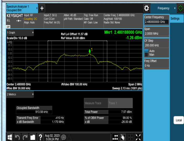
TX-Ant3-2480
