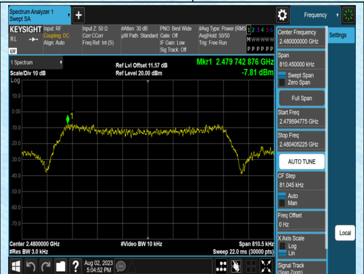
TX-Ant2-2480
