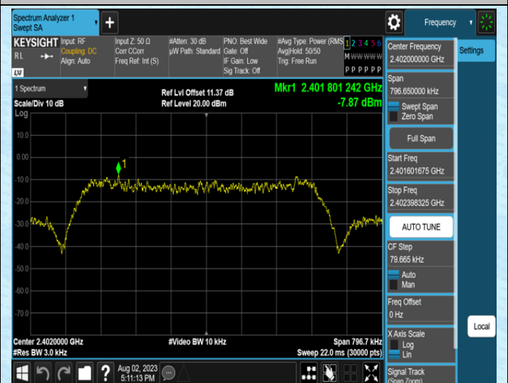
TX-Ant4-2402
