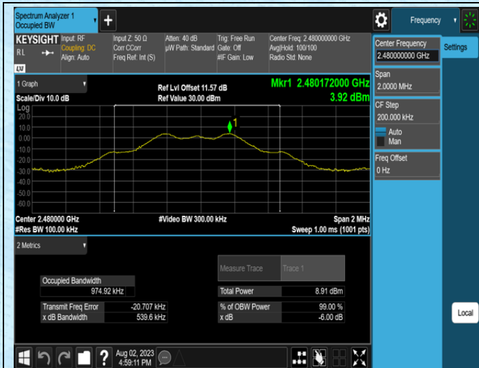
TX-Ant1-2480
