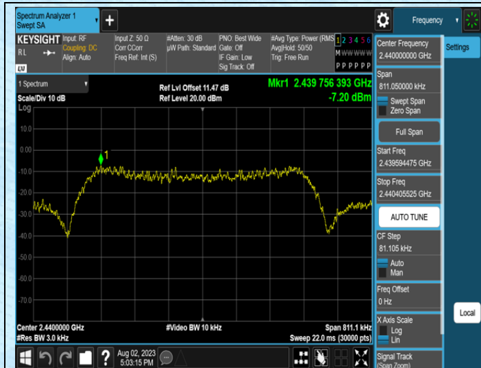
TX-Ant2-2440
