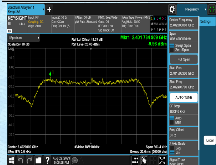
TX-Ant3-2402
