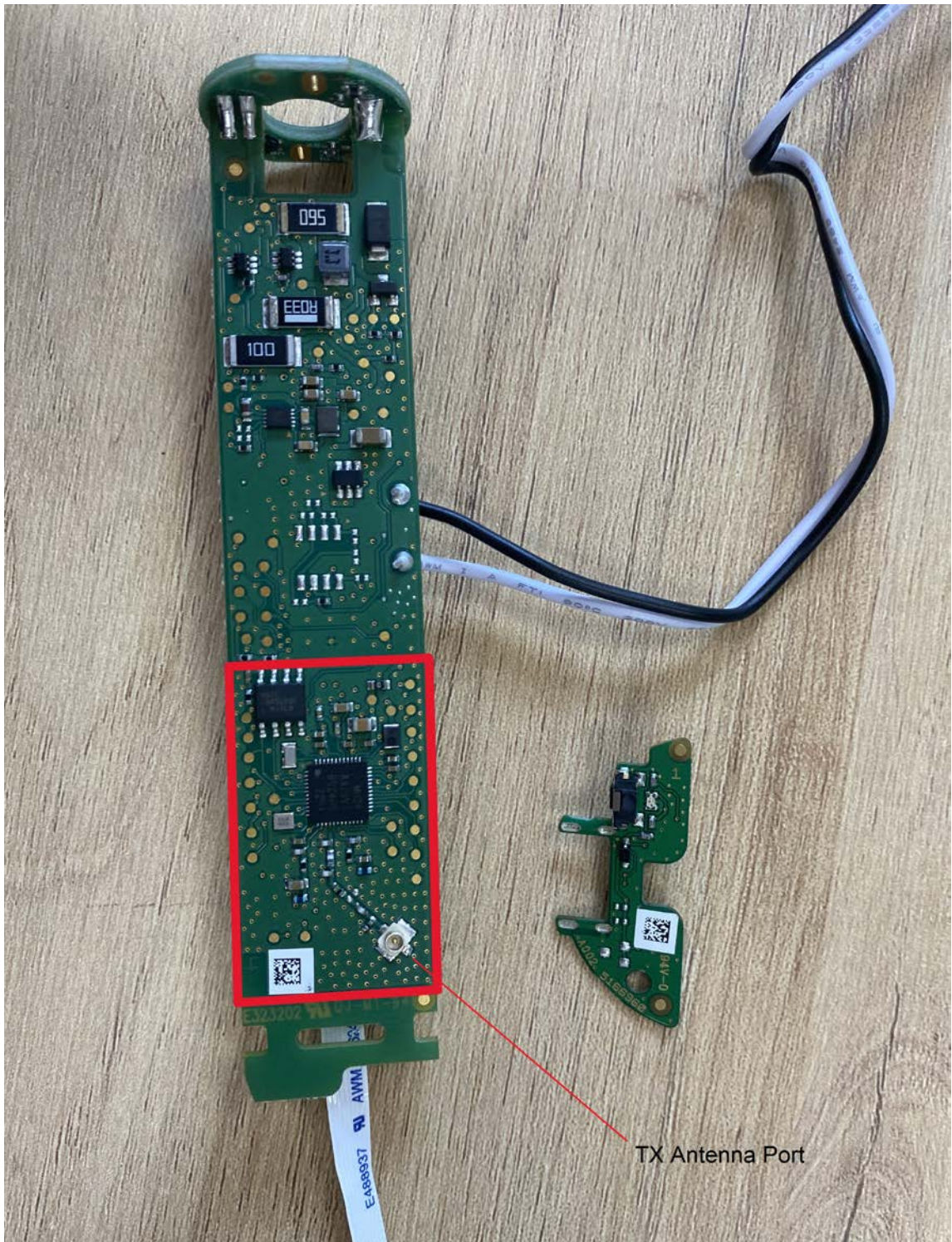
EUT Main PCB Back
