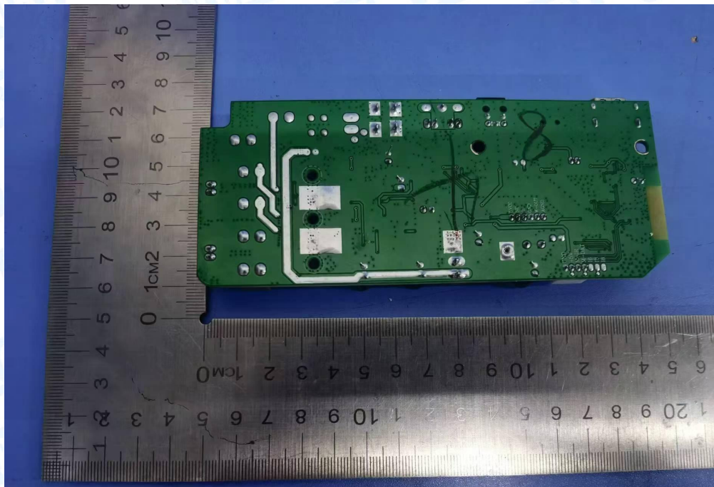
Photo 16 Appearance of PCB
