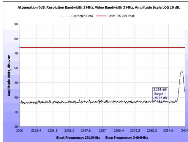
Plot 21. Radiated Restricted Band Edge, 2.402 GHz, Peak - Horizontal
