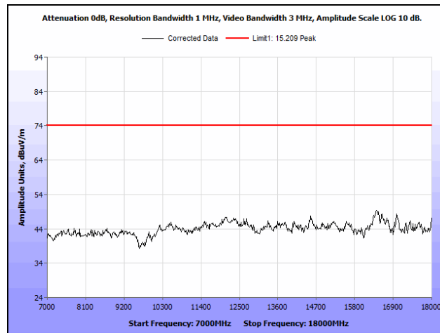
Plot 17. Radiated Spurious Emissions, 7 - 18 GHz, Peak – Horizontal
