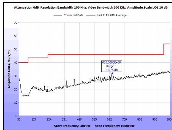
Plot 9. Radiated Spurious Emissions, 30 MHz – 1 GHz - Horizontal
