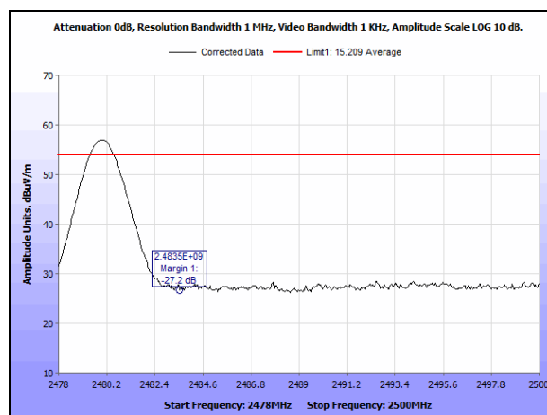
Plot 23. Radiated Restricted Band Edge, 2.480 GHz, Average - Horizontal
