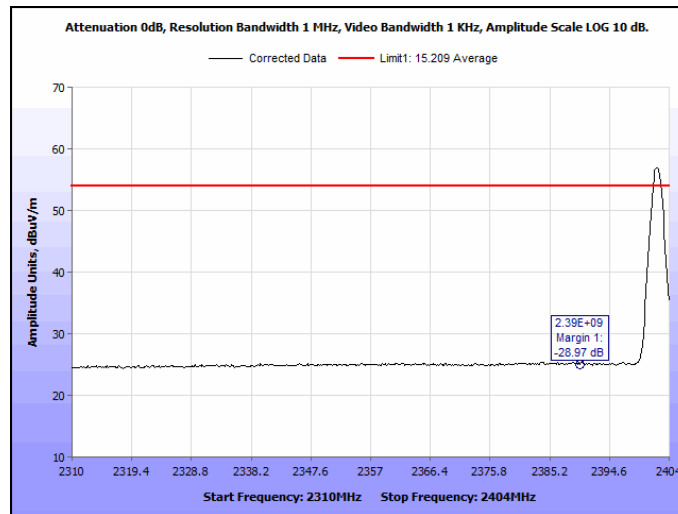
Plot 19. Radiated Restricted Band Edge, 2.402 GHz, Average - Horizontal
