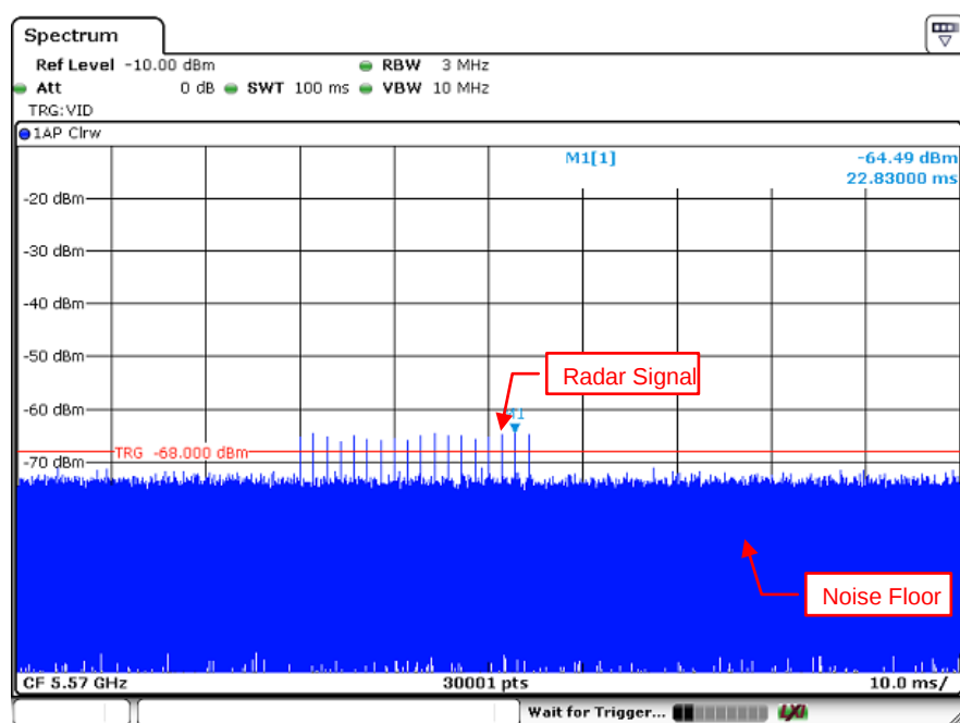
Radar Signal 0
