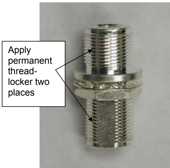
Figure 1. NF-NF bulkhead connector
