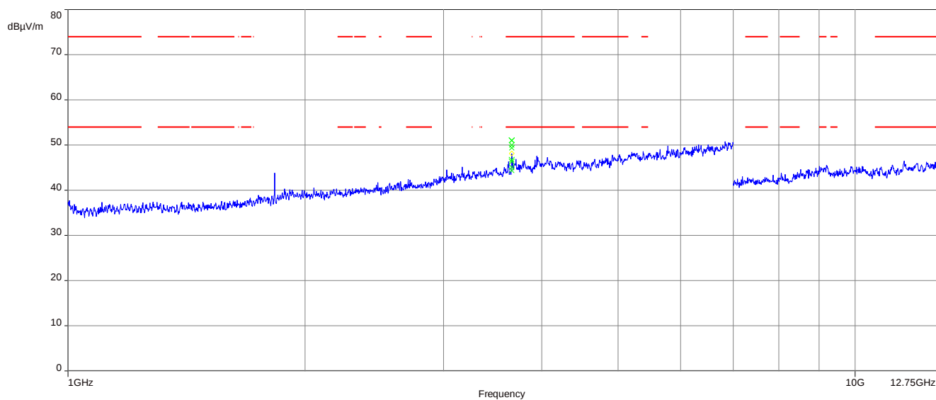
Plot 1: 1 GHz – 12.75 GHz, horizontal & vertical polarisation 915.420 MHz
