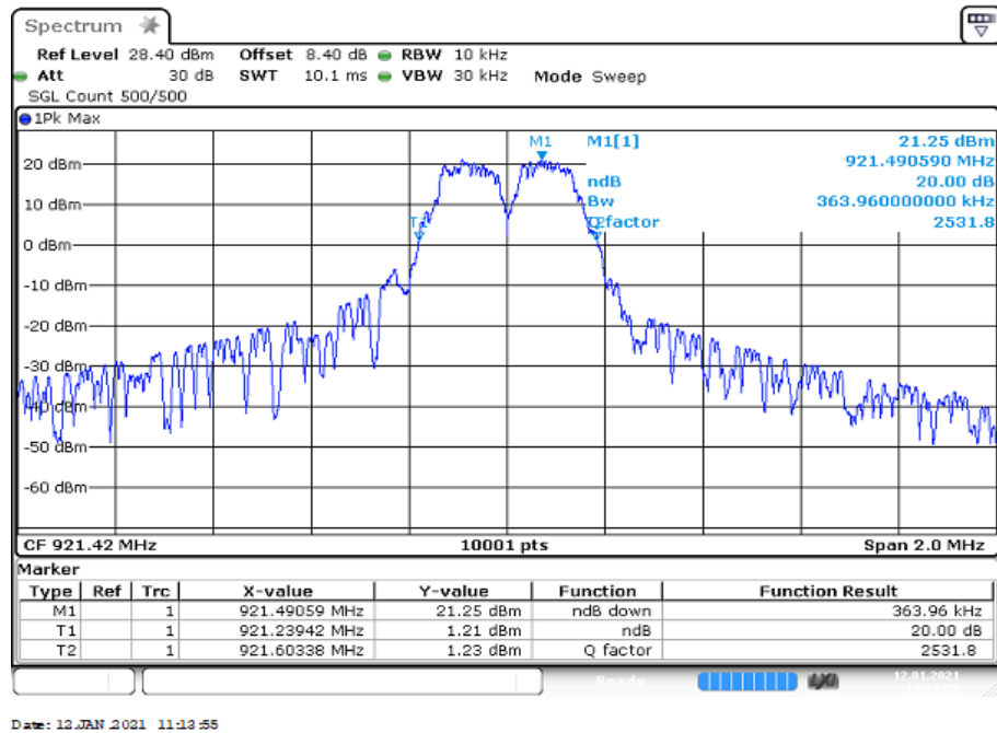
Plot 5: 921.420 MHz, 20 dB-BW
