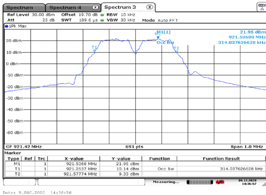
Plot 6: 921.420 MHz, 99%OBW
