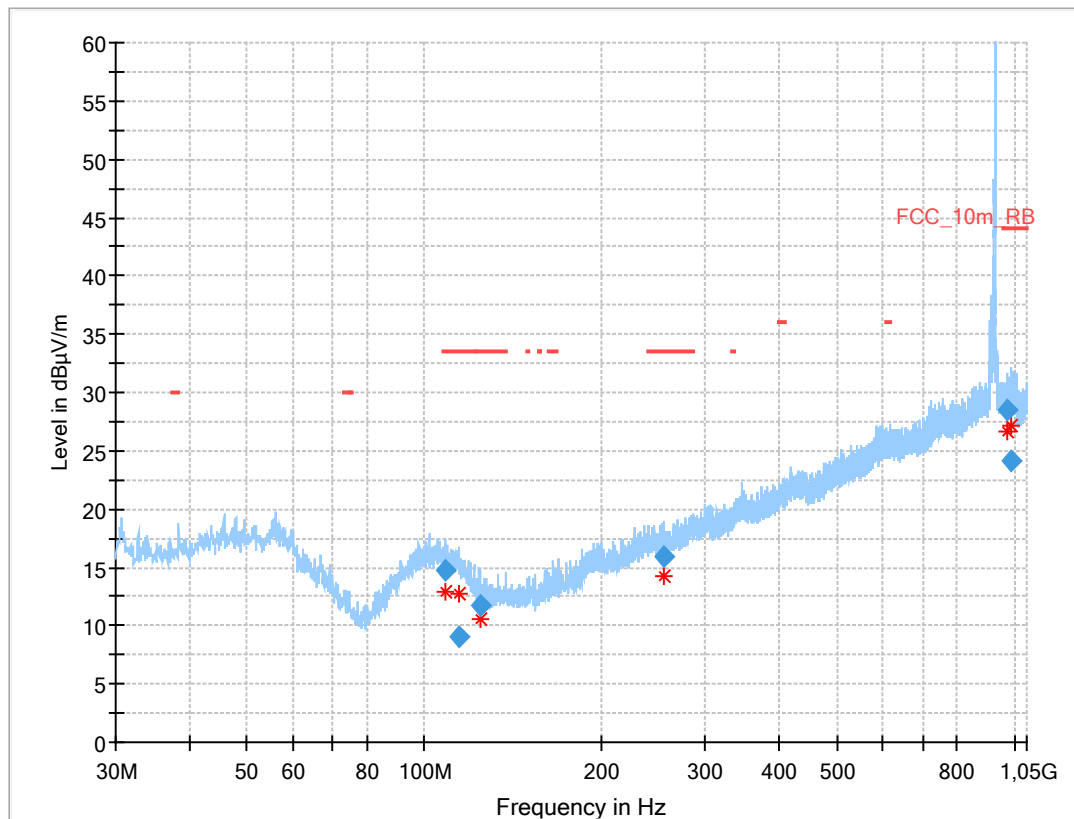
Plot 4: 30 MHz – 1 GHz, horizontal &amp; vertical polarisation 927.42 MHz
