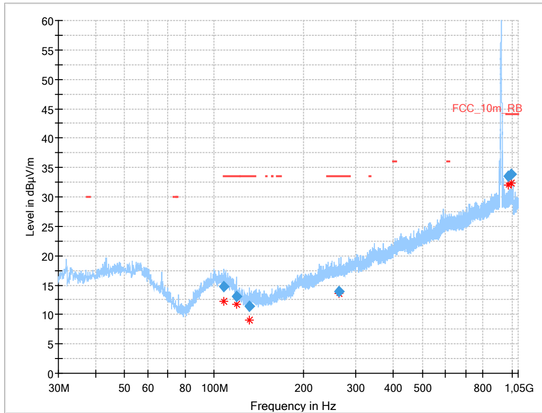
Plot 3: 30 MHz – 1 GHz, horizontal &amp; vertical polarisation 921.420 MHz
