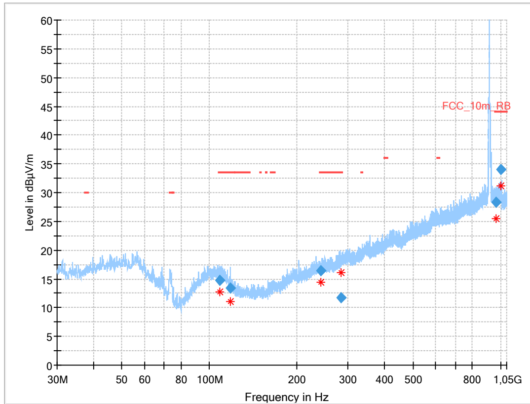
Plot 1: 30 MHz – 1 GHz, horizontal &amp; vertical polarisation 915.420 MHz
