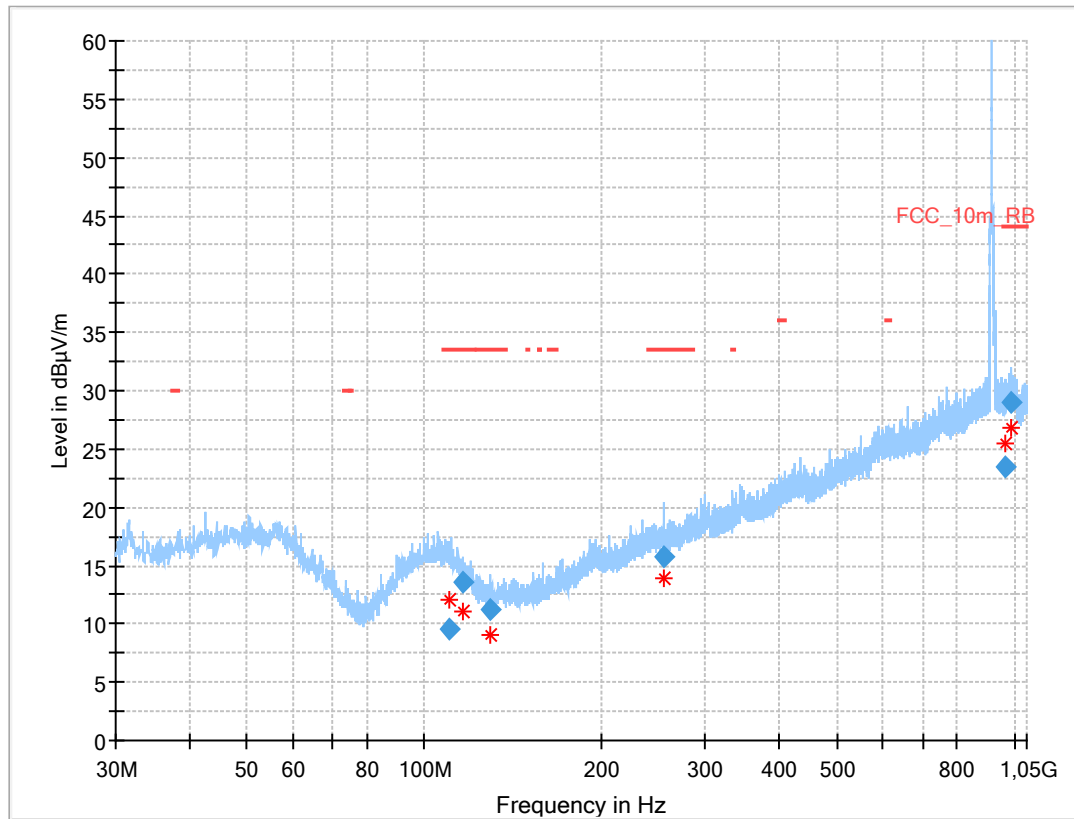
Plot 2: 30 MHz – 1 GHz, horizontal &amp; vertical polarisation 915.795 MHz
