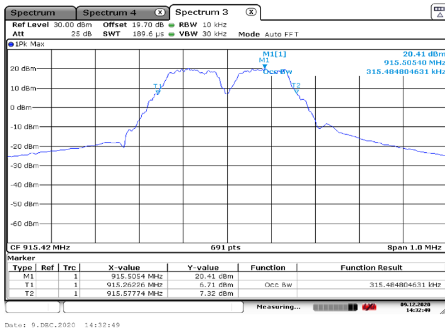
Plot 2: 915.420 MHz, 99%OBW
