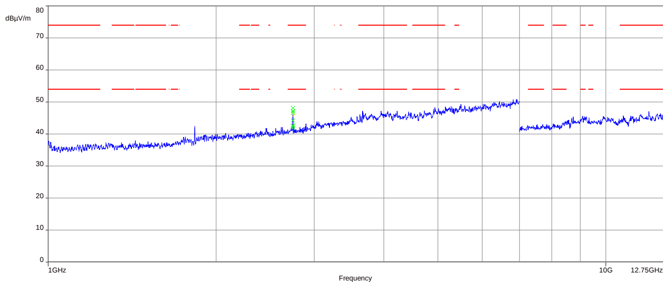
Plot 2: 1 GHz – 12.75 GHz, horizontal & vertical polarisation 915.795 MHz
