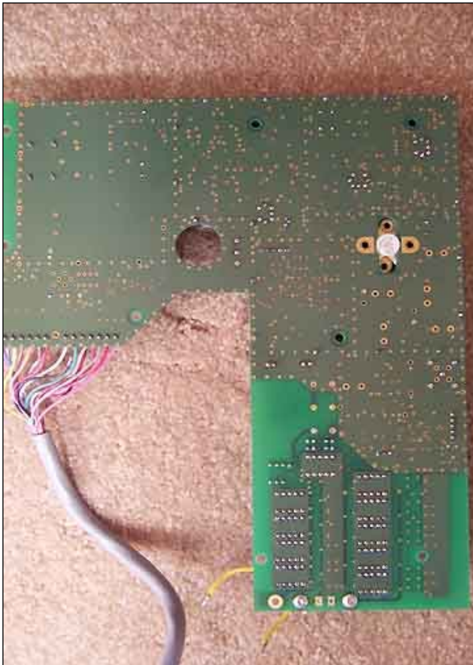
PCB Back
