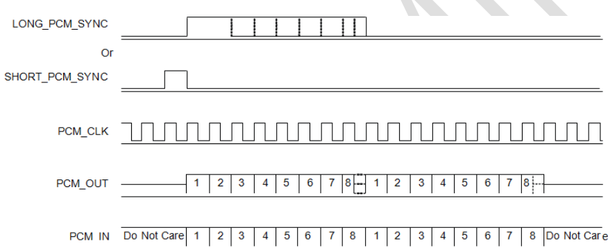
Figure 6: Multi-slot Operation with 2 Slots and 8-bit Companded Samples
