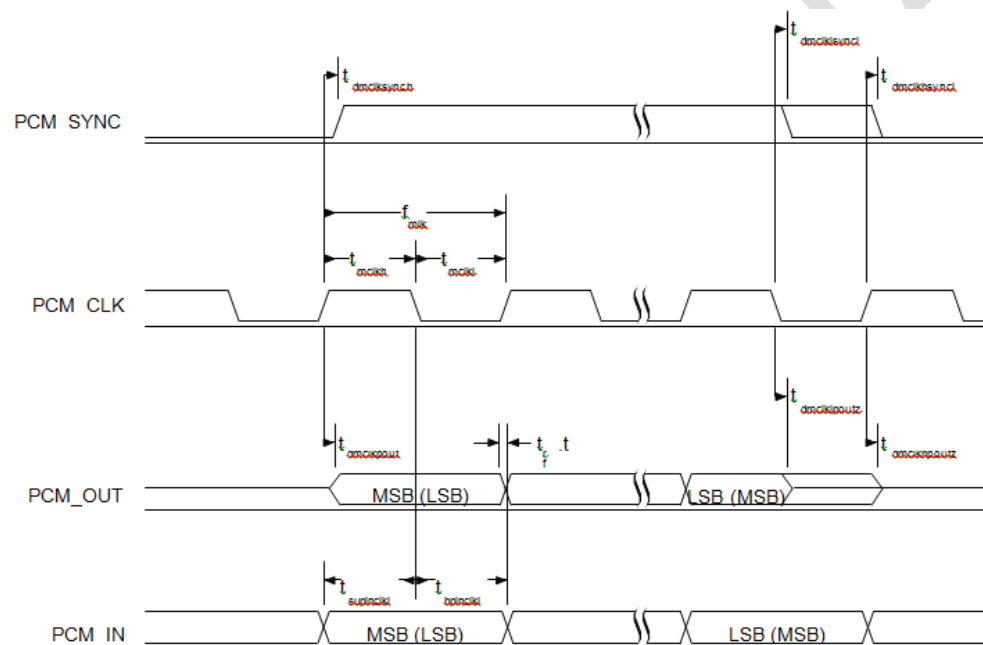
Symbol Parameter Min Typ Max Unit t_{dmclkhsvnd} Delay time from 4MHz DDS generation PCM_CLK high to PCM_SYNC low - - 20 ns 48MHz DDS generation - - 40.83 ns t_{dmclklpoutz} Delay time from PCM_CLK low to PCM_OUT high impedance - - 20 ns t_{dmclkhputz} Delay time from PCM_CLK high to PCM_OUT high impedance - - 20 ns t_{suninckl} Set-up time for PCM_IN valid to PCM_CLK low 20 - - ns t_{hpinckl} Hold time for PCM_CLK low to PCM_IN invalid 0 - - ns
