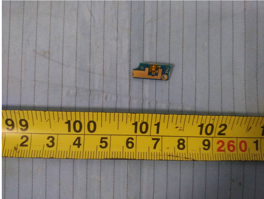
EUT – Antenna Match Board Bottom View
