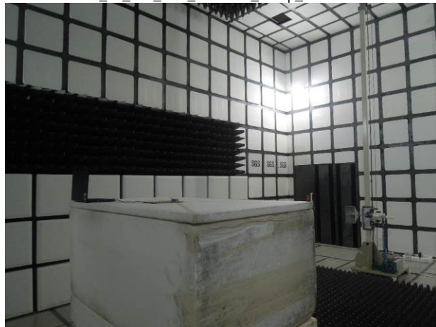
FCC_15_247_BLE_Radiated_Setup_2nd Source
