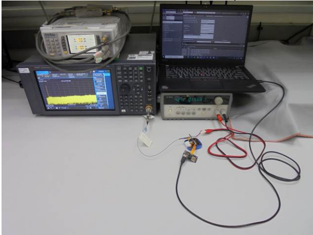
FCC 15 247 WLAN Conducted setup
