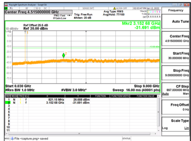
Band26Part90 / 3MHz / High CH / 64QAM
