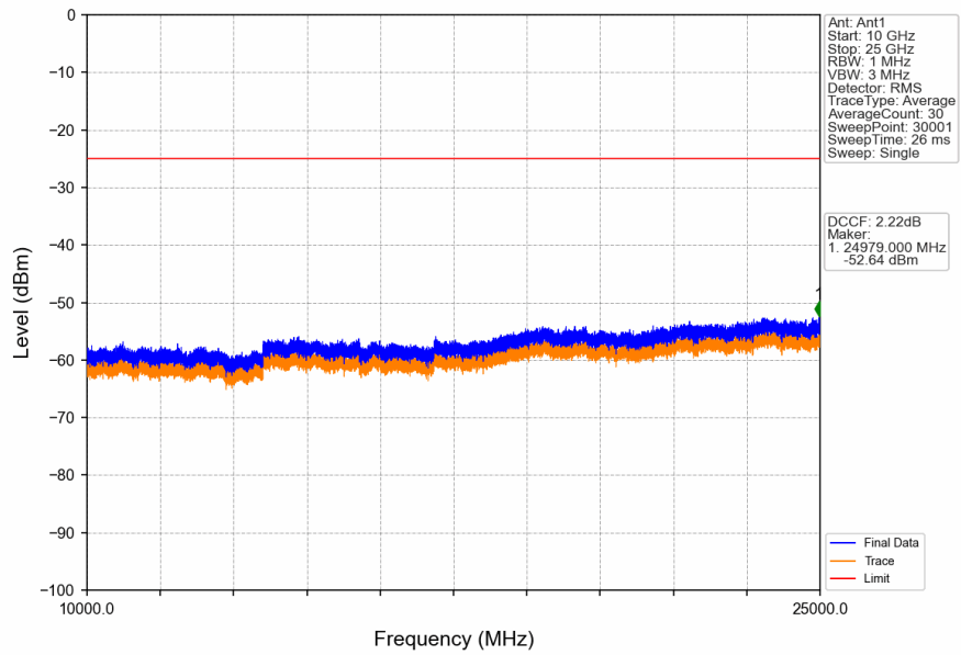
Band41_5MHz_16QAM_MCH_2593MHz_RB_1_0_NTNV
