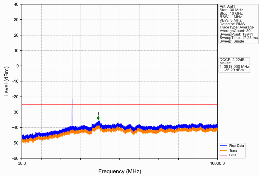
Band41_5MHz_16QAM_MCH_2593MHz_RB_1_0_NTNV
