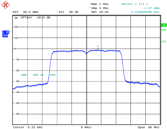
802.11ax40_5230MHz_RU_Full_Chain 0
