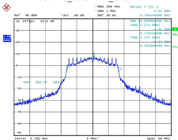
802.11a_5785MHz_Chain 0
