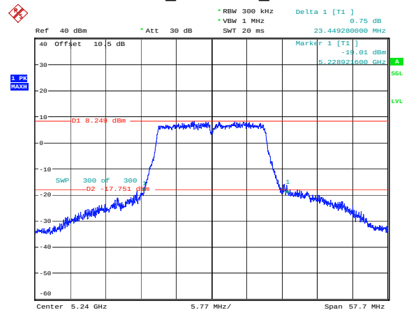
802.11n20_5240MHz_Chain 0
