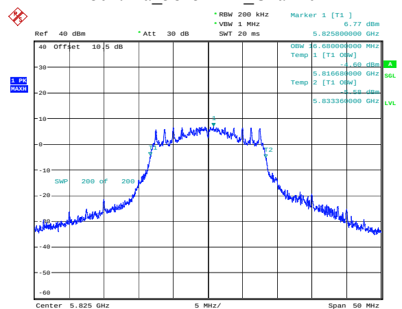
802.11a_5825MHz_Chain 0
