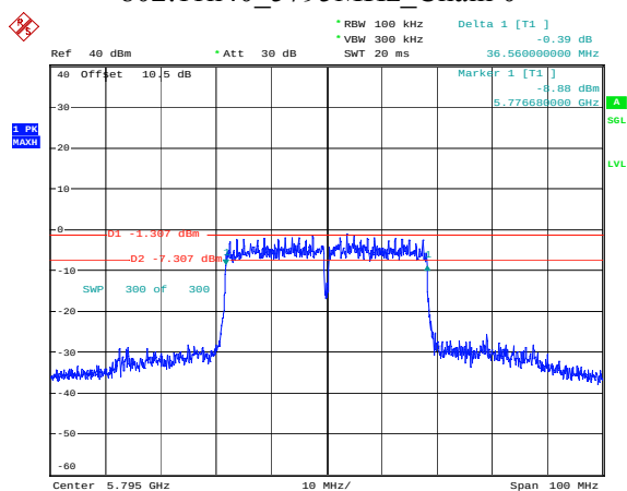
802.11n40_5795MHz_Chain 0
