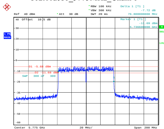
802.11ac80_5775MHz_Chain 0
