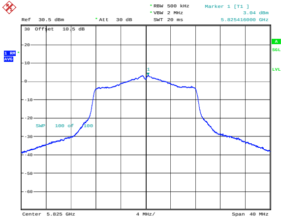
802.11a_5825MHz_Chain 0
