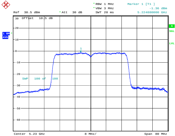
802.11ax40_5230MHz_RU_Full_Chain 1
