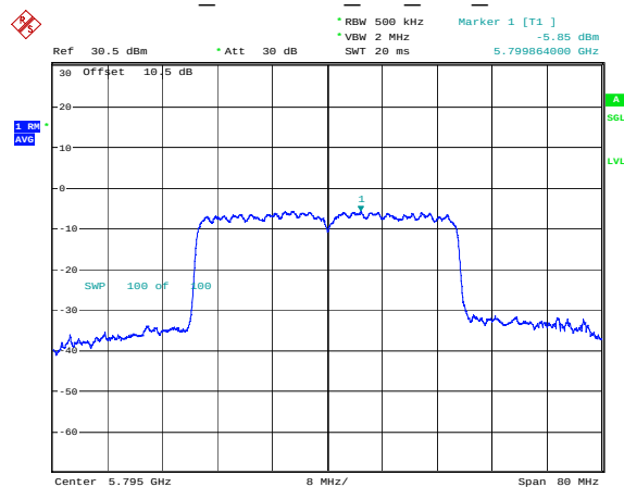
802.11ax40 5795MHz RU Full Chain 1
