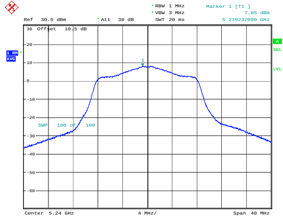
802.11a_5240MHz_Chain 0
