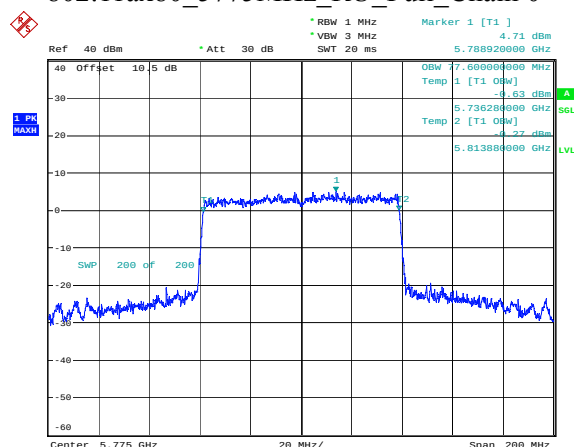
802.11ax80_5775MHz_RU_Full_Chain 0
