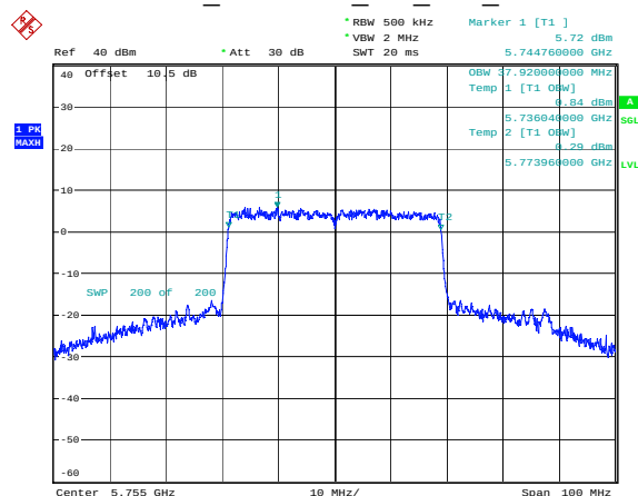
802.11ax40_5755MHz_RU_Full_Chain 0
