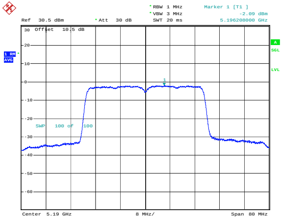
802.11ax40_5190MHz_RU_Full_Chain 0
