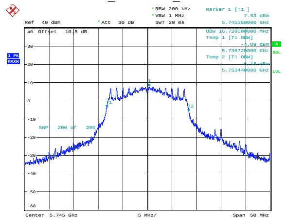
802.11a_5745MHz_Chain 0
