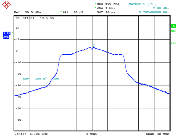
802.11a_5785MHz_Chain 0
