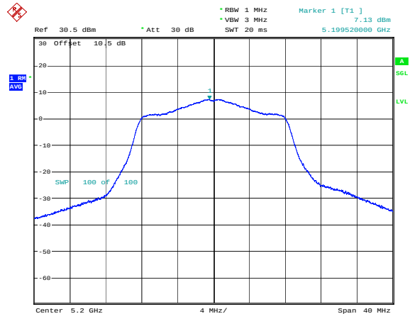
802.11a_5200MHz_Chain 1
