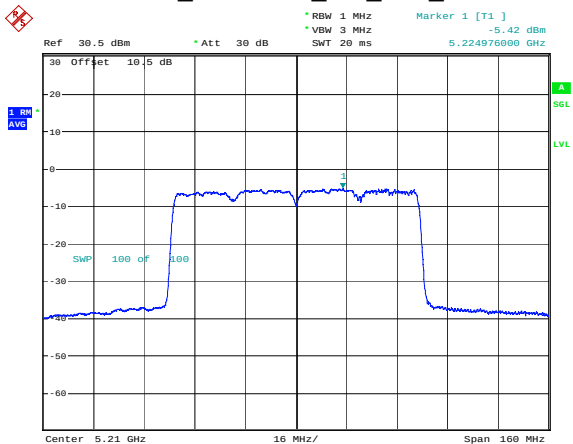
802.11ax80_5210MHz_RU_Full_Chain 0
