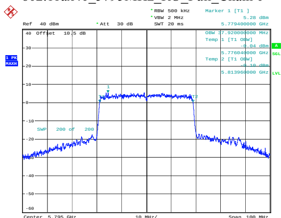
802.11ax40_5795MHz_RU_Full_Chain 0
