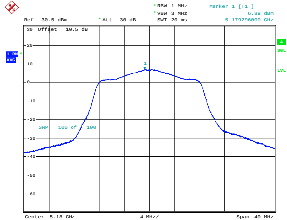
802.11a_5180MHz_Chain 0
