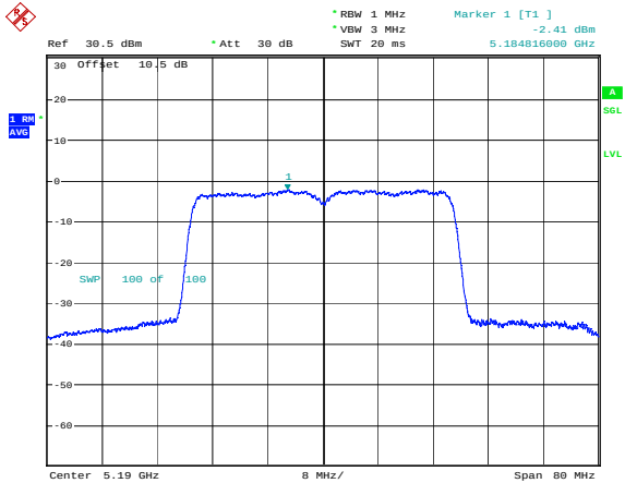
802.11ax40_5190MHz_RU_Full_Chain 1
