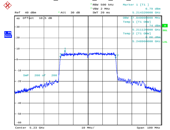
802.11ax40_5230MHz_RU_Full_Chain 0
