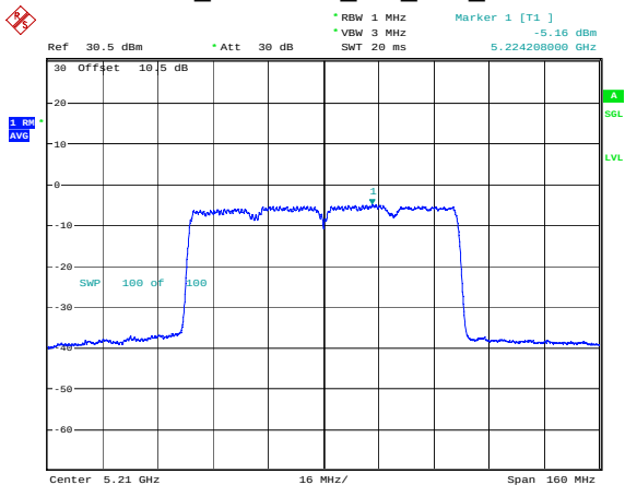
802.11ax80_5210MHz_RU_Full_Chain 1
