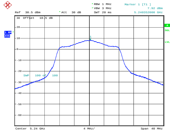
802.11a_5240MHz_Chain 1
