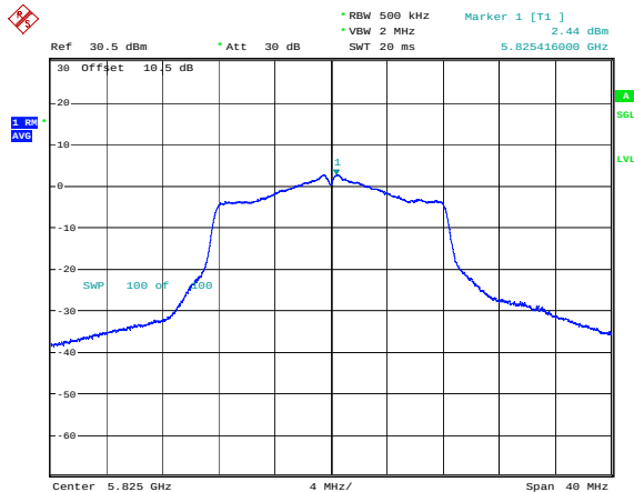
802.11a_5825MHz_Chain 1
