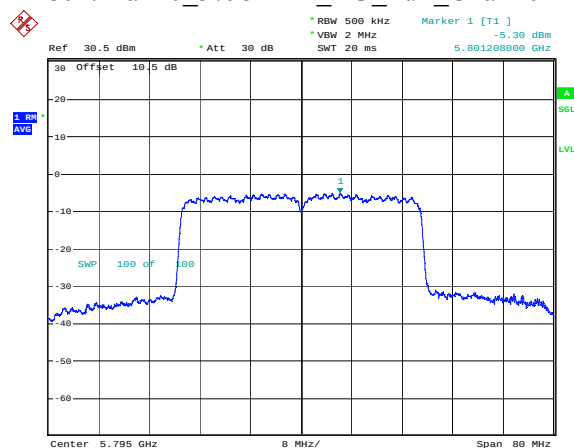
802.11ax40 5795MHz RU Full Chain 0
