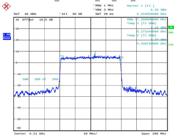
802.11ax80_5210MHz_RU_Full_Chain 0
