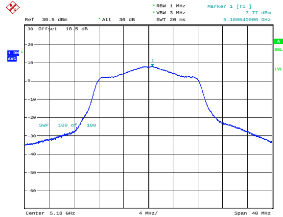
802.11a_5180MHz_Chain 1
