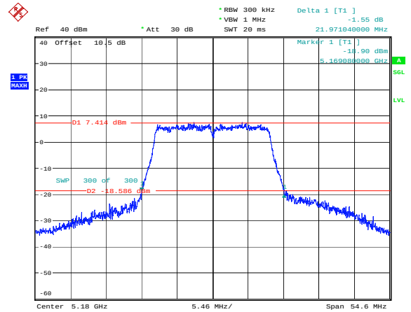
802.11n20_5180MHz_Chain 0
