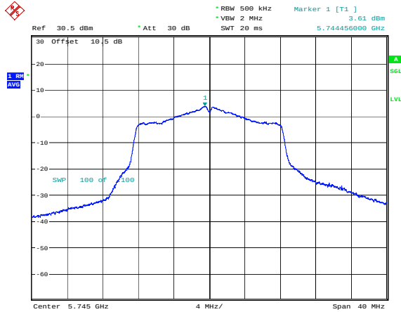
802.11a_5745MHz_Chain 1
