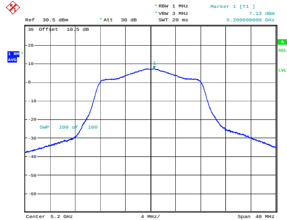
802.11a_5200MHz_Chain 0
