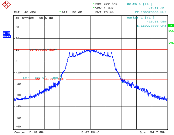
802.11a_5180MHz_Chain 0
