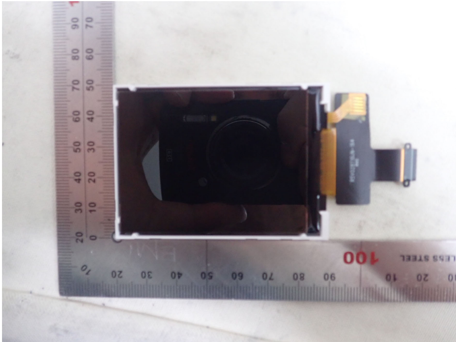
LCD Front
