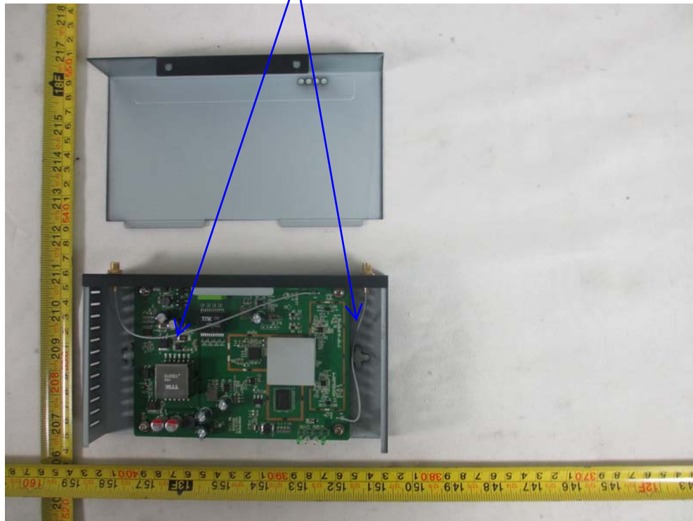
dipole antenna
