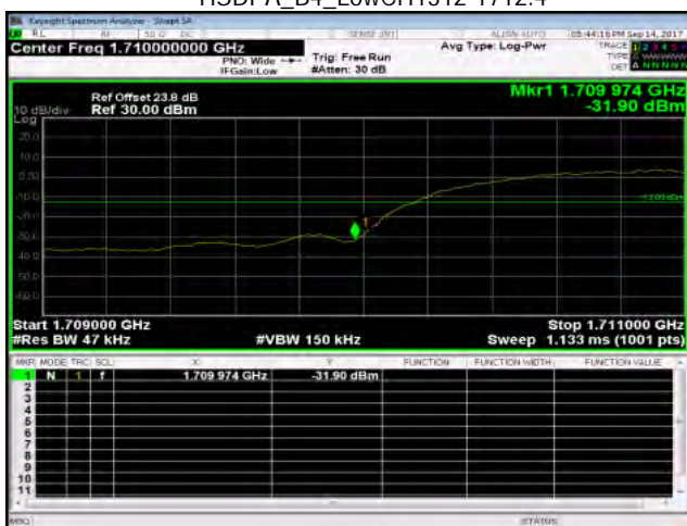
HSDPA_B4_LowCH1312-1712.4
