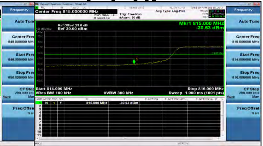
Band26_10MHz_QPSK_50_0_LowCH26750-820
