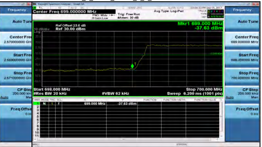
Band12_1_4MHz_QPSK_6_0_LowCH23017-699.7
