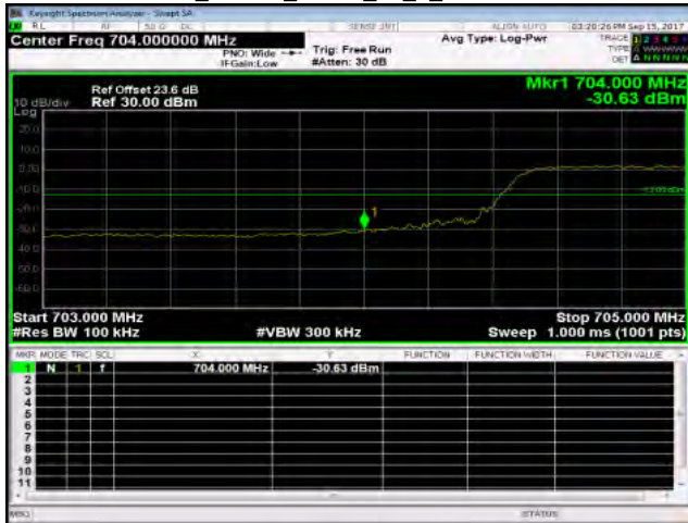
Band17_10MHz_QPSK_50_0_LowCH23780-709
