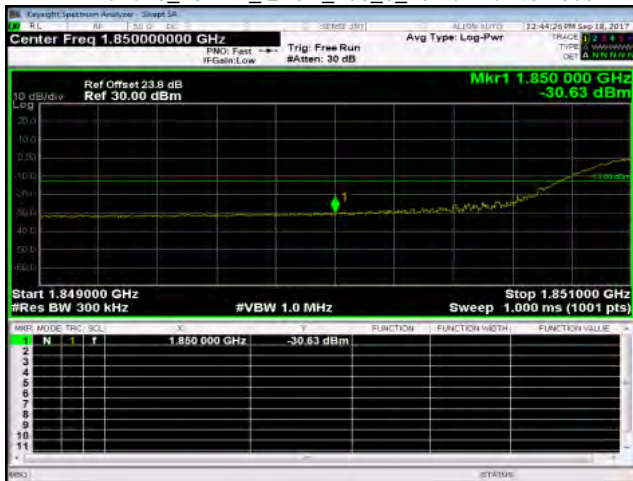
Band25_20MHz_QPSK_100_0_LowCH26140-1860
