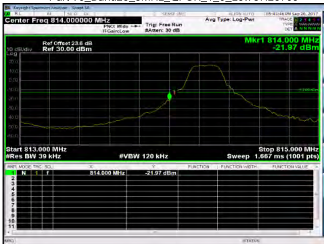
Part 90_Band26_3MHz_QPSK_1_0_LowCH26705
