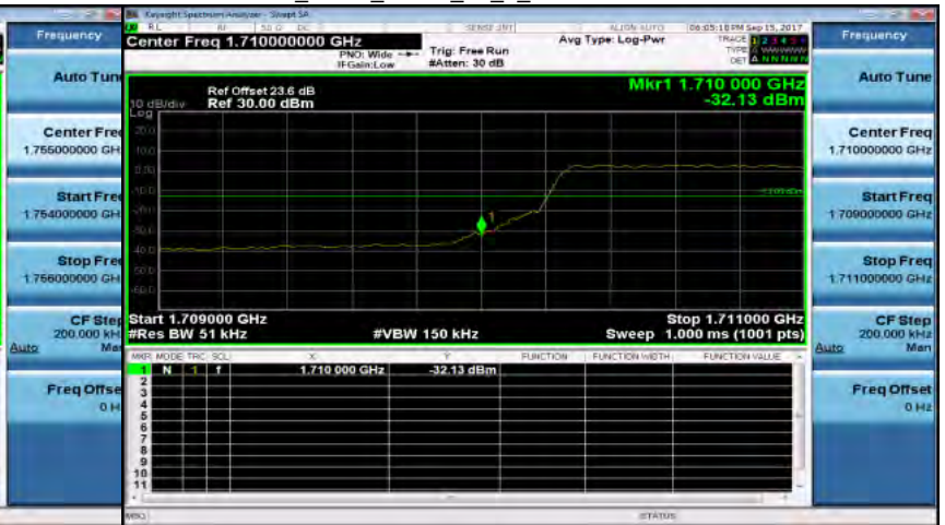
Band4_5MHz_QPSK_25_0_LowCH19975-1712.5
