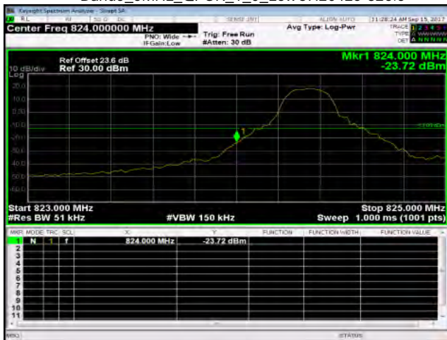
Band5_5MHz_QPSK_1_0_LowCH20425-826.5
