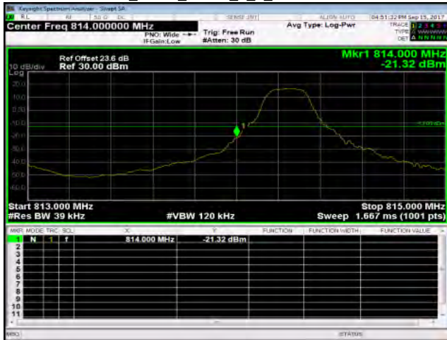
Band26_3MHz_QPSK_1_0_LowCH26705-815.5
