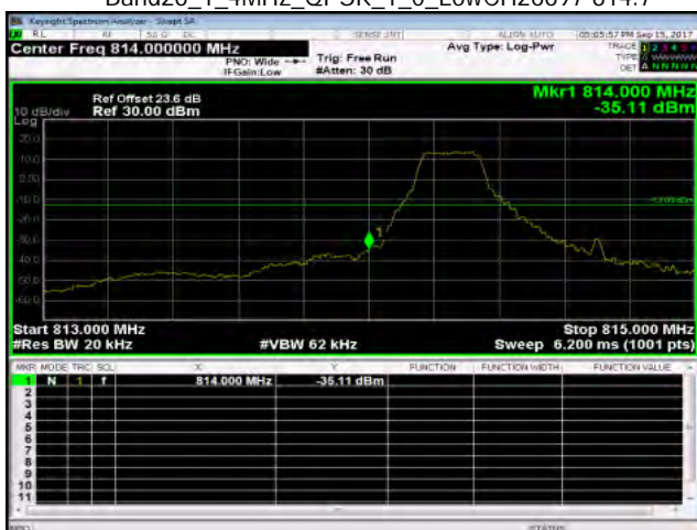
Band26_1_4MHz_QPSK_1_0_LowCH26697-814.7
