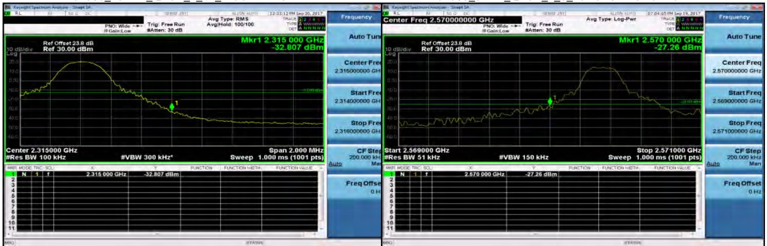
Band30_10MHz_QPSK_1_49_MidCH27710
