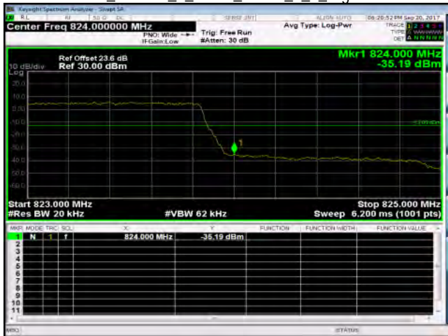
Part 90_Band26_1_4MHz_QPSK_6_0_HighCH26783
