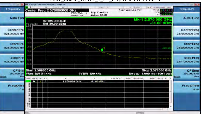
Band7_5MHz_QPSK_1_24_HighCH21425-2567.5
