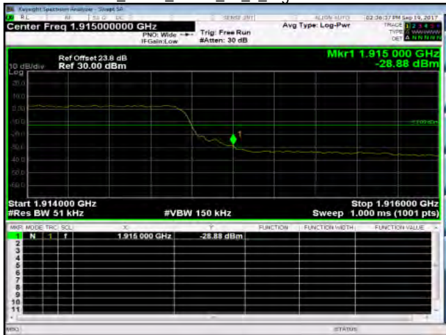
Band25_5MHz_QPSK_25_0_HighCH26665-1912.5
