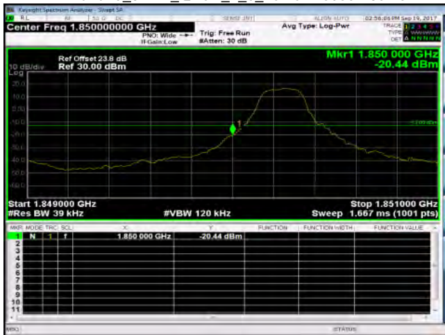
Band25_3MHz_QPSK_1_0_LowCH26055-1851.5
