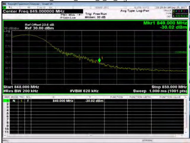
Band26_15MHz_QPSK_1_74_HighCH26965-841.5
