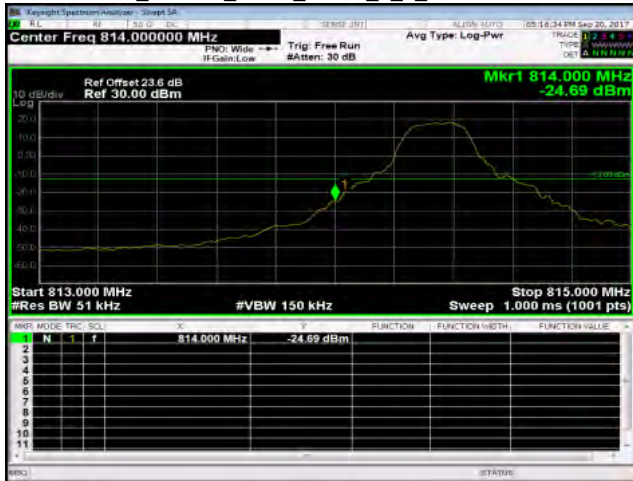
Part 90_Band26_5MHz_QPSK_1_0_LowCH26715-816.5
