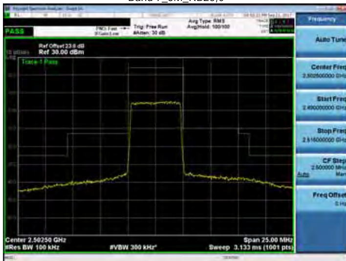
Band 7_5M_RB25,0
