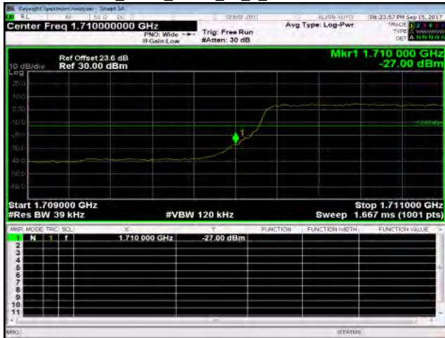
Band4_3MHz_QPSK_15_0_LowCH19965-1711.5
