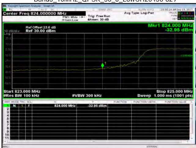
Band5_10MHz_QPSK_50_0_LowCH20450-829
