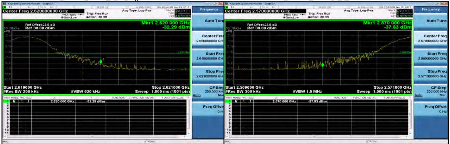
Band38_15MHz_QPSK_1_74_HighCH38175
