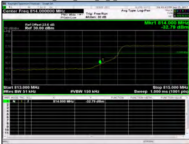
Band26_5MHz_QPSK_25_0_LowCH26715-816.5
