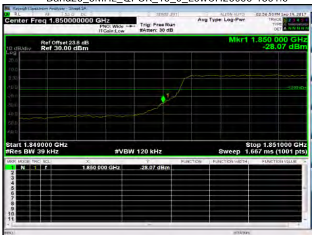
Band25_3MHz_QPSK_15_0_LowCH26055-1851.5
