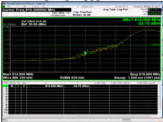
Band26_15MHz_QPSK_1_0_LowCH26775-822.5
