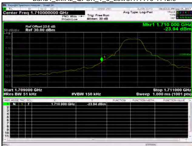
Band4_5MHz_QPSK_1_0_LowCH19975-1712.5
