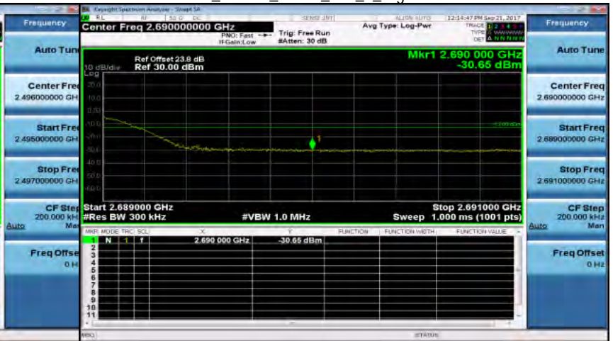
Band41_20MHz_QPSK_100_0_HighCH41490
