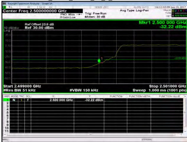
Band7_5MHz_QPSK_25_0_LowCH20775-2502.5
