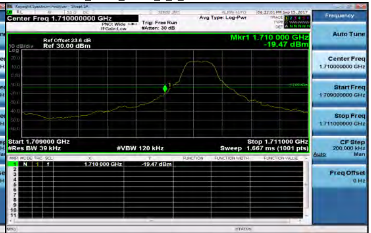
Band4_3MHz_QPSK_1_0_LowCH19965-1711.5
