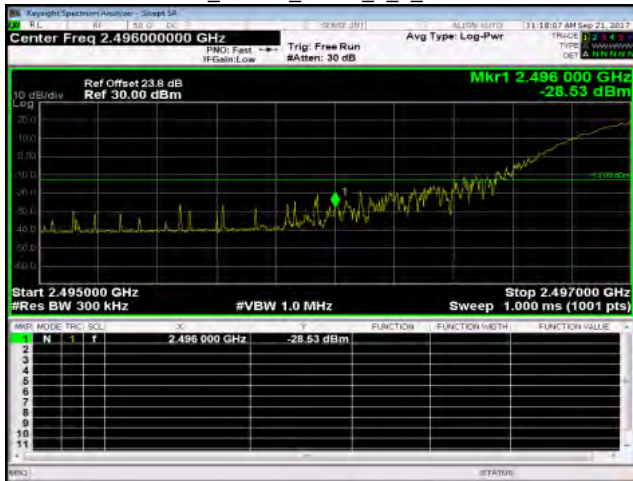
Band41_20MHz_QPSK_1_0_LowCH39750
