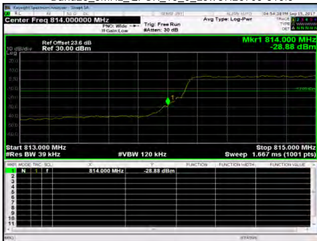
Band26_3MHz_QPSK_15_0_LowCH26705-815.5
