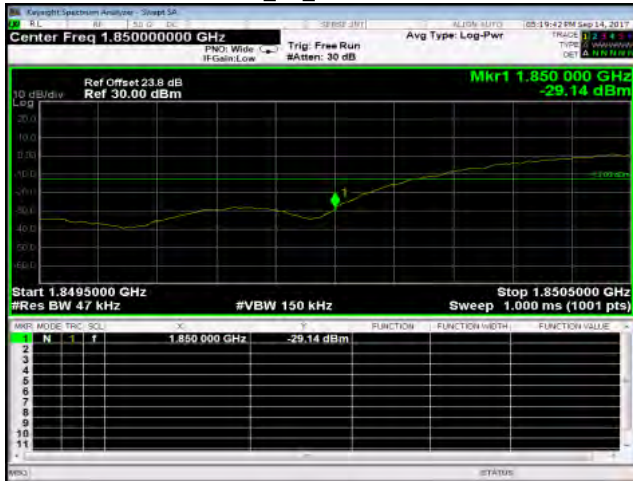
WCDMA_B2_LowCH9262-1852.4
