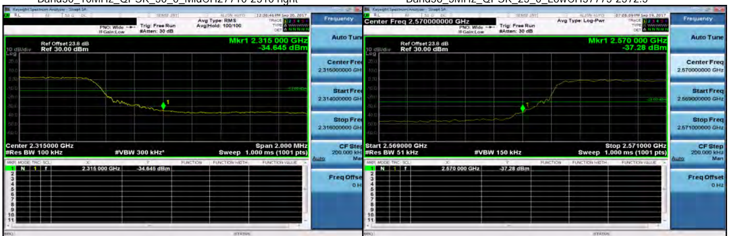
Band30_10MHz_QPSK_50_0_MidCH27710-2310 right
