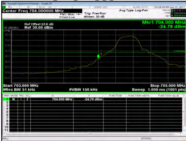
Band17_5MHz_QPSK_1_0_LowCH23755-706.5
