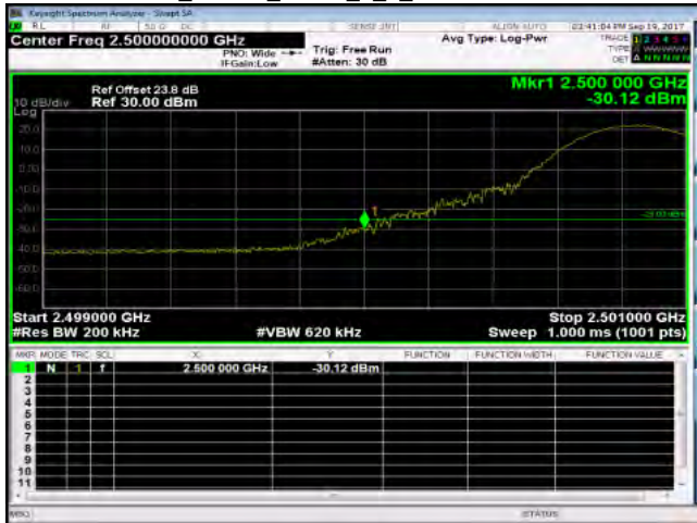
Band7_15MHz_QPSK_1_0_LowCH20825-2507.5
