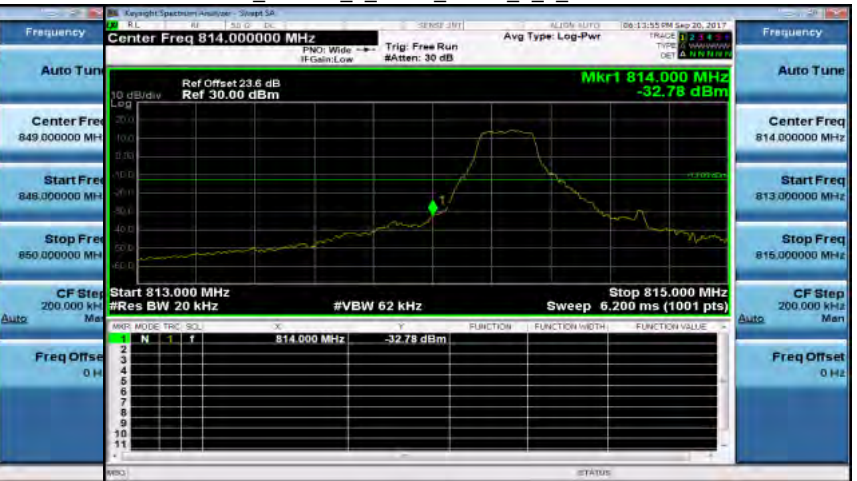
Part 90_Band26_1_4MHz_QPSK_1_0_LowCH26697
