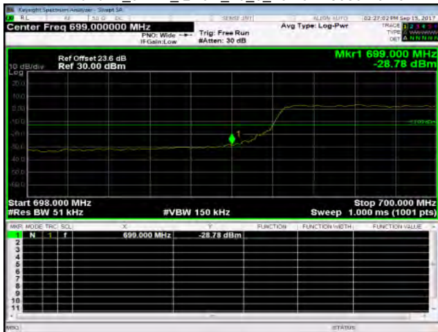
Band12_5MHz_QPSK_25_0_LowCH23035-701.5
