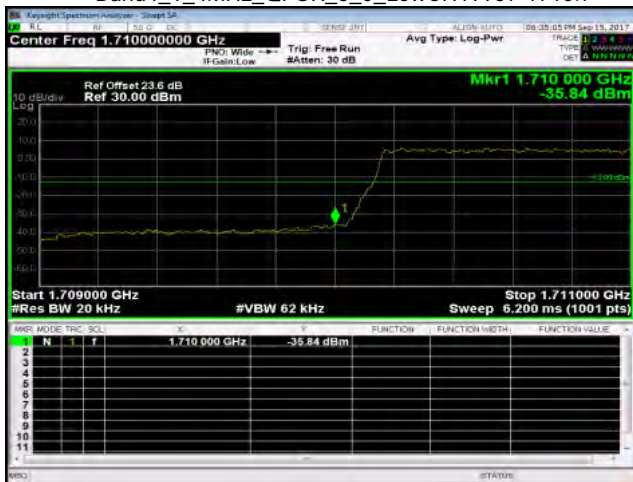
Band4_1_4MHz_QPSK_6_0_LowCH19957-1710.7
