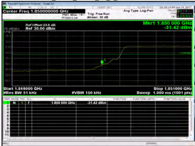
Band25_5MHz_QPSK_25_0_LowCH26065-1852.5
