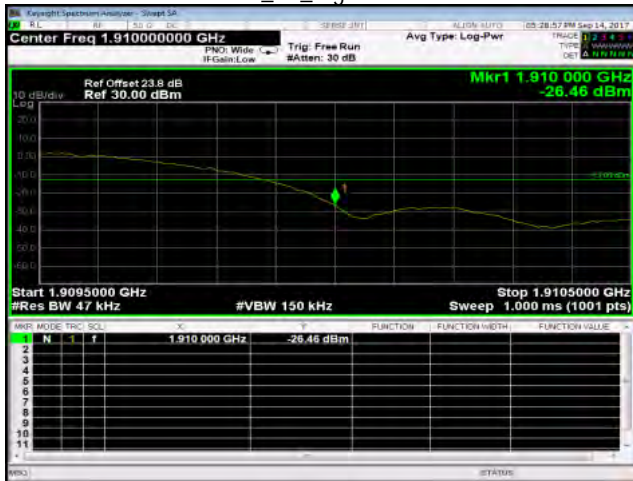
WCDMA_B2_HighCH9538-1907.6
