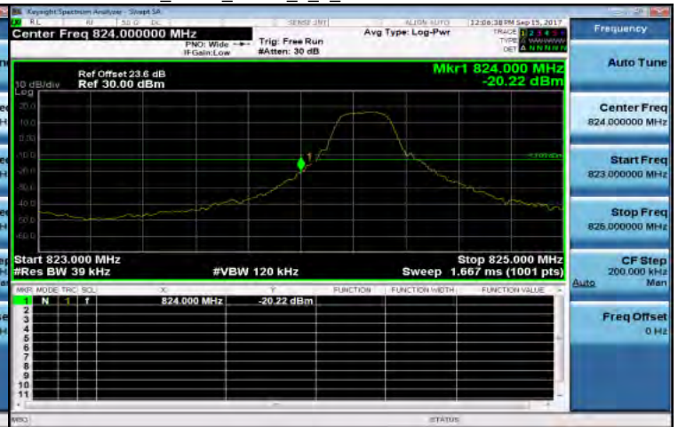
Band5_3MHz_QPSK_1_0_LowCH20415-825.5
