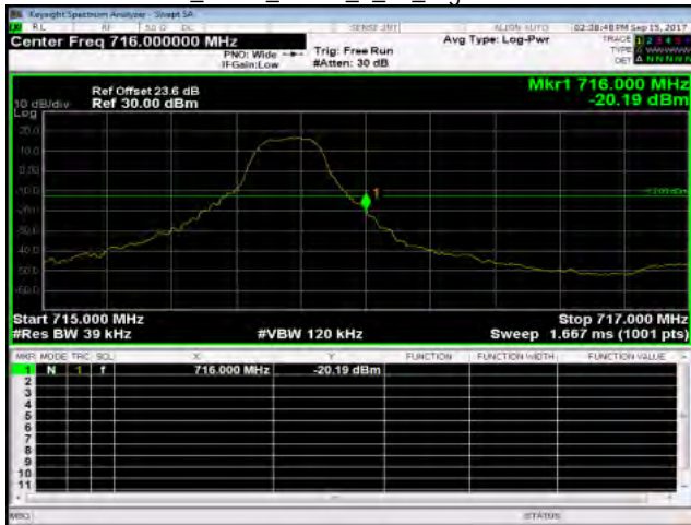
Band12_3MHz_QPSK_1_14_HighCH23165-714.5
