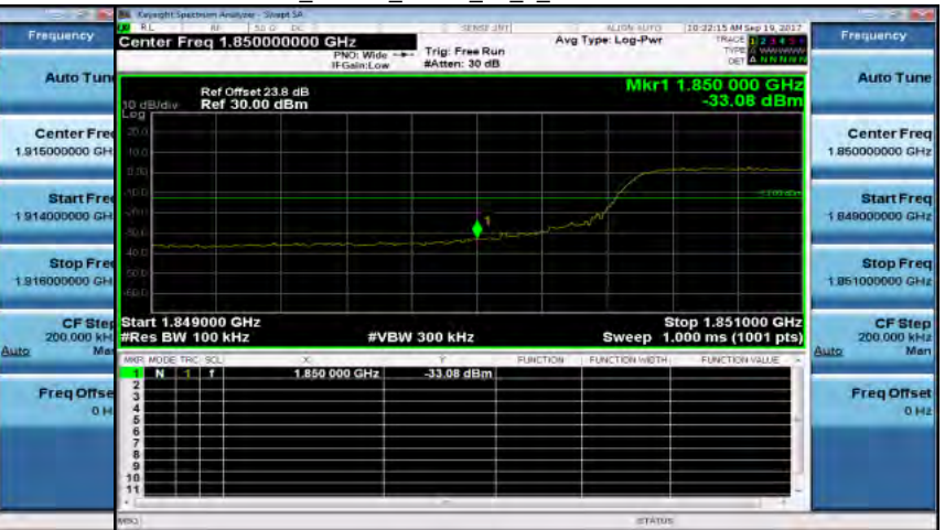
Band25_10MHz_QPSK_50_0_LowCH26090-1855
