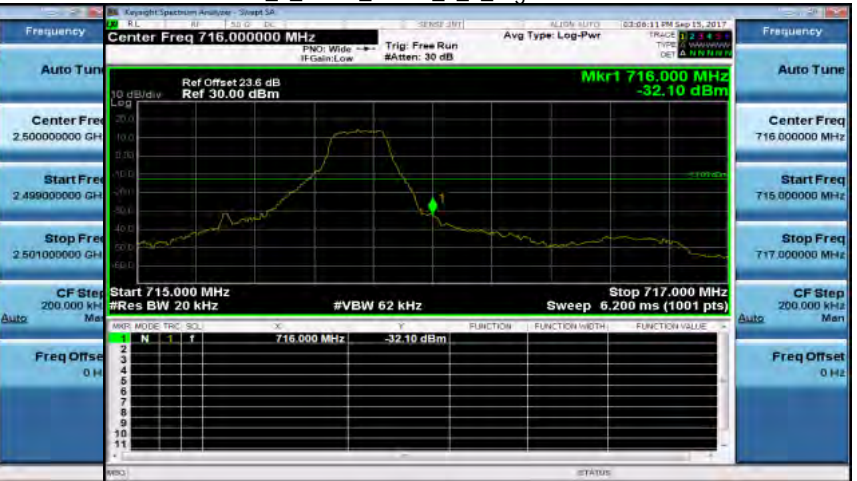
Band12_1_4MHz_QPSK_1_5_HighCH23173-715.3
