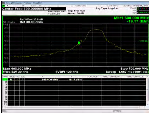
Band12_3MHz_QPSK_1_0_LowCH23025-700.5
