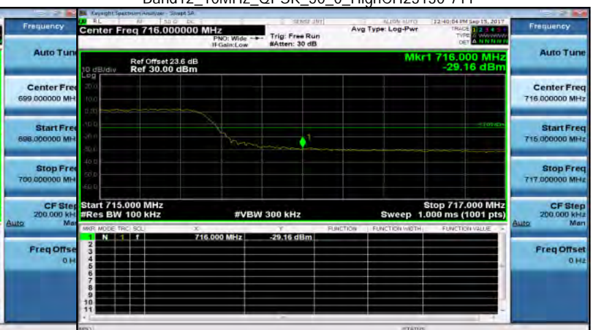
Band12_10MHz_QPSK_50_0_HighCH23130-711
