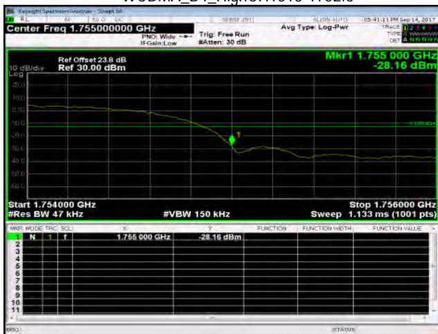
WCDMA_B4_HighCH1513-1752.6
