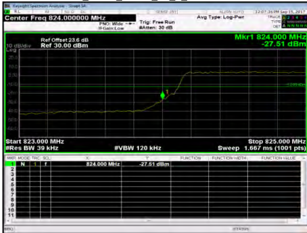
Band5_3MHz_QPSK_15_0_LowCH20415-825.5
