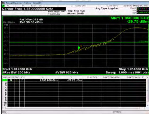
Band25_15MHz_QPSK_1_0_LowCH26115-1857.5
