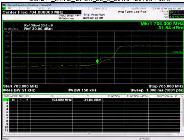
Band17_5MHz_QPSK_25_0_LowCH23755-706.5
