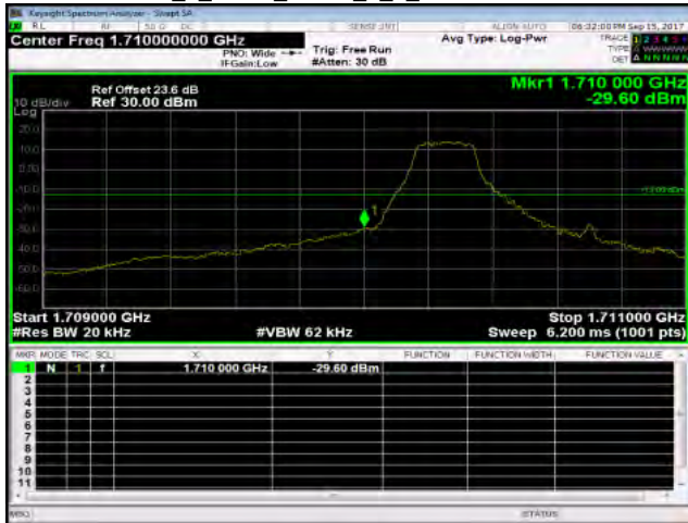
Band4_1_4MHz_QPSK_1_0_LowCH19957-1710.7
