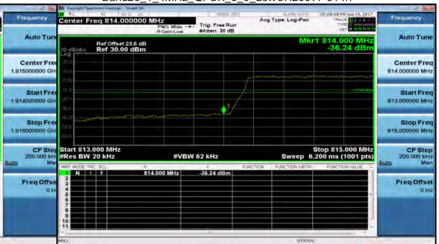
Band26_1_4MHz_QPSK_6_0_LowCH26697-814.7
