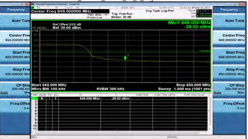
Band5_10MHz_QPSK_50_0_HighCH20600-844
