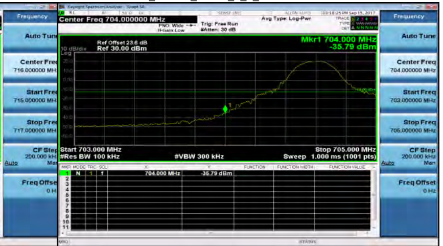
Band17_10MHz_QPSK_1_0_LowCH23780-709
