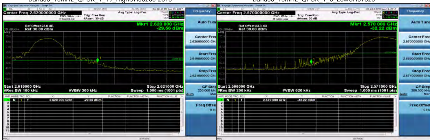
Band38_10MHz_QPSK_1_49_HighCH38200-2615
