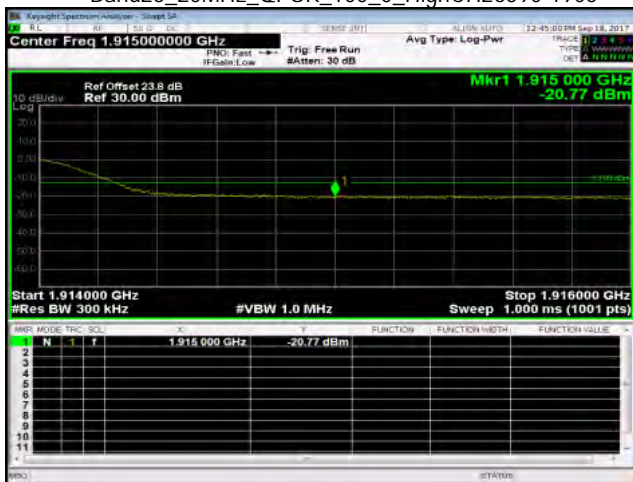
Band25_20MHz_QPSK_100_0_HighCH26590-1905
