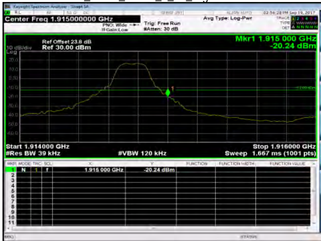
Band25_3MHz_QPSK_1_14_HighCH26675-1913.5
