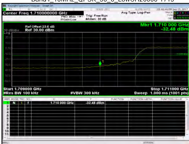
Band4_10MHz_QPSK_50_0_LowCH20000-1715
