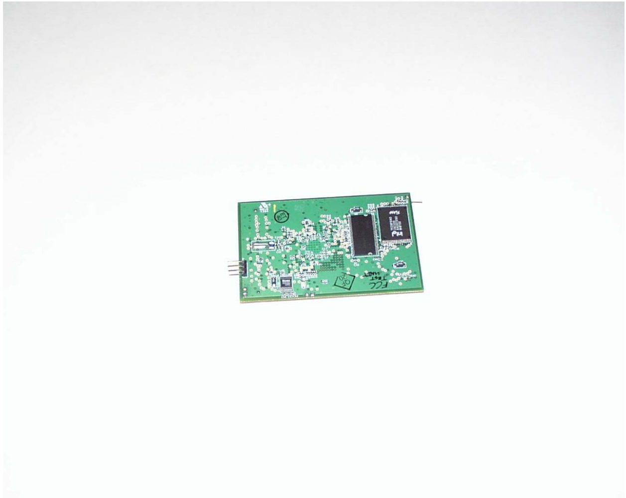
Photograph 7 - View of the Trace Side of the Daughter Card
