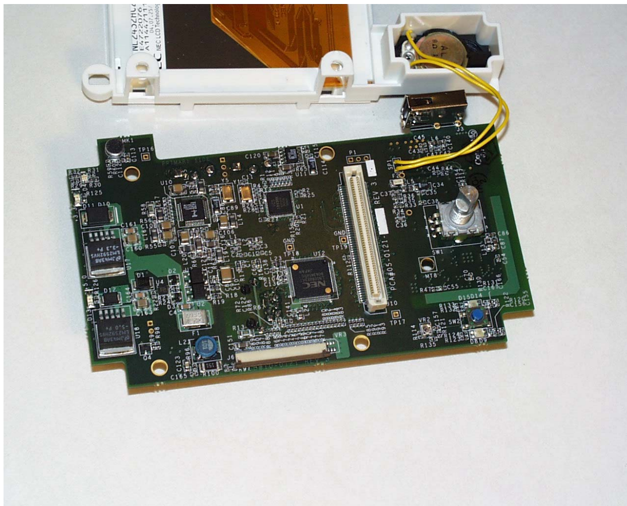
Photograph 5 - Top View of the Main Card
