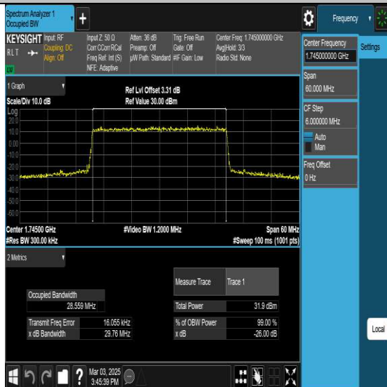
NTN-N66-PC3-15-30-M-DFT-QPSK-Outer_Full-Ant1-PASS
