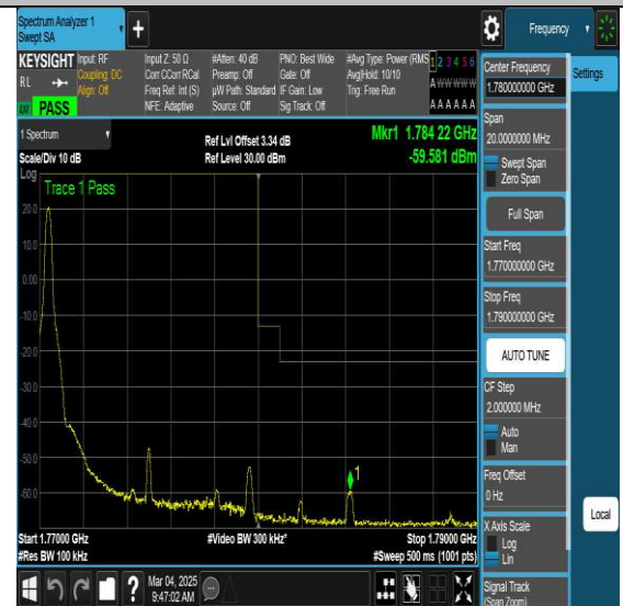
NTVN-N66-PC3-15-10-H-DFT-QPSK-Edge_1RB_Left-Ant1-PASS
