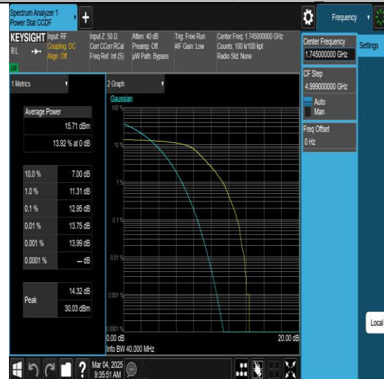
NTNV-N66-PC3-15-40-M-DFT-QPSK-Outer Full-PASS
