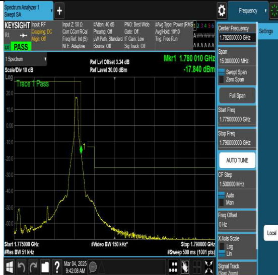
NTVN-N66-PC3-15-5-H-DFT-QPSK-Edge_1RB_Right-Ant1-PASS
