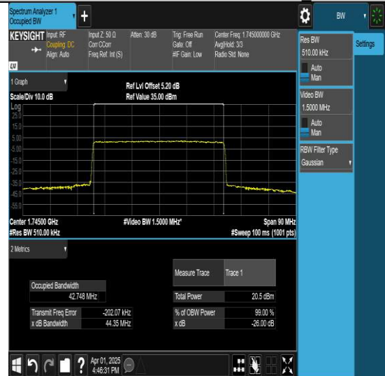
NTNV-N66-PC3-15-45-M-DFT-256QAM-Outer_Full-Ant1-PASS
