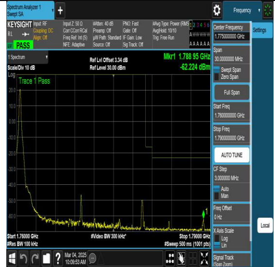
NTNV-N66-PC3-15-20-H-DFT-QPSK-Edge_1RB_Left-Ant1-PASS
