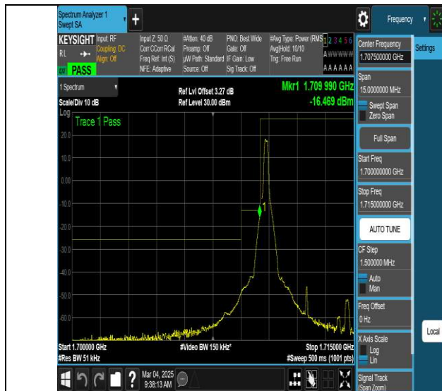
NTN-N66-PC3-15-5-L-DFT-QPSK-Edge_1RB_Left-Ant1-PASS
