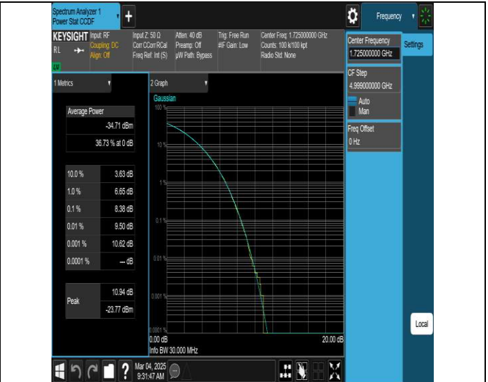
NTNV-N66-PC3-15-30-L-DFT-QPSK-Outer Full-PASS
