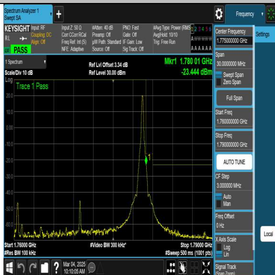
NTNV-N66-PC3-15-20-H-DFT-QPSK-Edge_1RB_Right-Ant1-PASS
