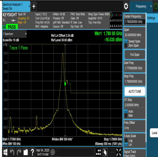
NTNV-N66-PC3-15-10-H-DFT-QPSK-Edge_1RB_Right-Ant1-PASS
