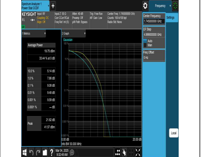
NTNV-N66-PC3-15-30-M-DFT-QPSK-Outer_Full-PASS
