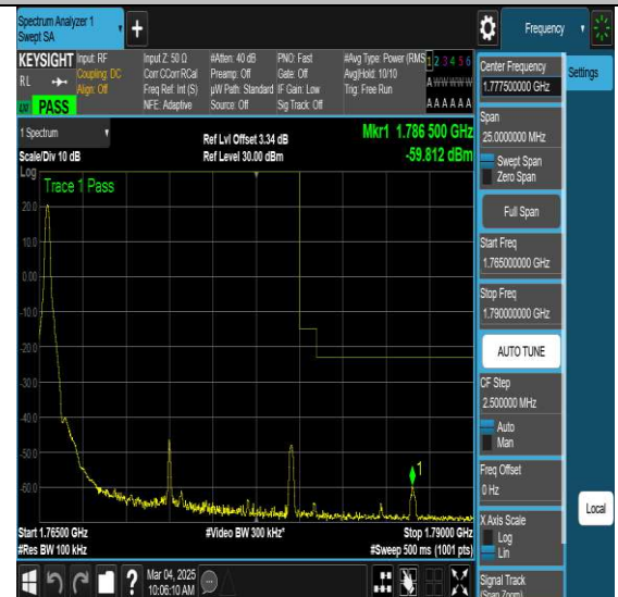
NTNV-N66-PC3-15-15-L-DFT-QPSK-Edge_1RB_Right-Ant1-PASS
