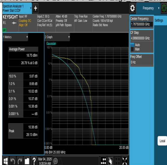
NTNV-N66-PC3-15-25-H-DFT-QPSK-Edge 1RB Left-PASS
