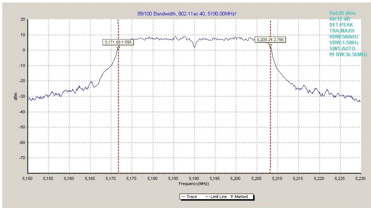
Fig.100 99% Occupied bandwidth (802.11ac-HT40, 5190MHz)
