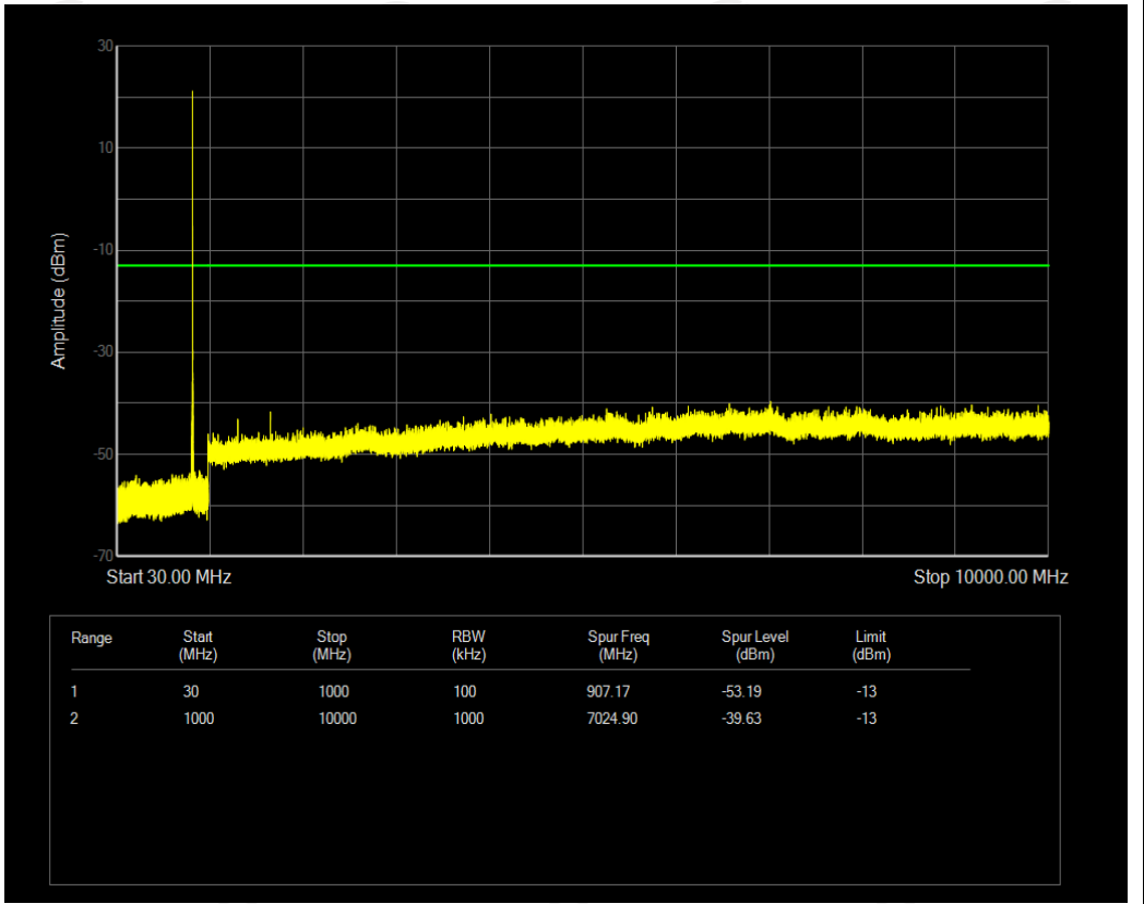
n26(824-849) SCS=15kHz DFT_BPSK BW=5MHz Channel=167300 RB=1@0
