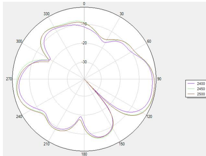
Phi 90 2D
