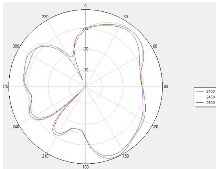
Theta 90 2D
