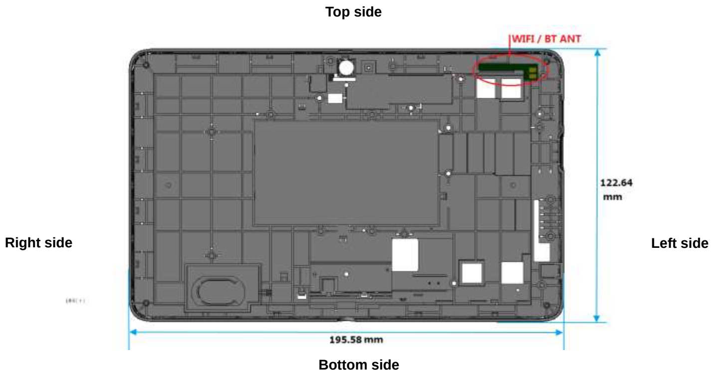
Picture 11.1 Antenna Locations (Back View)
