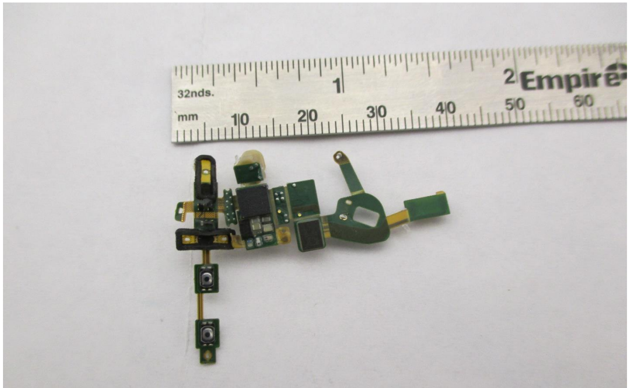
PCBA back
