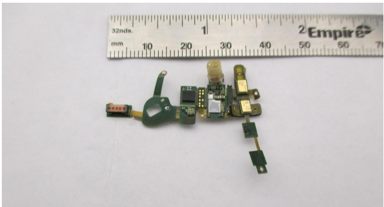
PCBA front
