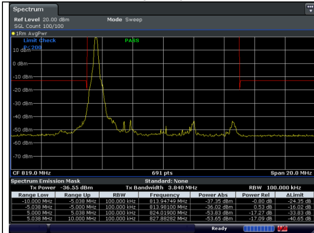
16QAM Middle Channel - 1 RB_Low
