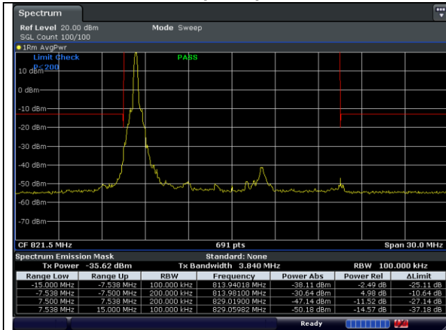
QPSK Middle Channel - 1 RB_Low
