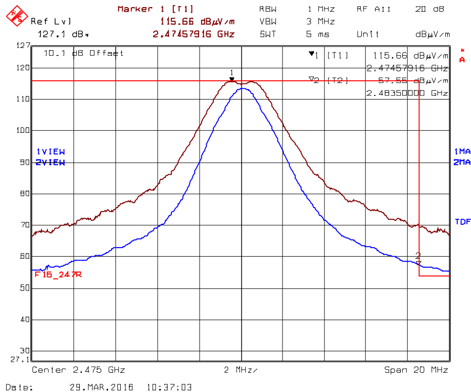
Plot 5.2.4.5.2.6. Band-Edge RF Radiated Emissions at 3 m, Vertical Polarization Higher End of Frequency Band, Ch25- 2475 MHz, QPSK Modulation, Power 8 Mode 1 @ 66% Duty Cycle
