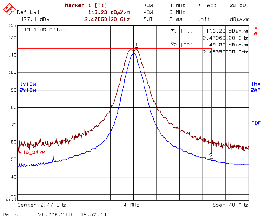
Plot 5.2.4.3.2.4. Band-Edge RF Radiated Emissions at 3 m, Vertical Polarization High End of Frequency Band, Ch24- 2470 MHz, QPSK Modulation, Power 8 Mode 1
