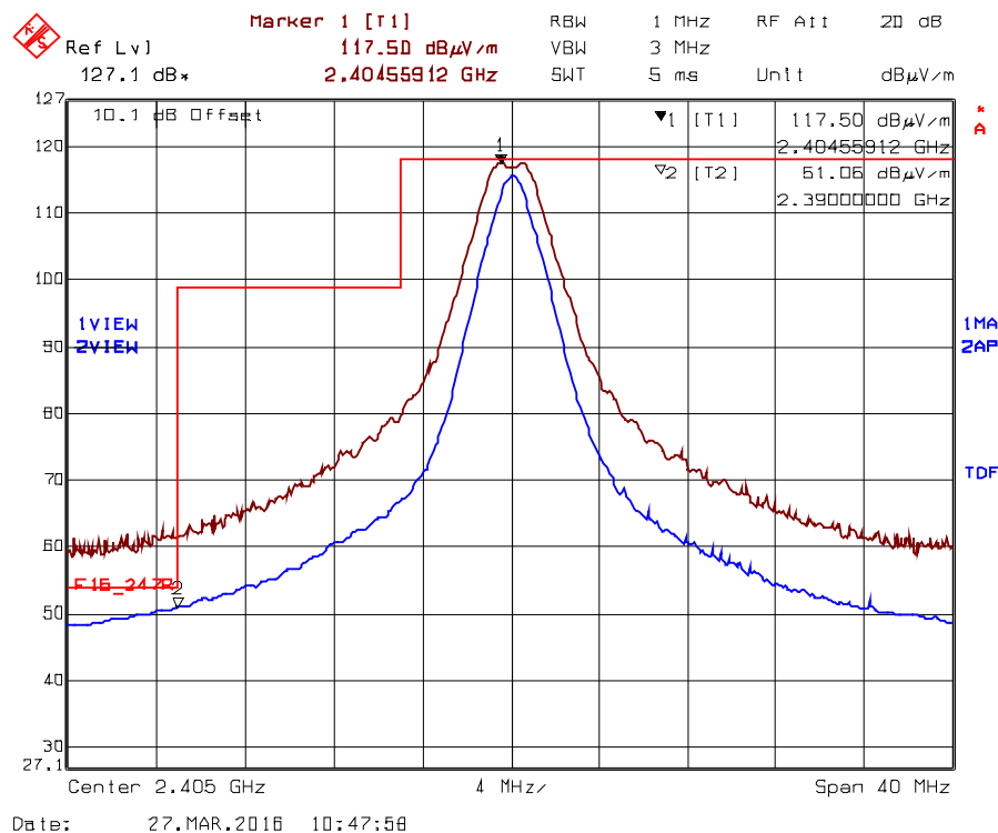
Plot 5.2.4.4.2.1. Band-Edge RF Radiated Emissions at 3 m, Horizontal Polarization Low End of Frequency Band, Ch11- 2405 MHz, QPSK Modulation, Power 8 Mode 1
