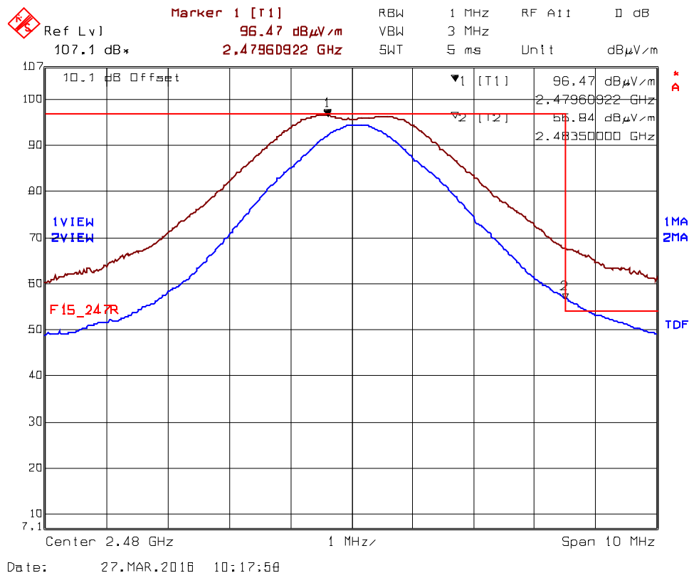
Plot 5.2.4.4.2.8. Band-Edge RF Radiated Emissions at 3 m, Vertical Polarization Highest End of Frequency Band, Ch26- 2480 MHz, QPSK Modulation, Power -5 Mode 1 @ 66% Duty Cycle
