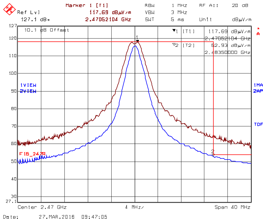
Plot 5.2.4.4.2.4. Band-Edge RF Radiated Emissions at 3 m, Vertical Polarization High End of Frequency Band, Ch24- 2470 MHz, QPSK Modulation, Power 8 Mode 1
