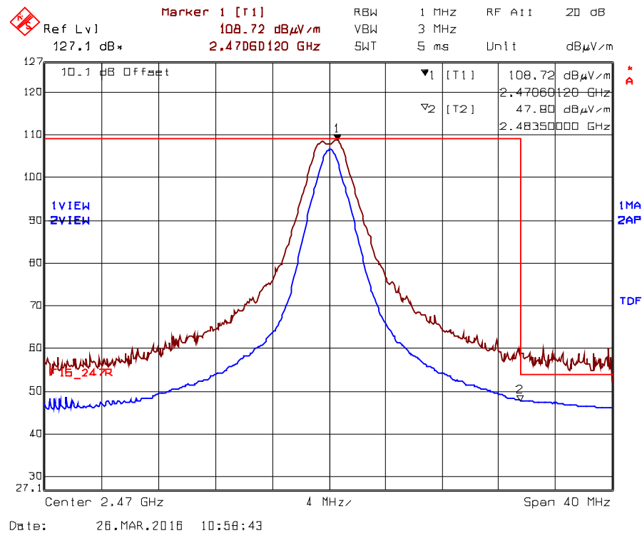
Plot 5.2.4.3.2.3. Band-Edge RF Radiated Emissions at 3 m, Horizontal Polarization High End of Frequency Band, Ch24- 2470 MHz, QPSK Modulation, Power 8 Mode 1
