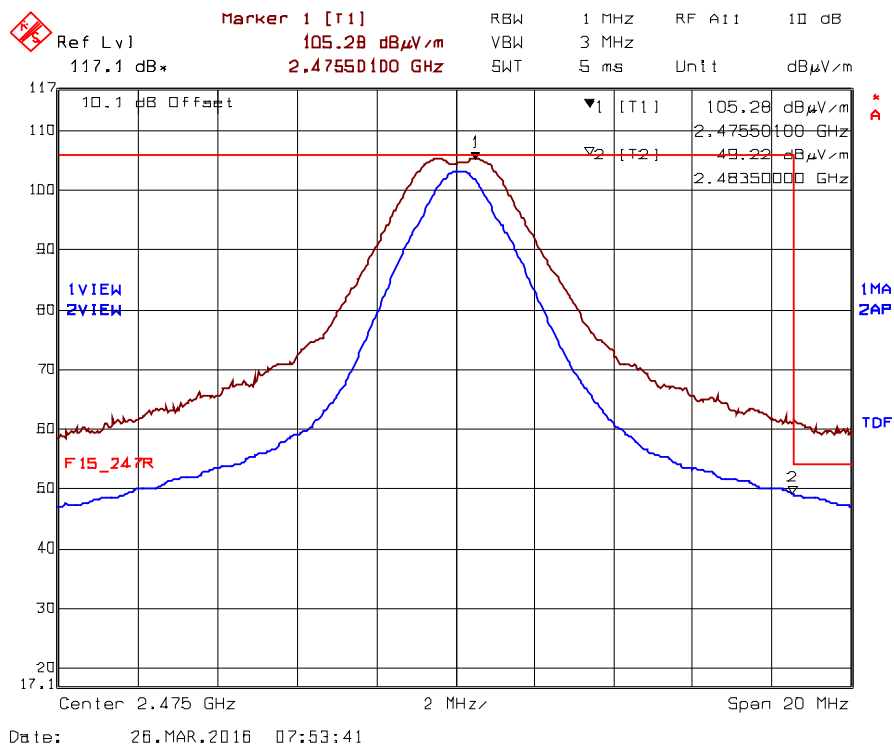
Plot 5.2.4.1.2.3. Band-Edge RF Radiated Emissions at 3 m, Horizontal Polarization High End of Frequency Band, Ch25- 2475 MHz, QPSK Modulation, Power 8 Mode 1
