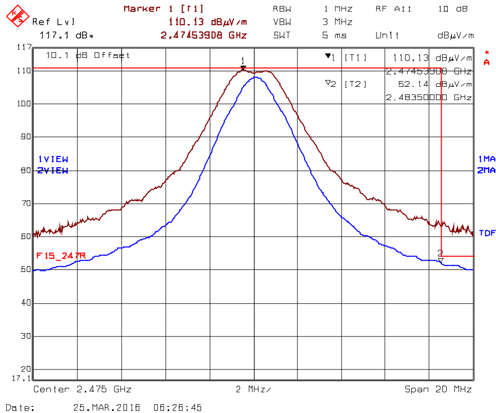
Plot 5.2.4.2.2.4. Band-Edge RF Radiated Emissions at 3 m, Vertical Polarization High End of Frequency Band, Ch25- 2475 MHz, QPSK Modulation, Power 8 Mode 1
