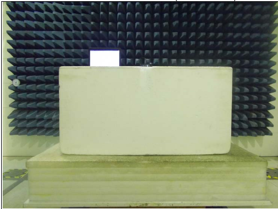
Radiated Emission Test above 1GHz (BT EDR / BT LE)
