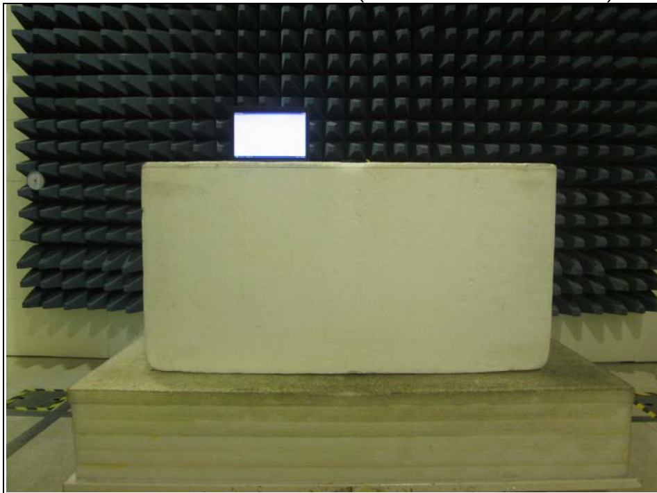
Radiated Emission Test above 1GHz (WLAN 2.4GHz / WLAN 5GHz)
