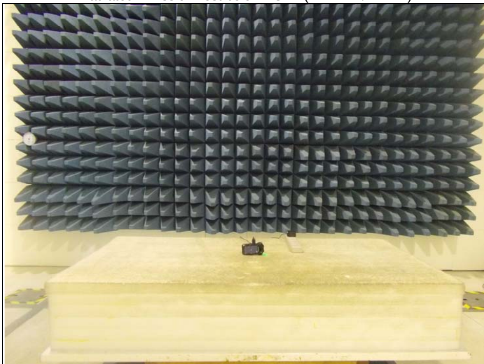
Radiated Emission Test below 1GHz (BT EDR / BT LE)
