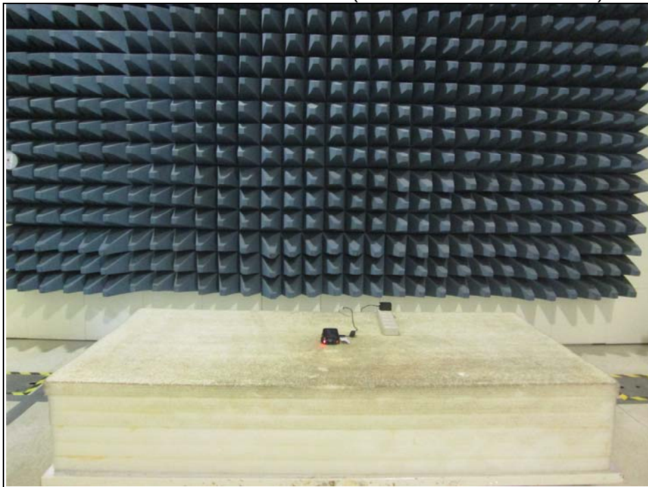
Radiated Emission Test below 1GHz (WLAN 2.4GHz / WLAN 5GHz)
